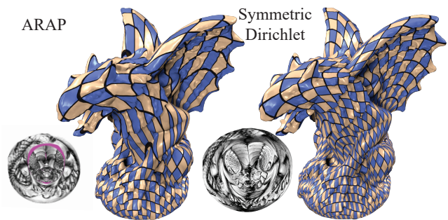
Figure 3: The ARAP energy (left) introduces 6K inverted triangles in the parametrization (highlighted in magenta) which result in highly distorted regions around the neck and the wing of the Gargoyle. Our algorithm avoids the problem by minimizing a flip preventing symmetric Dirichlet energy (right). This model has 99K faces and took 20 iterations and 3 seconds to optimize.
