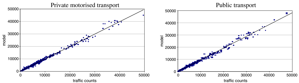
Fig. 7. Comparison of traffic counts and final adjusted matrices.
