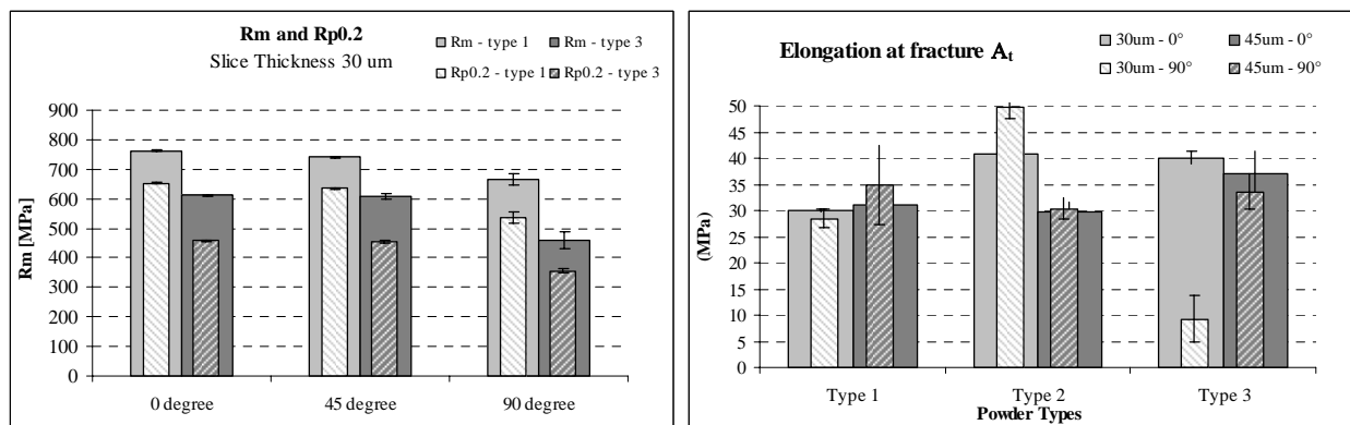
Figure 6: Ultimate tensile strength R_m and yield strength at 0.2% offset R_{p0.2} for 0°, 45° and 90° orientations (left) and elongation at fracture A_t (right) for powder type 1 and 3.
