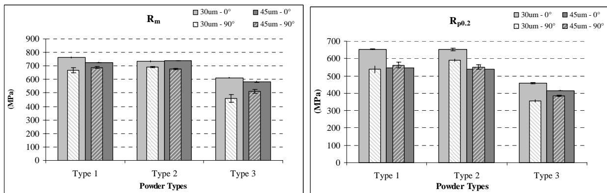
Figure 5: Ultimate tensile strength R_m and yield strength at 0.2% offset R_{p0.2} for powder types 1, 2 and 3 for 30 \mu m- and 45 \mu m-layers and for the two specimen orientations 0° and 90°
