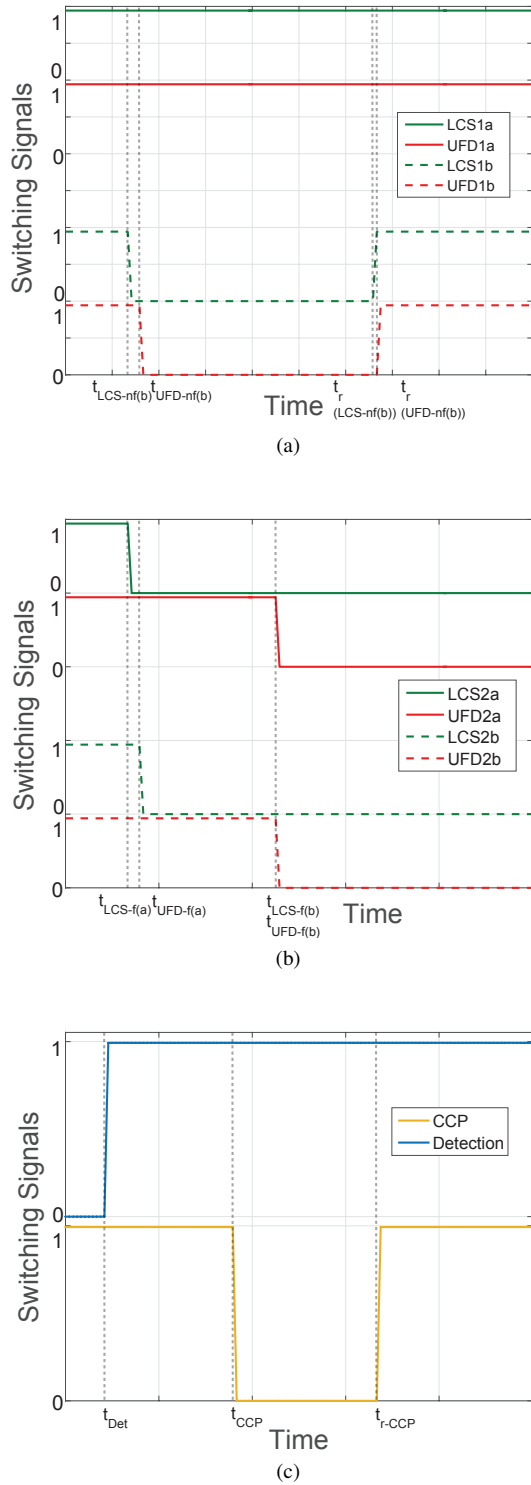
Fig. 6. Pole-to-ground - Switching Sequence MLB1: (a) Healthy line path (1); (b) Faulty line path (2); (c) Main Breaker path and Fault signals. '1' and '0' values indicate the 'on' and 'off' states respectively.
