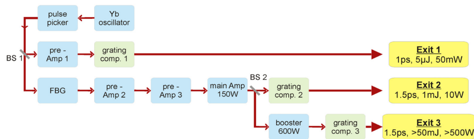
Fig. 1. Schematic diagram of the Yb-InnoSlab platform providing three different exit ports at different power levels, all derived from the same oscillator pulse to minimize temporal jitter. The total optical path between exit 1 to exit 3 is only about 16m. BS: beam splitter, FBG: fiber Bragg grating, comp: compressor, Amp: amplifier.
