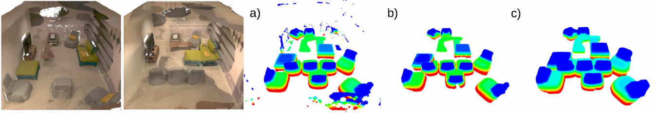
Fig. 3: Filtering of label grid \mathcal{D} : Example of the first coarse change detection step applied to two reconstructions ( left ). a ) - c ) show the state of the label grid \mathcal{D} . For better visibility \mathcal{D} is colored by height. a ) Voxel labels that are obtained by applying a threshold \theta to the raw TSDF difference of the two reconstructions ( left ). b ) The labels are filtered using an erosion kernel to reduce false positives caused by sensor and systematic noise in the reconstructions. c ) A dilation kernel is applied to recover the original geometry.
