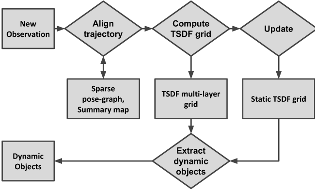
Fig. 2: Change Detection Algorithm Overview
