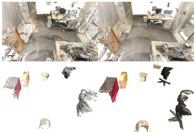
Fig. 4: Comparison of our approach ( right ) to the meta-room [9] algorithm ( left ). Static scene after processing all 4 observations ( top ). Our approach exhibits a cleaner and more complete segmentation and a better completion of the scene geometry that was occluded by objects. Our extracted objects ( bottom right ) are more complete and some of the smaller changes are missing with the meta-room based algorithm ( bottom left ). See table II for details.
