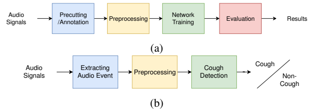
Fig. 3: (a) Machine learning pipeline: Describes the learning of a model from audio signals. (b) Cough detection pipeline: Describes the inference of cough from audio recordings.
