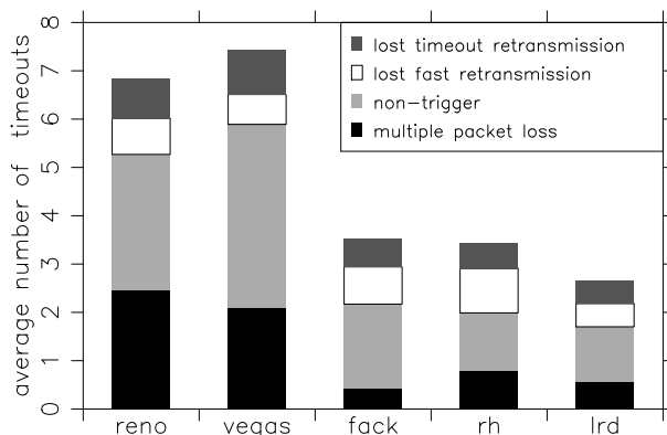
Figure 8: Breakdown of timeout causes for each protocol.
