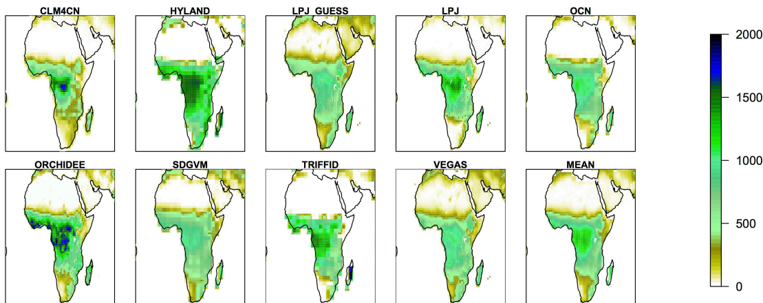
Fig. 4. Average Net Primary Productivity (NPP) for each DGVM and model mean over the period 1990–2009, units, \text{kg C m}^{-2} \text{yr}^{-1} .
