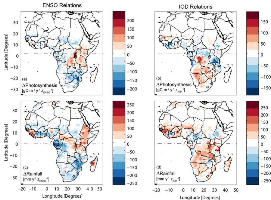
Fig. 7. Spatial distribution across Africa of the slope of least-squares linear regressions of SiB3 modeled (a, b) annual net photosynthesis ( P_{\text{net}} ) or CRU/TRMM (c, d) annual rainfall on climate indices. Each column corresponds to analyses with a particular index with the left column (a, c) for the multivariate ENSO index, and the right column (b, d) for the Indian Ocean Dipole Mode Index (IOD). Results are based on Williams et al. (2008).
