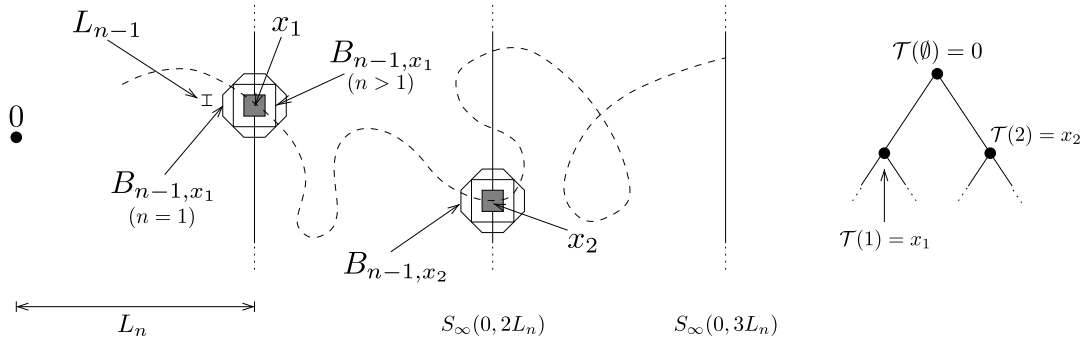
Figure 1: Any nearest-neighbor path in E_\varphi^{\geq h} (represented by the dashed line) connecting B_\infty(0, L_n) to S_\infty(0, 3L_n) , for some n \geq 1 , must cross a box B_{n-1, x_1} , for some x_1 \in S_\infty(0, L_n) \cap \mathbb{L}_{n-1} , as well as B_{n-1, x_2} , for some x_2 \in S_\infty(0, 2L_n) \cap \mathbb{L}_{n-1} , thus giving rise to the simultaneous occurrence of A_{n-1, x_1}^h and A_{n-1, x_2}^h .
