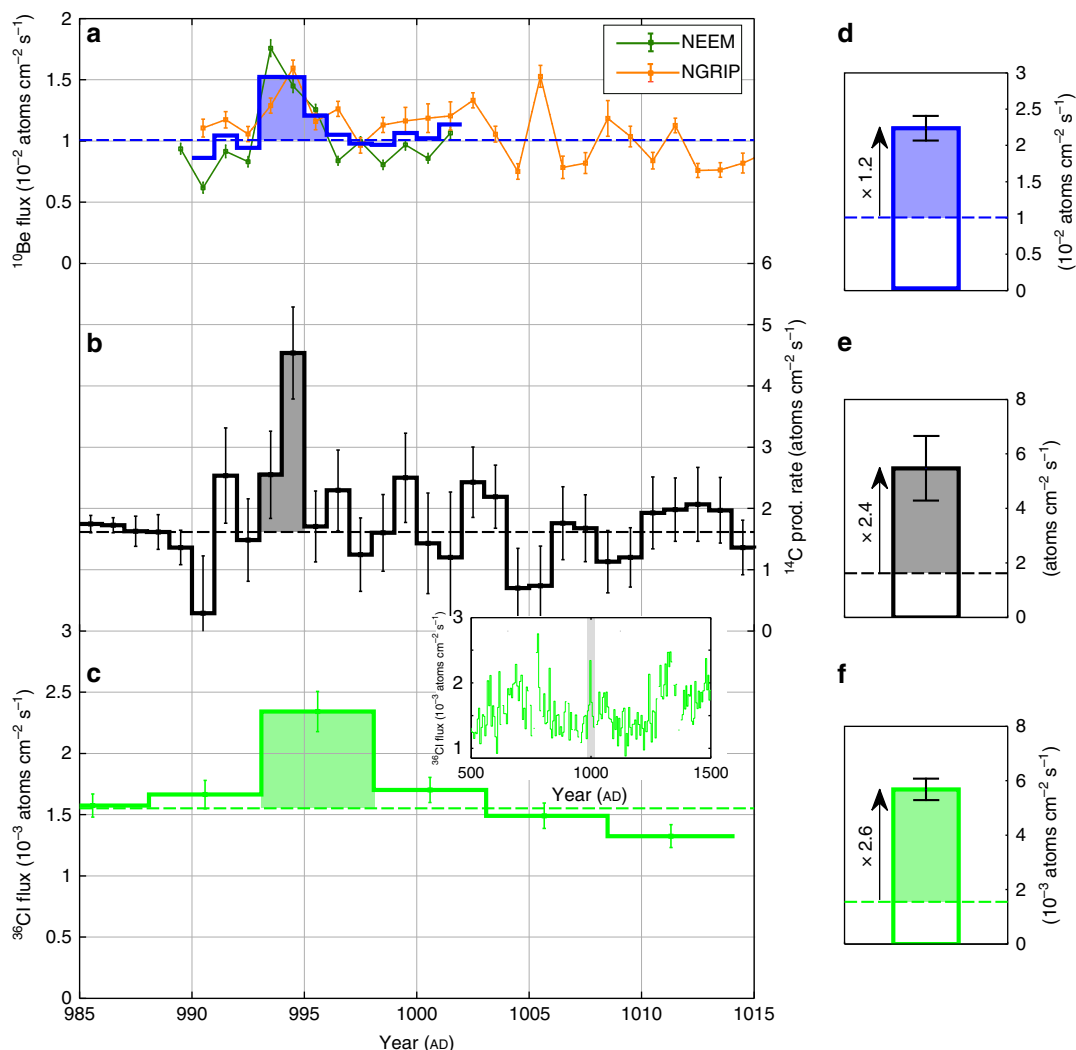
Figure 3 | The AD 993/4 event in view of ^{10}\text{Be} , ^{14}\text{C} and ^{36}\text{Cl} . Time series for AD 985–1015 (a) of ^{10}\text{Be} flux from the NEEP-2011-S1 and NGRIP ice cores in addition to the inferred average ^{10}\text{Be} flux (thick blue curve), (b) of modelled ^{14}\text{C} production rate based on previously published measurements 13 and (c) of ^{36}\text{Cl} flux 21 in addition to an inset with a longer series spanning AD 500–1500 for ^{36}\text{Cl} where the grey rectangle represents the time slice investigated. The dashed lines represent the natural background level which is set as the average value prior to and following the filled areas. The filled areas represent the estimated production enhancement caused by the cosmic-ray event of AD 993/4. The ^{10}\text{Be} and ^{36}\text{Cl} series have been corrected for a temporal offset between ice-core and tree-ring chronologies (Methods). The right panel shows radionuclide production enhancements caused by the AD 993/4 event in atoms \text{cm}^{-2} \text{s}^{-1} for 1 year for (d) ^{10}\text{Be} , (e) ^{14}\text{C} and (f) ^{36}\text{Cl} . The radionuclide increases are illustrated with arrows corresponding to the ratio between the inferred flux/production enhancements stacked over 1 year (coloured rectangles) and the estimated background levels (white rectangles). Uncertainties are based on error propagation including measurement errors and background variability of 1\sigma .
