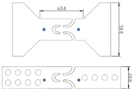
Figure 2. Specimens used for the experiments at low and intermediate strain rates (on the top), and high strain rates (on the bottom). Blue solid dots highlight the position of the virtual extensometer for relative displacement and speed measurements.
