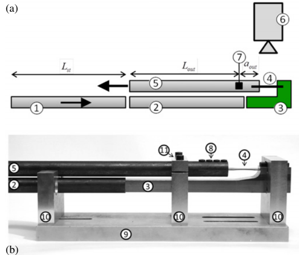
Figure 3. (a) Illustration of the experimental setup (b) Photograph of the Load Inversion Device – ① striker bar, ② input bar, ③ pusher of the LID, ④ specimen, ⑤ output bar, ⑥ high speed camera, ⑦ position of strain gauge, ⑧ grip section with slit, ⑨ base plate, ⑩ bearings, ⑪ removable clamp.
