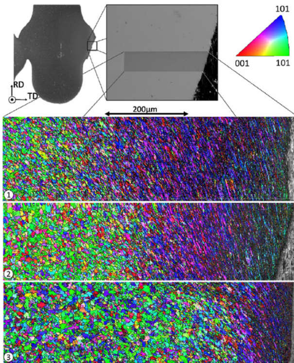
Figure 6. IPF-Y plots of the ① slow, ② intermediate and ③ fast experiments with added grain boundaries. Colors represent the grain orientation normal to the sample surface as defined by the stereographic triangle inset in the top right corner of the image.
