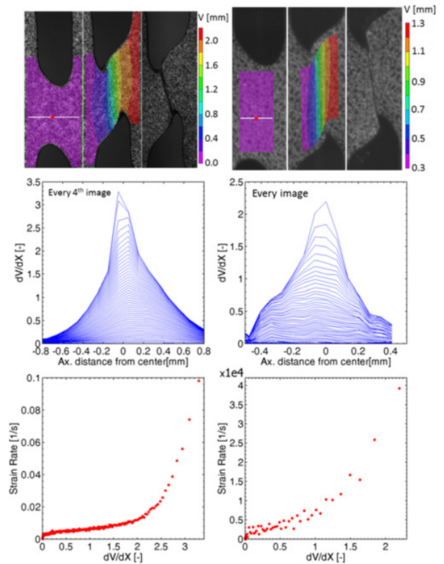
Figure 5. Displacement field and the extracted evolution of the strain along the white line and the strain rate at the location of the red dot (slow case left column, fast case right column).
