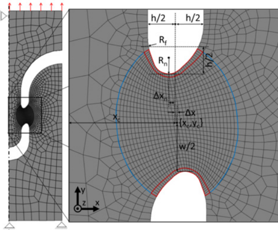
Figure 1. Finite element model of the optimized shear specimen geometry, including the parameterized variables.
