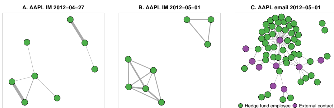
Figure 5.3: Examples of communication networks relevant for the trading of Apple stock on selected business days. While the instant messaging subgraph on April 27, 2012 (panel A) exhibits low clustering and balance, the opposite is true a couple of days later (panel B). The email subgraph on May 1st, 2012 (panel C) shows the communication between hedge fund employees (green) and external contacts at investment banks (purple).
