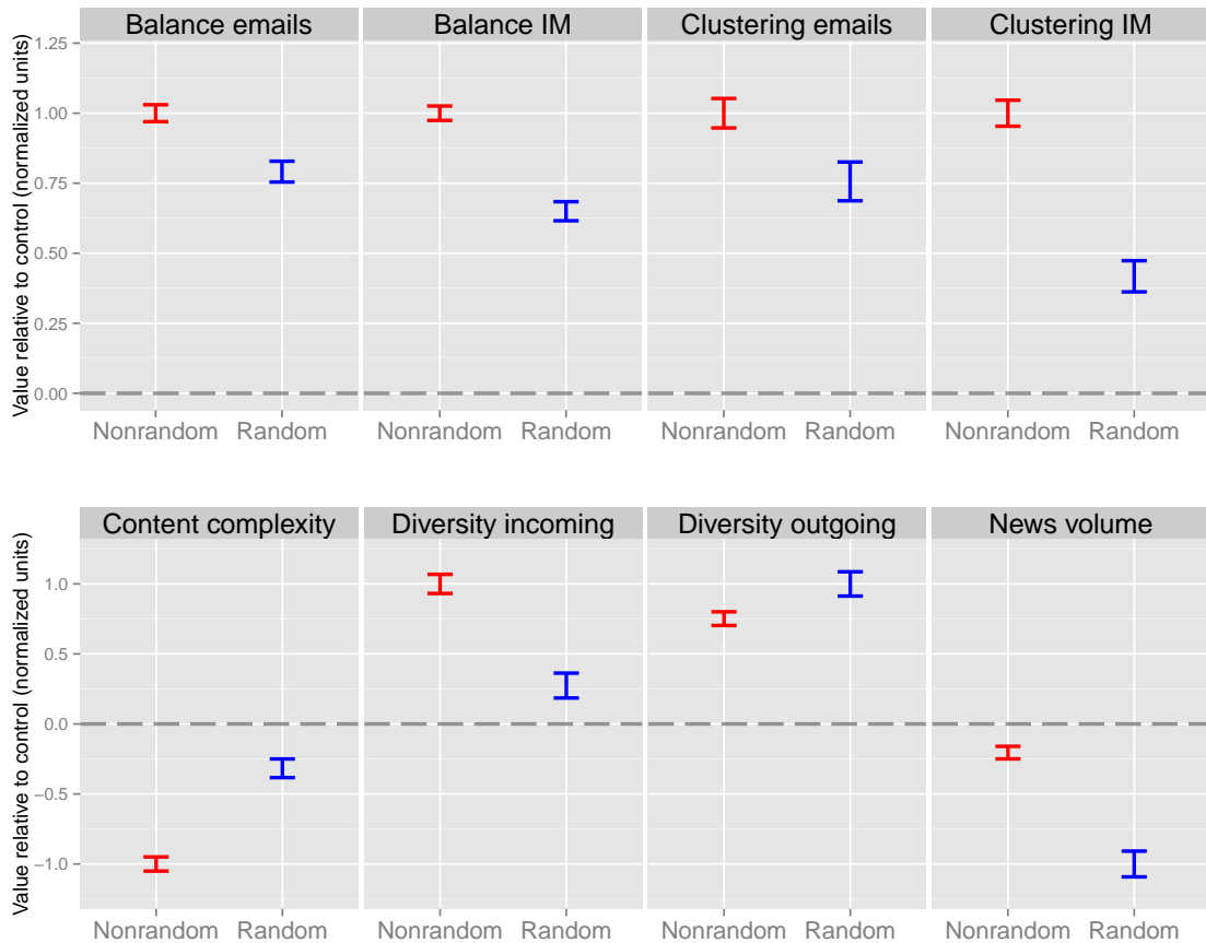
Figure 5.4: Contextual variables associated with random trading by humans relative to non-trading (control). (A) Especially after the Global Financial Crisis random trading is associated with less clustered and less balanced email and instant messaging (IM) internal communication networks. (B) A stock is more likely to be traded randomly when there is less business news reported, when the incoming information is less diverse and when there is more sector-specific complexity in the market. By contrast, a more diverse outgoing communication pattern does not lead to a reduced likelihood of random trading.
