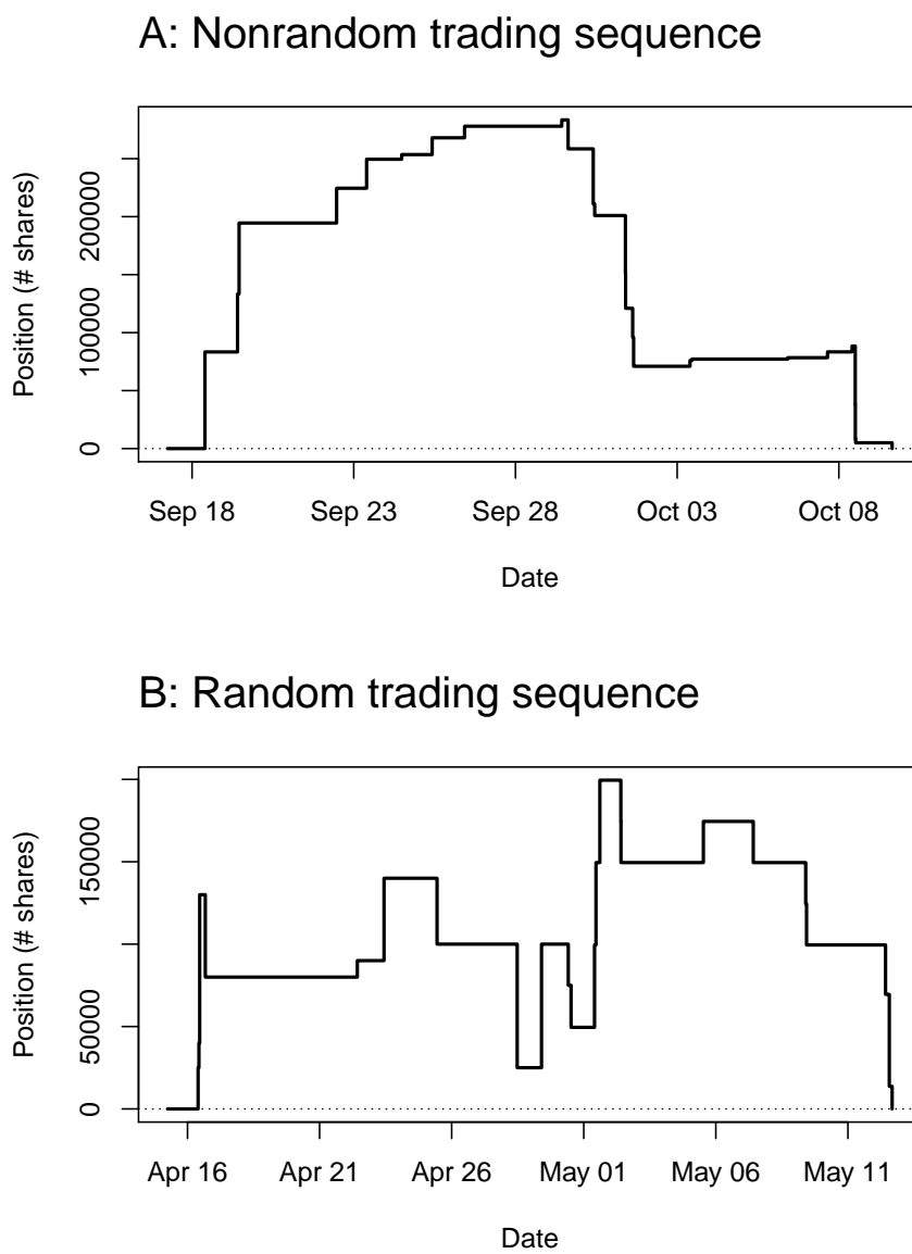
Figure 5.1: Illustrative examples for trading sequences classified as nonrandom (A) and random (B).
