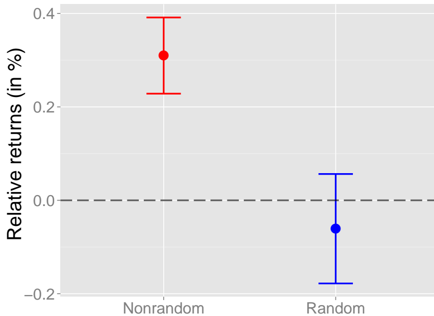
Figure 5.2: Profitability of trade sequences vs stochasticity. While the returns of nonrandom trading are significantly positive, random trading does not make money on average.
