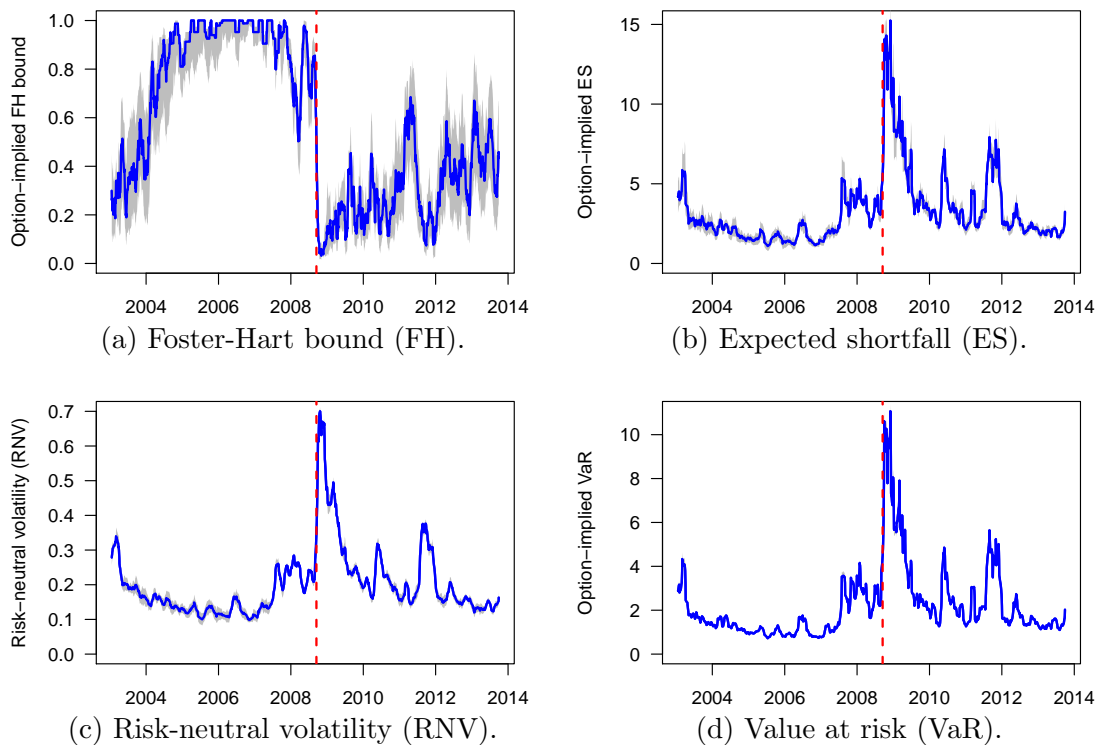
Figure 4.1: Option-implied measures of riskiness.
