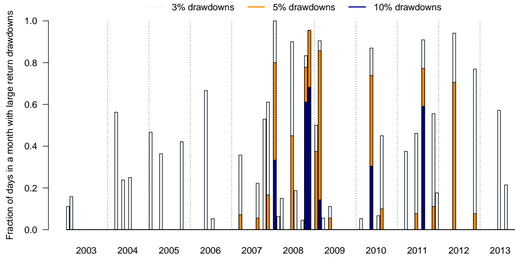
Figure 4.2: Distribution of S&P 500 downturns over time.
