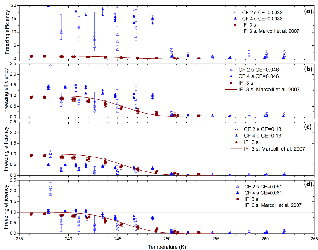
Figure 5. Freezing efficiency for 800 nm ATD particles with a concentration of 1000\text{ cm}^{-3} calculated with four different assumptions for CE: panel (a), with theoretical CE from Wang et al. (1978) and Park et al. (2005); panel (b), with 14\times CE from panel (a) (see text for details); panel (c), with CE = 0.13 (applying the value for 200 nm AgI particles for all particle sizes); panel (d), with CE = 0.061, which shifts collision efficiencies close to 1. Filled triangles show contact freezing for 4 s residence time in the CLINCH chamber; the open triangles are for 2 s residence time. Each triangle represents an independent measurement. Error bars represent the precision of the IODE detector. Brown circles show the freezing efficiency for immersion freezing of droplets in the IMCA–ZINC chamber for a 3 s residence time. The brown lines show the FF calculated with the active site immersion freezing parameterization from Marcolli et al. (2007) evaluated for 800 nm particles and a 3 s residence time. The gray horizontal line indicates FE = 1. Note that the y scale in panel (a) is different from the ones in panels (b), (c) and (d).
