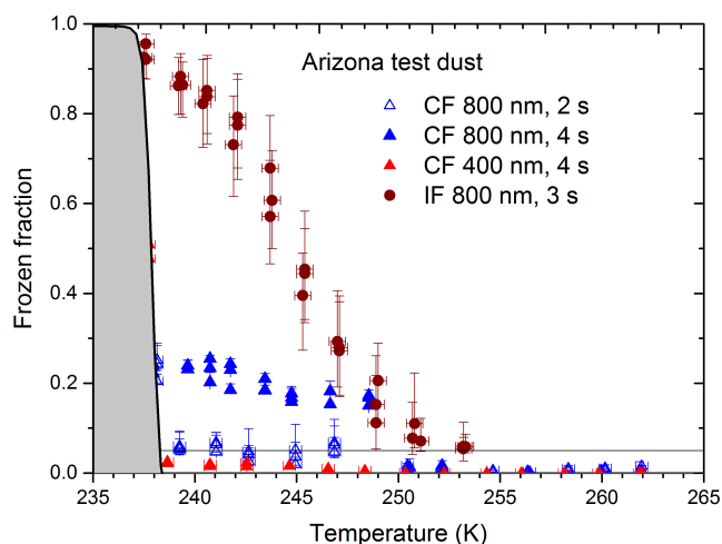
Figure 2. Frozen fraction against chamber temperature for ATD particles of 400 nm and 800 nm diameter. Contact freezing (CF) for aerosol concentrations of 1000\text{ cm}^{-3} is given by triangles for droplet residence times of 2 and 4 s. Immersion freezing (IF from IMCA–ZINC) for 800 nm ATD particles and a 3 s residence time in ZINC is shown by circles. The gray shaded area shows the homogeneous freezing of droplets determined from blank experiments (without aerosol), and the black horizontal line indicates the lower reliability limit of the measurements determined from the blank signal level observed in experiments without aerosol. Error bars represent the uncertainty in the frozen fraction due to the classification (liquid or ice) uncertainty of the IODE detector (Lüönd et al., 2010).
