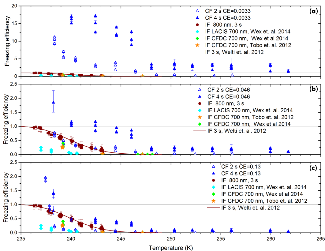
Figure 6. Freezing efficiency for 800 nm kaolinite particles with a concentration of 1000\text{ cm}^{-3} calculated with 3 different assumptions for CE: panel (a), with the theoretical CE from Park et al. (2005) and Wang et al. (1978); panel (b), with 14\times CE from panel (a); panel (c), with CE = 0.13 (applying the value of 200 nm AgI particles) for lower bound of freezing efficiency. Each triangle represents an independent measurement. Error bars represent the precision of the IODE detector. Brown circles show the freezing efficiency of droplets in ZINC for a residence time of 3 s for 800 nm kaolinite particles. Orange stars show immersion freezing of droplets activated by 700 nm Fluka kaolinite particles (from Fig. 2a of Tobo et al., 2012). Light blue diamonds show immersion freezing of droplets activated by a 700 nm Fluka kaolinite particle (LACIS data with 1.6 s residence time (from Fig. 2 (right panel) of Wex et al., 2014)). The green diamond shows immersion freezing of droplets activated by 700 nm kaolinite particles (CFDC data with 5 s residence time (from Fig. 2 (right panel) of Wex et al., 2014)). The brown line represents the \alpha -pdf parameterization from Welts et al. (2012). The gray horizontal line indicates the maximum freezing efficiency. Note that the y scale for panel (a) is different from the ones in panels (b) and (c).
