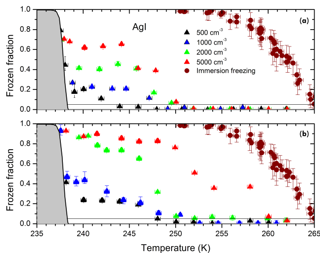
Figure 1. Frozen fraction against chamber temperature for silver iodide particles of 200\text{ nm} diameter. Contact freezing for aerosol concentrations from 500 to 5000\text{ cm}^{-3} is given by triangles for a droplet residence time of 2\text{ s} in panel (a) and 4\text{ s} in panel (b). Immersion freezing for a 3\text{ s} residence time of droplets in the ZINC chamber is shown by circles. The gray shaded area shows the homogeneous freezing of droplets determined from blank experiments (without aerosol) and the black horizontal line indicates the lower reliability limit of the measurements determined from the blank signal level observed in experiments without aerosol. Error bars represent the uncertainty in the frozen fraction due to the classification (liquid or ice) uncertainty of the IODE detector (Lüönd et al., 2010).
