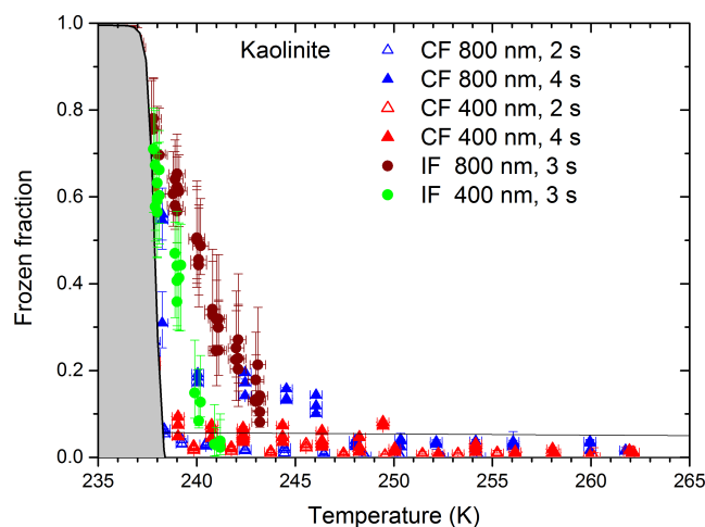
Figure 3. Frozen fraction against chamber temperature for kaolinite particles of 400 and 800 nm diameter. Contact freezing (CF) for aerosol concentrations of 1000\text{ cm}^{-3} is given by triangles for droplet residence times of 2 and 4 s. Immersion freezing (IF from IMCA–ZINC) for 400 and 800 nm kaolinite particles and a 3 s residence time in ZINC is shown by green and brown circles, respectively. The gray shaded area shows the homogeneous freezing of droplets determined from blank experiments (without aerosol), and the black horizontal line indicates the lower reliability limit of the measurements determined from the blank signal level observed in experiments without aerosol. Error bars represent the uncertainty in the frozen fraction due to the classification (liquid or ice) uncertainty of the IODE detector (Lüönd et al., 2010).
