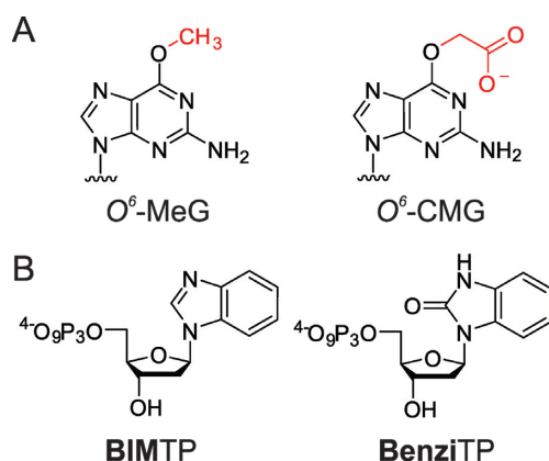
Figure 1. (A) Chemical structure of O 6 -alkylguanine adducts studied herein. (B) Artificial nucleotides BIMTP and BenziTP investigated as probes for DNA adducts.
