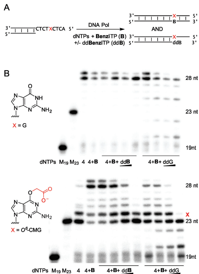
Figure 5. (A) Primer extension experiment with ddBenziTP marking the position of O 6 -CMG adduct in DNA by KTqM747K DNA polymerase. (B) PAGE analysis of reactions with DNA containing X = G or X = O 6 -CMG at 24 nt using increasing concentrations of ddBenziTP (0, 100, 500, 1000 and 2000 μM) added to 10 μM of all four natural dNTPs and 10 μM BenziTP . M 19 , primer 19 nt; M 23 , 23 nt marker; 4, all four dNTPs; 4+B, all four dNTPs plus BenziTP ; 4+B+ddB, all four dNTPs, BenziTP , plus ddBenziTP ; 4+B+ddG, all four dNTPs, BenziTP , plus ddGTP .
