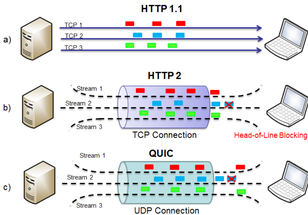
Figure 2. Multiplexing Comparison
