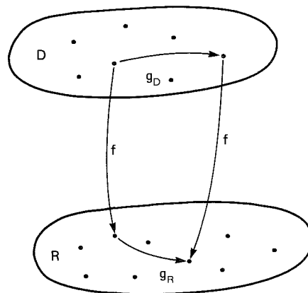
Figur 1-7 Homomorphismus
