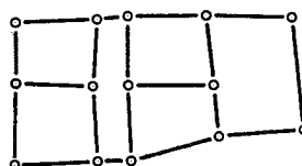
Figur 7-2 Partition
