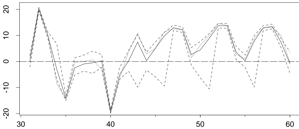
Figure 7: Behavior of Monte Carlo filter (kernel method) for t = 31, \dots, 60 : State variable (dotted line), 50%-quantiles of Monte Carlo filter (solid line) and 10%-, 90%-quantiles of Monte Carlo filter (dashed lines).
