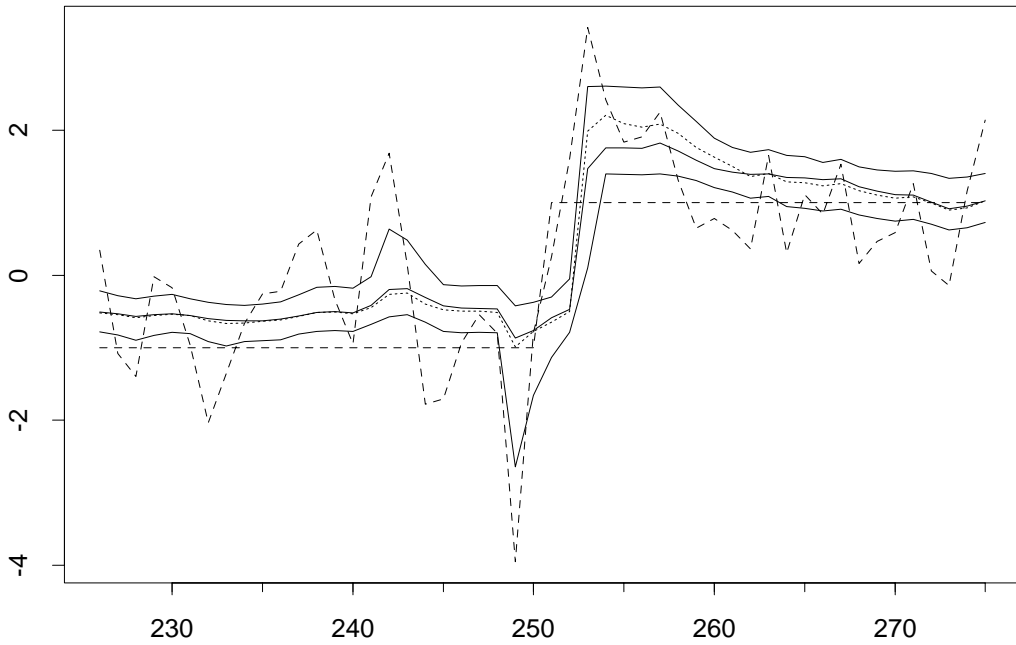
Figure 2: Behavior of Monte Carlo filter (direct method) near the jump at t = 250 : Observations and state variable (dashed lines), 10%-, 50%- and 90%-quantiles of Monte Carlo filter (solid lines) and 50%-quantiles of filter with numerical integration (dotted line).
