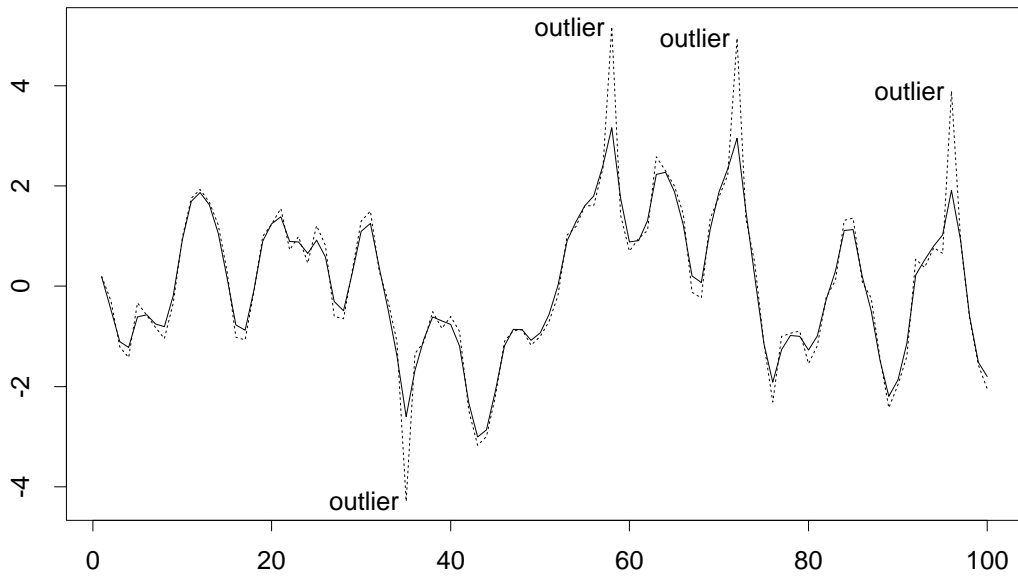
Figure 11: AR(2) with outliers: Mean of the direct smoother (solid line) for sample size N=1000 and the observations y_t (dotted line). The four outliers are indicated.
