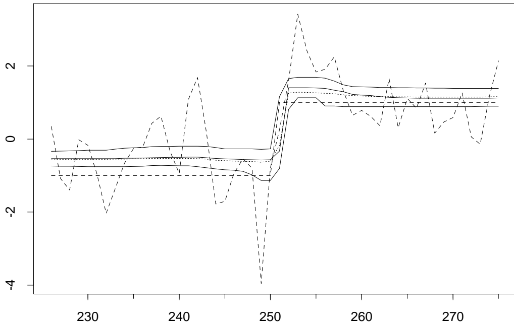
Figure 3: Behavior of Monte Carlo smoother (direct method) near the jump at t = 250 : Observations and state variable (dashed lines), 10%-, 50%- and 90%-quantiles of Monte Carlo smoother (solid lines) and 50%-quantiles of smoother with numerical integration (dotted line).
