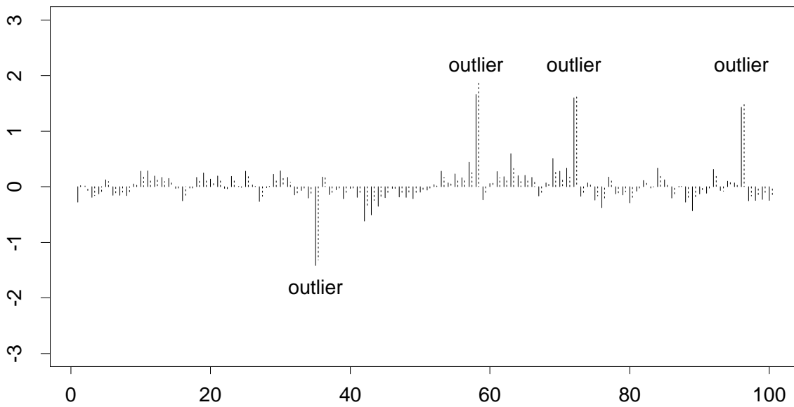
Figure 12: AR(2) with outliers: Observation noise estimated by the direct filter (solid) and the acm.filt (dotted).
