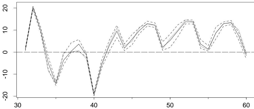
Figure 8: Behavior of Monte Carlo smoother (kernel method) for t = 31, \dots, 60 : State variable (dotted line), 50%-quantiles of Monte Carlo smoother (solid line) and 10%-, 90%-quantiles of Monte Carlo smoother (dashed lines).
