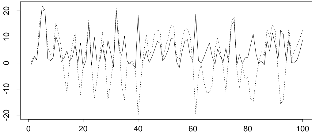
Figure 6: Nonlinear model: Simulated series of observation (solid line) and state variable (dotted line).
