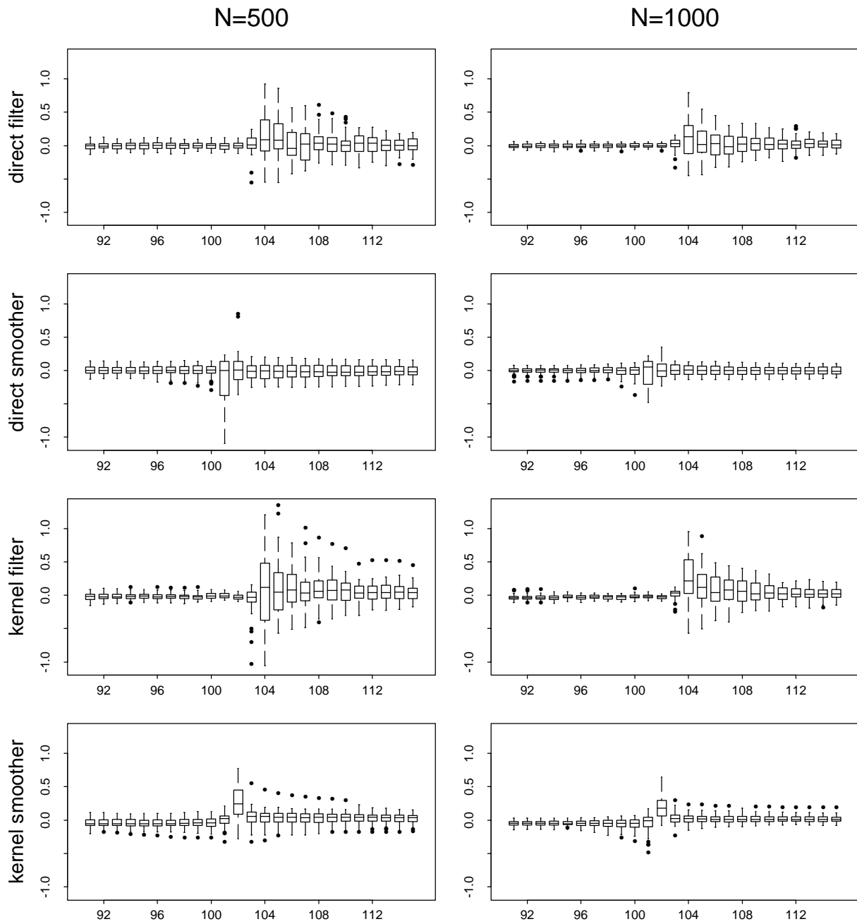
Figure 5: Shifted-mean model: Monte Carlo errors of filters and smoothers.
