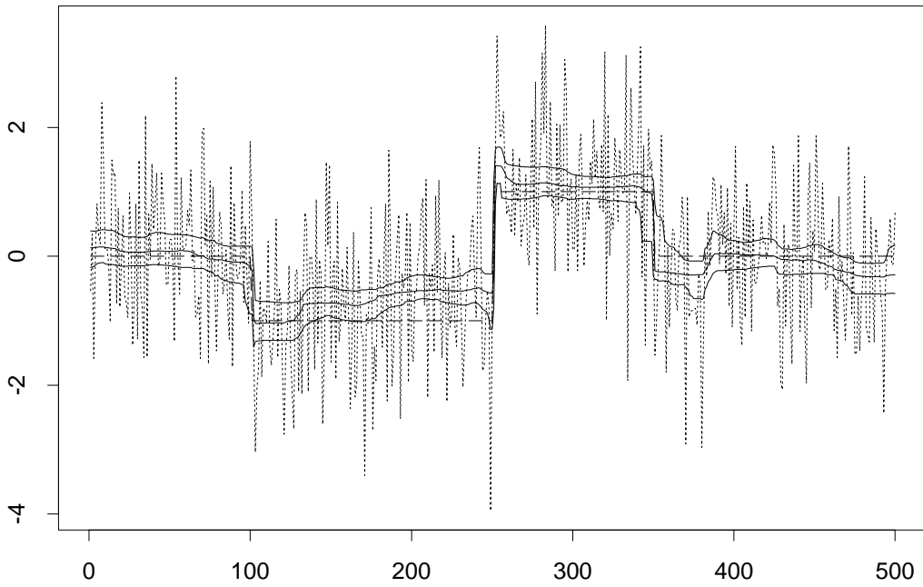
Figure 1: Shifted-mean model: Observations (dotted line) and state variable (dashed line) and the 10%-, 50%- and 90%-quantiles of the Monte Carlo smoother by the direct method (solid lines).
