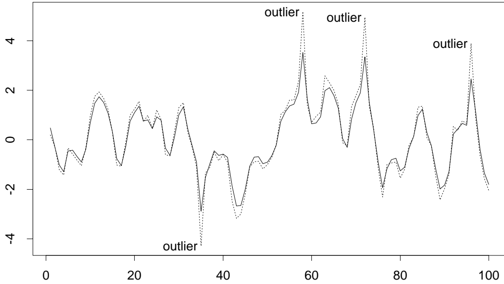
Figure 10: AR(2) with outliers: Mean of the direct filter (solid line) for sample size N=1000 and the observations y_t (dotted line). The four outliers are indicated.
