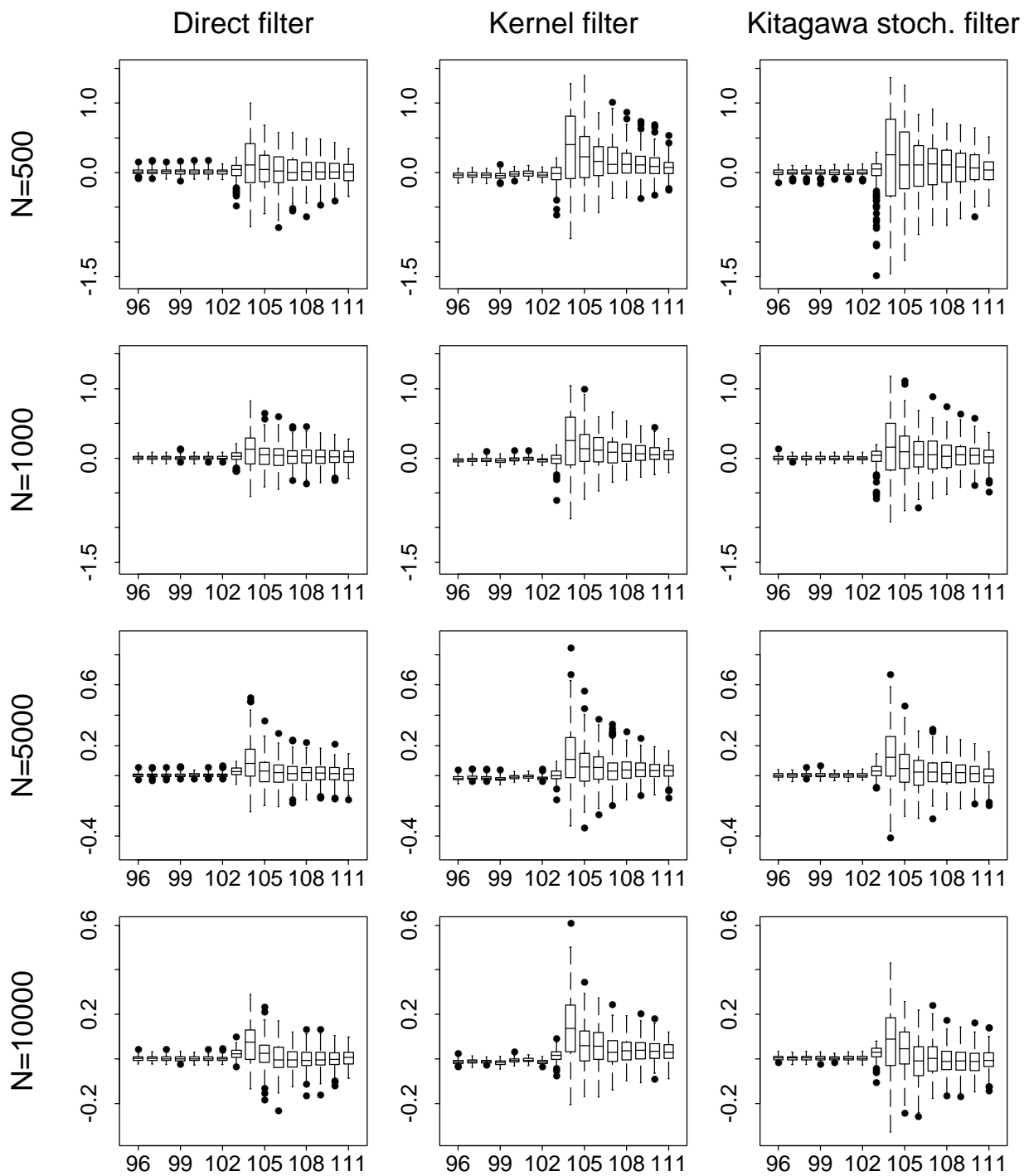
Figure 4: Shifted-mean model: Monte Carlo errors of different filters.
