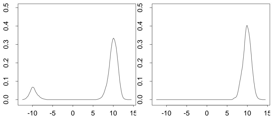
Figure 9: Density Estimation: Filter density (left figure) and smoother density (right figure, T=100 ) at t = 46 obtained by the kernel method.
