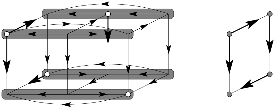
Fig. 6 A USO \psi on the left and its ‘projected’ USO \phi generated by vertices (white) having refined index 1 w.r.t. their hypervertices (shaded)
