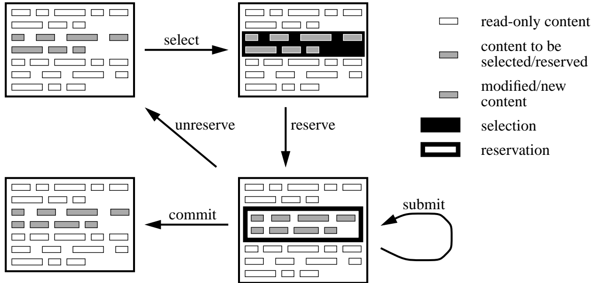
Figure 2: Reservation Model
