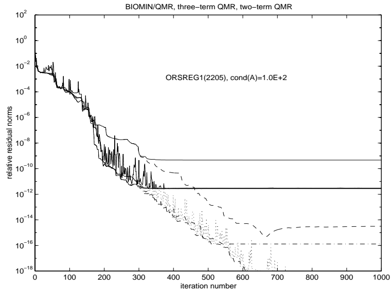
FIG. 6.5. QMR smoothing of standard BiCG (BIOMIN) compared with the QMR method, when applied to a linear system with the matrix ORSREG1 . Relative 2-norms of updated (dots) and true (initially oscillating solid line) residuals of BIOMIN. Comparison with the QMR method and QMR smoothing: updated (lower dashed line) and true (lower solid line) residuals of BIOMIN|QMR, true residuals of standard three-term QMR (upper solid line) and two-term QMR (lower solid line overlapping the one of BIOMIN|QMR), and the quantities \tilde{\rho}_n of three-term QMR (upper dashed line) and two-term QMR (dash-dotted line ending in lowest plateau).
