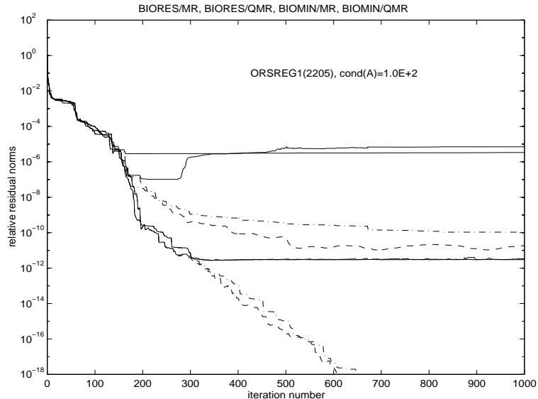
FIG. 6.7. QMR smoothing vs. MR smoothing, both for coupled two-term and three-term BICG, applied to the nonsymmetric system with the matrix ORSREG1 . Relative 2-norms of updated BIOMIN|QMR residuals (lower dashed line) vs. updated BIOMIN|MR residuals (lower dot-dashed line), as well as norms of true BIOMIN|QMR vs. BIOMIN|MR residuals (nearly overlapping lower solid lines). Comparison with norms of updated BIORES|QMR residuals (upper dashed line) and updated BIORES|MR residuals (upper dot-dashed line), as well as norms of true BIORES|QMR residuals (middle solid line) and BIORES|MR residuals (top solid line).
