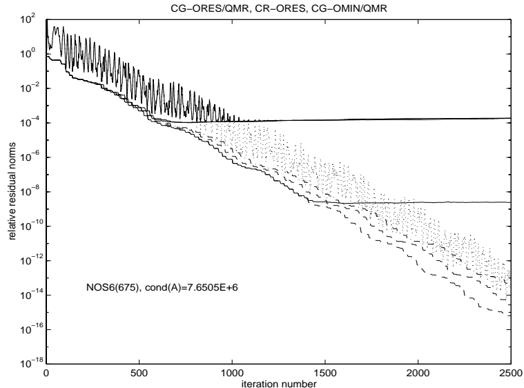
FIG. 6.3. QMR smoothing of coupled two-term CG (CG-OMIN) vs. three-term CG (CG-ORES), applied to the spd system with the matrix NOS6. Relative 2-norms of updated (dots) and true (initially oscillating solid line) residuals of CG-ORES. Comparison with norms of updated (upper dashed line) and true (upper solid line) residuals of CG-ORES|QMR, and with updated (dash-dotted line) and true (overlapping upper solid line) residual norms of CR-ORES. For reference, the norms of the updated (lower dashed line) and true (lower solid line) residuals of CG-OMIN|QMR residuals are shown again.
