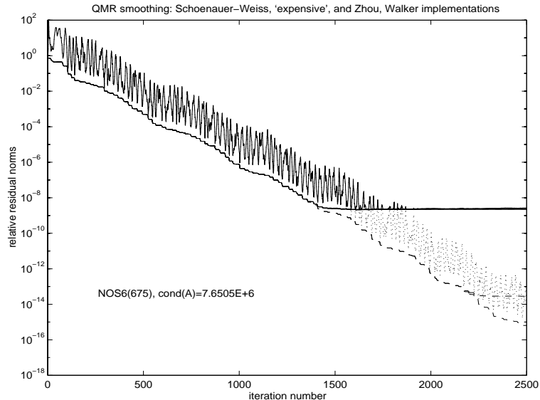
FIG. 6.1. QMR smoothing of Hestenes-Stiefel CG (CG-OMIN) applied to an spd system with the matrix NOS6. Relative 2-norms of updated (dots) and true (initially oscillating solid line) residuals of CG-OMIN. Comparison with three implementations of QMR smoothing applied to the CG results: updated (lower dashed line) and true (solid line) residuals of the Schönauer-Weiss implementation, updated (dashed line ending in lower plateau) and true (solid line) residuals of the Zhou-Walker implementation, and updated (dashed line covered by solid line) and true (solid line) residuals of ‘expensive’ implementation. On the plateau, the four solid lines cannot be distinguished.
