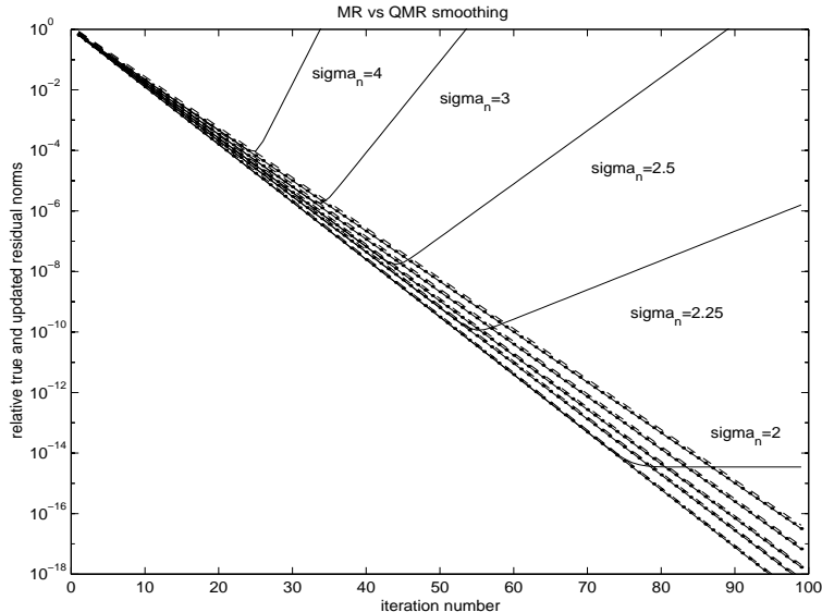
FIG. 3.1. Relative norms of updated (solid lines with dots) and true (solid lines) smoothed residuals obtained by MR smoothing of the sequence of residuals constructed according to (3.5) (relative norms shown as dashed lines) for various choices of the smoothing coefficients \sigma = \sigma_n (independent of n ).
