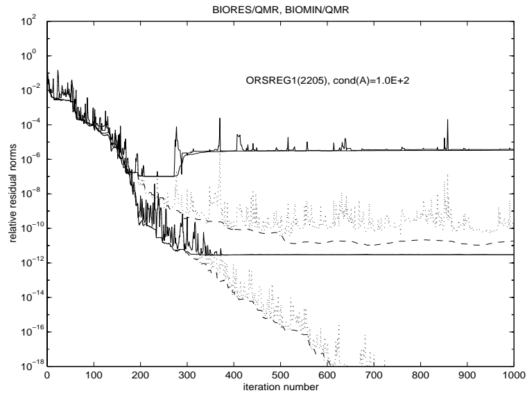
FIG. 6.6. QMR smoothing of coupled two-term BiCG (BIOMIN) vs. coupled three-term BiCG (BIORES), applied to the nonsymmetric system with the matrix ORSREG1 . Relative 2-norms of updated (upper set of dots) and true (initially oscillating top dash-dotted line) residuals of BIORES, and of updated (lower set of dots) and true (initially oscillating solid line) residuals of BIOMIN. QMR-smoothed updated (upper dashed line) and true (top solid line) residuals of BIORES|QMR, and of updated (bottom dashed line) and true (lower solid line, overlapping with the one of BIOMIN) residuals of BIOMIN|QMR.
