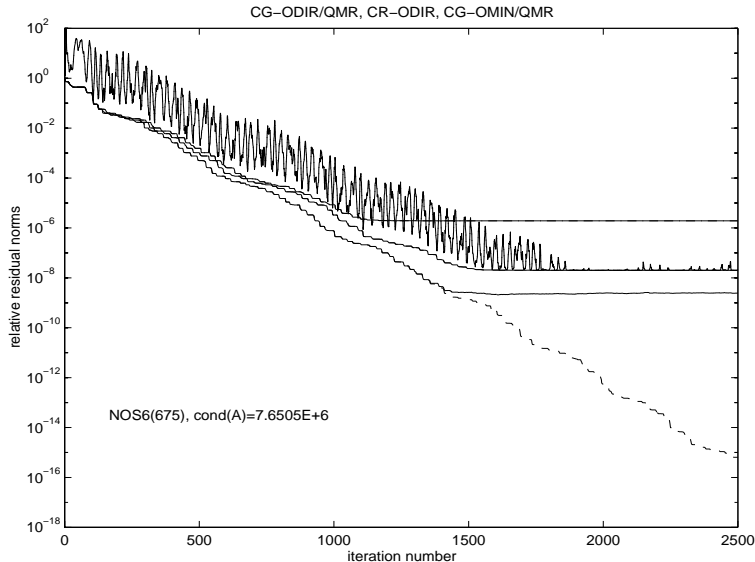
FIG. 6.4. QMR smoothing of coupled two-term CG (CG-OMIN) vs. coupled two/three-term CG (CG-ODIR), applied to the spd system with the matrix NOS6. Relative 2-norms of updated (invisible dots, covered by oscillating solid line) and true (initially oscillating solid line covering the dots) residuals of CG-ODIR. Comparison with the norms of updated (covered upper dashed line) and true (middle solid line covering the dashed line) residuals of CG-ODIR|QMR, and with updated (dash-dotted line covered by upper solid line) and true (top solid line covering the dash-dotted line) residual norms of CR-ODIR. For reference, the norms of the updated (lower, visible dashed line) and the true (bottom solid line) residuals of CG-OMIN|QMR are shown once more.
