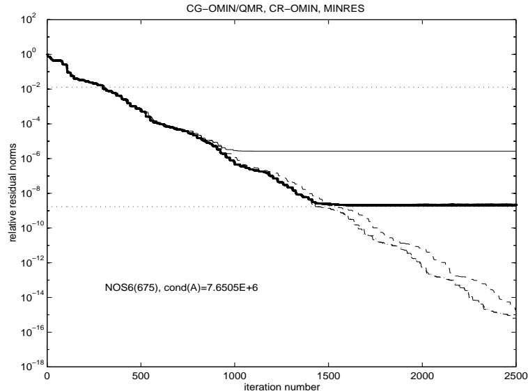
FIG. 6.2. Comparison of QMR-smoothed CG-OMIN with CR-OMIN and MINRES applied to the spd system with the matrix NOS6. Relative 2-norms of true residuals (lower solid line) obtained by QMR smoothing from CG-OMIN. Comparison with the norms of the true residuals of CR-OMIN (overlapping lower solid line) and MINRES (upper solid line). Also shown are the norms of the updated residuals of CG-OMIN|QMR (lower dashed line), and CR-OMIN (mostly overlapping dash-dotted line), and the MINRES quantities \tilde{\rho}_n (upper dashed line), as well as the levels of \kappa(\mathbf{A})\epsilon (lower dotted straight line) and of \kappa^2(\mathbf{A})\epsilon (upper dotted straight line).
