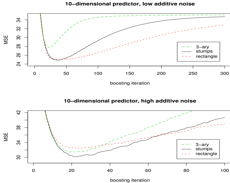
Figure 2: MSE of L_2 Boosting with stumps (solid line), rectangle basis indicator function (short dashed line) as in (4.1) and 3-ary tree with 3 nodes (long dashed line), always with shrinkage factor \nu = 0.1 . Indicator function f(x) as in (4.10). Top: noise variance \sigma_\varepsilon^2 = 0.01 ; Bottom: noise variance \sigma_\varepsilon^2 = 100 . Sample size n = 100 .
