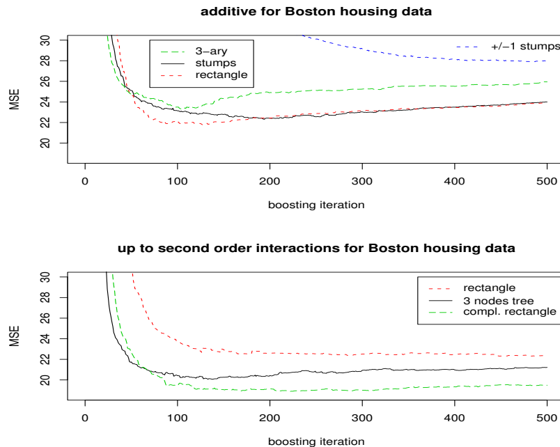
Figure 3: Estimated MSE \mathbb{E}[(\hat{F}_n^m(X) - Y)^2] , via 5-fold cross-validation, for Boston housing data. Top: additive L_2 Boosting fits where every tree or rectangle involves only one predictor variable. L_2 Boosting with stumps (solid line), rectangle indicator basis function (short dashed line) as in (4.1) and 3-ary tree with 3 nodes (long dashed line); in the upper right hand corner, also with \pm 1 -stumps (dashed line) as in (4.2). Bottom: L_2 Boosting fits where every tree or rectangle involves one or two predictor variable (second order interactions). L_2 Boosting with 3 nodes regression tree (solid line), rectangle indicator basis function (short dashed line) as in (4.1) and complementary rectangle indicators (long dashed line) as in (4.8). Always using shrinkage factor \nu = 0.1 .
