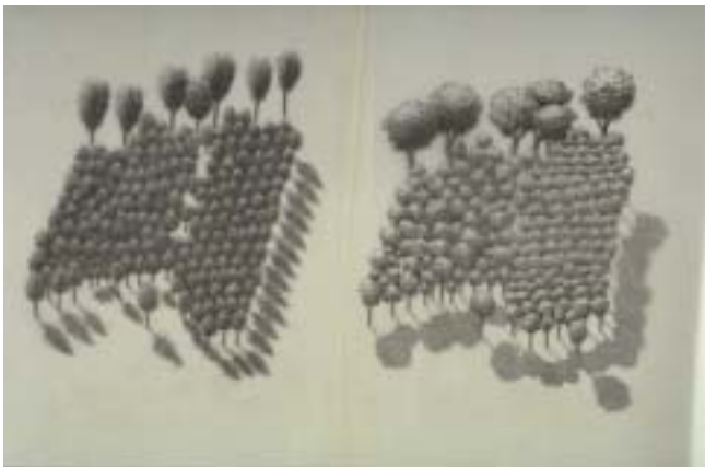
Stangenholz
