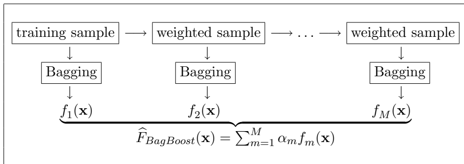
Figure 1: The fundamental idea of BagBoosting
