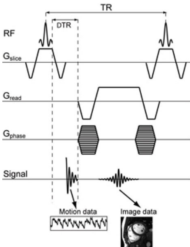
Figure 1 Modified SSFP sequence for self-gating. For motion data acquisition all gradients after the rephasing slice encoding gradient are shifted to record an FID at the k-space center. A prospective self-gated approach for cardiac imaging was successfully implemented and evaluated. Cardiac and respiratory related signal variations were accurately detected in real-time from the repeatedly acquired k-space center. The image quality obtained is comparable to retrospective and ECG-triggered approaches.
