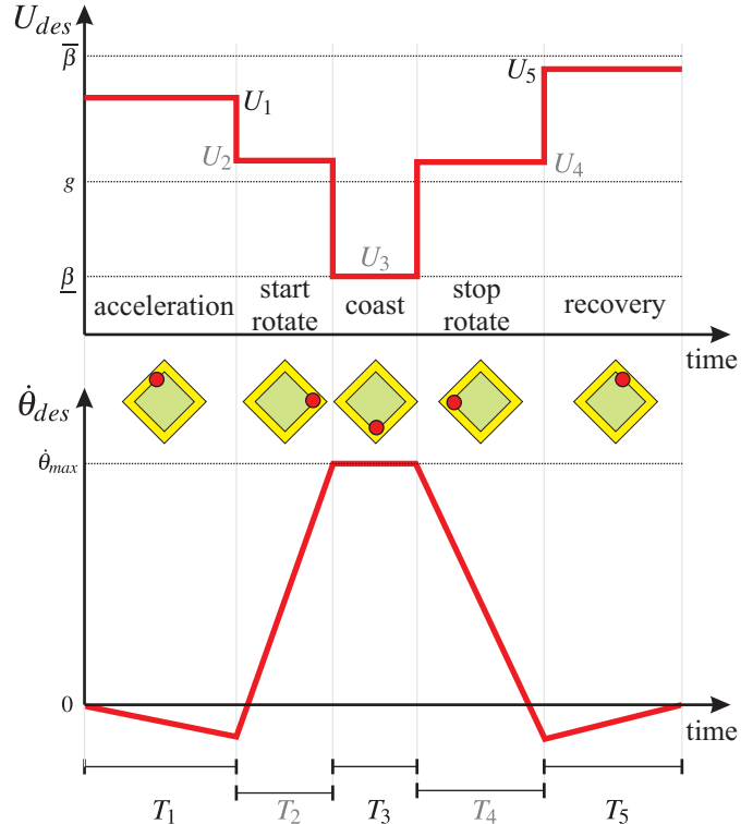
Fig. 5. The collective thrust and commanded angular rate profile of the multi-flip maneuver, with control actions depicted with respect to the reduced control envelope at each stage of the primitive. Note that the grayed out variables along with the rest of the profile are fully determined by the five selected parameters.
