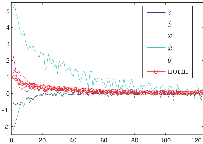
Fig. 11. Final state error and parameter evolution over 124 iterations for a vehicle with \dot{\theta}_{max} = 1300^\circ/s using J and P_0 calculated for \theta_{max} = 1600^\circ/s . Step size \gamma = 0.07 . Note that \theta_f is normalized to (-\pi, \pi) .
