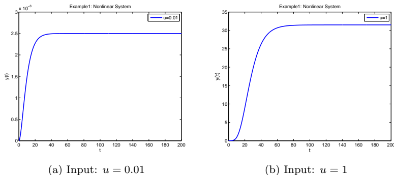
Figure 4.2: The simulated output of system 4.1, for the following parameter values: a_1 = a_2 = a_3 = K_i = K_e = 0.1 and initial condition (0, 0, 0) . Total simulation time: 200 seconds. The qualitative behavior of the system is the same, regardless of the input value.
