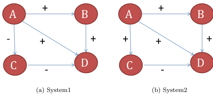
Figure 1: Example networks
