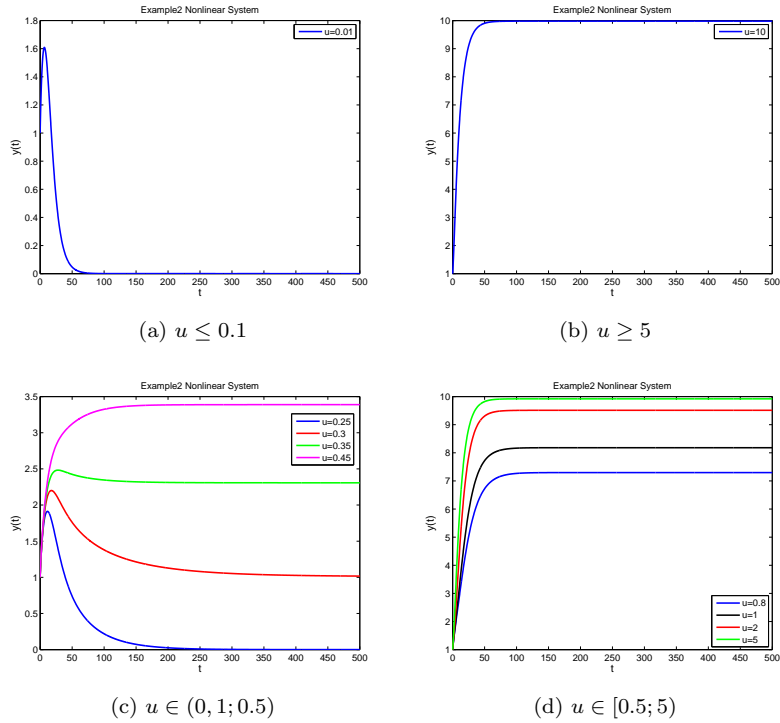
Figure 4.4: The simulated output for system 4.8, for the following parameter values: a_1 = a_2 = b_1 = b_2 = c_1 = c_2 = 0.1 , \hat{\sigma}_1 = \hat{\sigma}_2 = \hat{K}_2 = 1 , \hat{K}_1 = 2 and initial condition (1, 1, 1, 1) . Total simulation time: 500 seconds. For inputs u \leq 0.1 , the output is invariant to the input and its qualitative behavior is the one from subfigure 4.4a. For inputs u \geq 5 , the output reaches saturation and it becomes invariant to the input as well, as it can be seen in subfigure 4.4b. Subfigure 4.4c shows the qualitatively different outputs for inputs in the range (0, 1; 0.5) and subfigure 4.4d shows the qualitatively similar outputs when the input is in the range of [0.5; 5) , scaling with the input value until the output reaches saturation.
