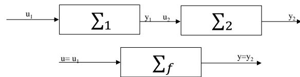
(a) Cascade interconnection of two systems.
