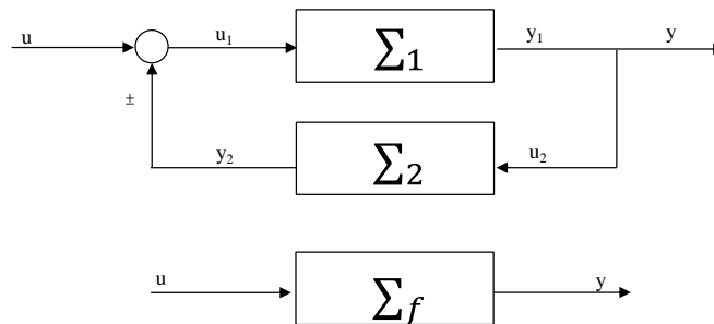
(b) Feedback interconnection of two systems
