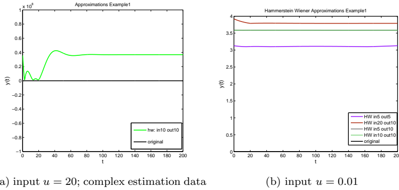
Figure 5.3: Comparison of simulated output for Hammerstein Wiener identified models for system 4.2, simulated under the following parameter values: a_1 = a_2 = a_3 = K_i = K_e = 0.1 and initial condition (0, 0, 0) . Total simulation time: 200 seconds. in represents the number of units in the input nonlinearity, while out represents the number of units in the output nonlinearity. In subfigure 5.3a, the estimation was performed on a complex dataset, consisting of signals of different types, while in subfigure 5.3b, all the approximations previously performing well in figure 5.2, on different inputs, failed under the input 0.01
