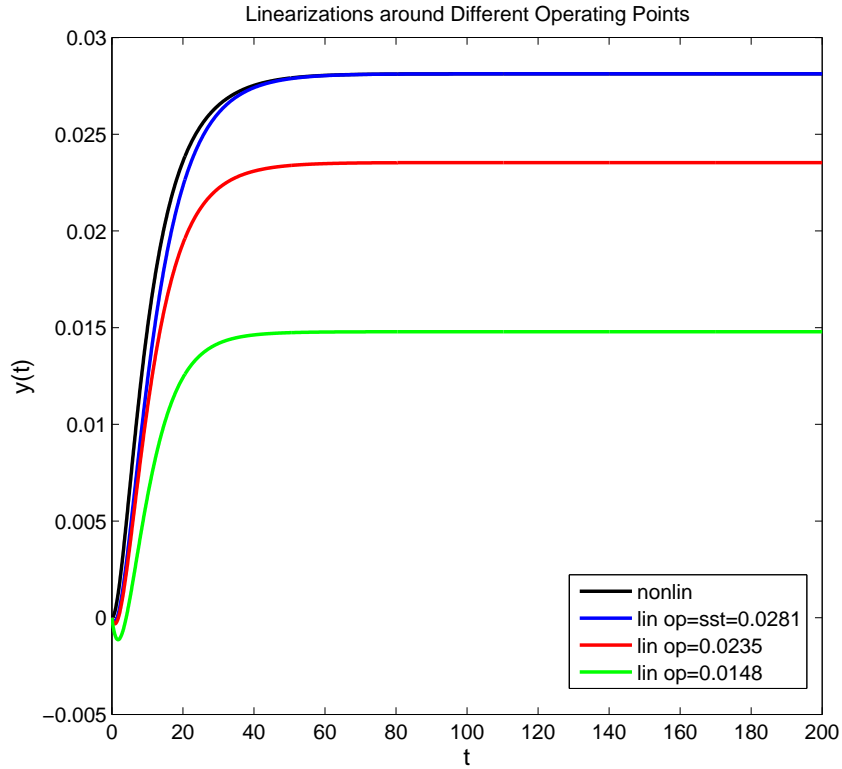
Figure 1.1: Simulated output for system 1.15 under the following parameter values: a_1 = a_2 = a_3 = K_i = K_e = 0.1 , initial condition (p(0), q(0), r(0)) = (0, 0, 0) and constant input u(t) \equiv 0.1 . nonlin represents the output of the original system, lin op=sst represents the trajectory of the linearization done around the steady state, while the other two curves represent trajectories of linearizations done around the non-steady-state specified operating points. The similarity between the nonlinear outputs and the linear ones is the highest when the linearization is done around the steady state.
