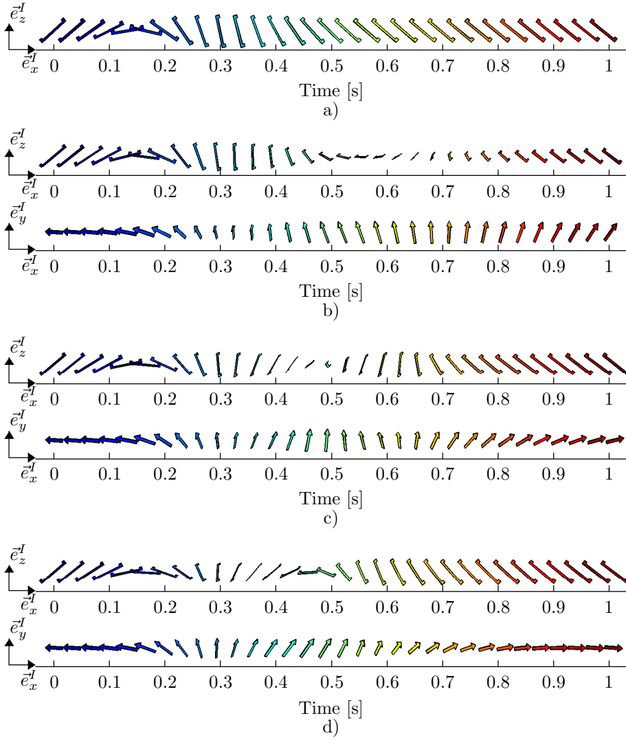
Figure 10: View of the quadcopter in the xz -plane and xy -plane respectively for different prioritization factors: a) p = 0.0 , b) p = 0.133 , c) p = 0.267 and d) p = 0.4 .
