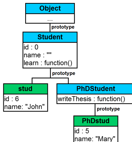
Fig. 2.1: Objects and their prototypes in JavaScript
