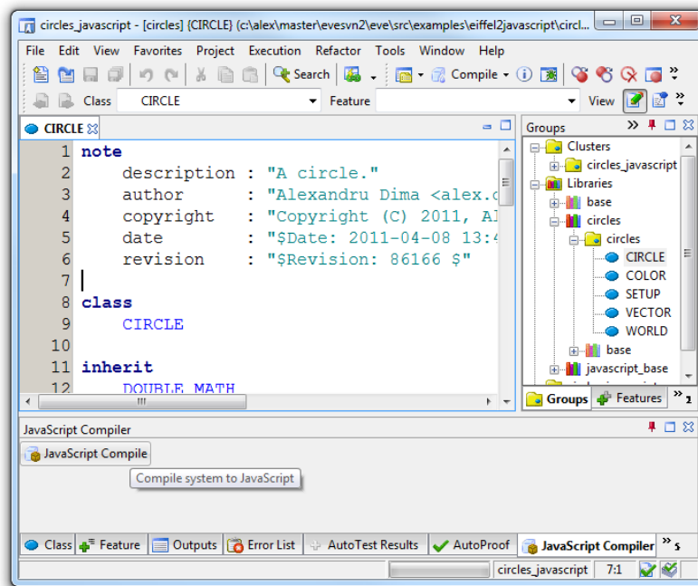
Fig. 3.1: Invoking the translator over the current project
