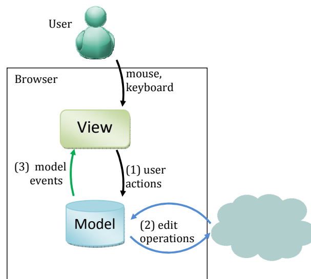
Fig. 4.3: Events in the editor
