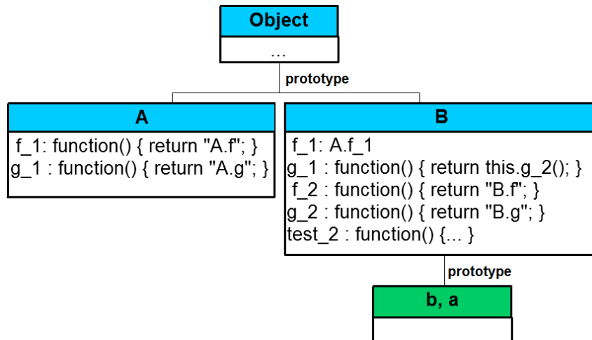
Fig. 2.3: Objects and their prototypes in JavaScript
