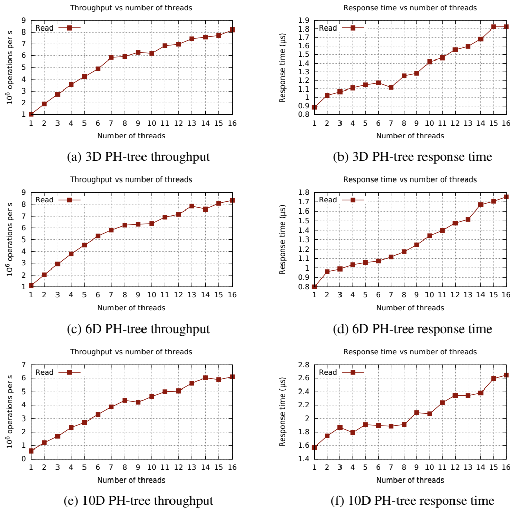
Figure 6.4: Evolution of read throughput and response time for the PH-tree
