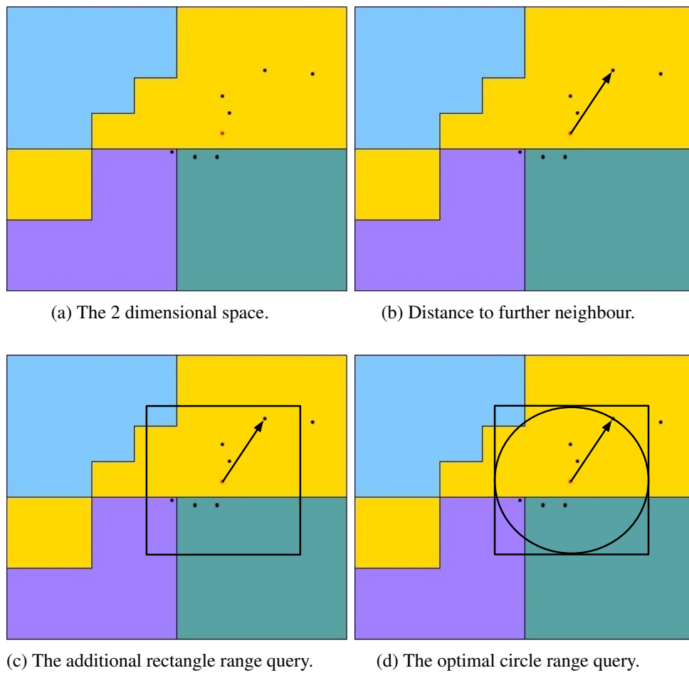
Figure 3.12: Illustration of a 3 nearest neighbour query execution in a 2 dimensional space.
