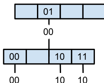
Figure 2.1: 2 dimensional 4bit PH-tree containing the points: (0000, 1000), (0011, 1000), (0011, 1010).
