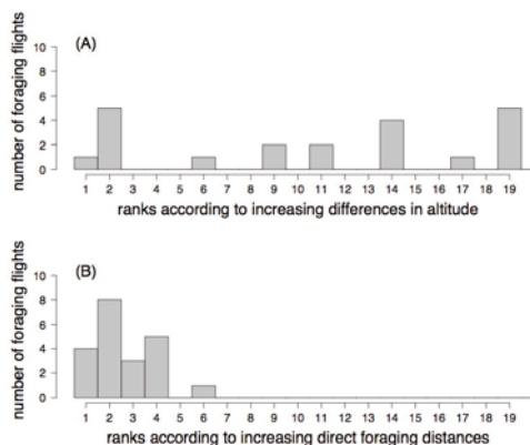
Figure 3. Total number of foraging flights of Chelostoma florissomne per rank with respect to (A) the difference in altitude from each nesting site and (B) the minimum direct distance to each nesting site. Rank 1 represents the Ranunculus patches with the least difference in altitude from each of the four nesting sites and the closest patches from each of the four nesting sites, respectively.
