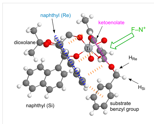
Figure 8: Excerpt from the X-ray structure of a catalyst/substrate complex [Ti(1-naphthyl-TADDOLato)(β-ketoenolate) 2 ] [102]. Two important attractive interactions between substrate and TADDOL ligand fragments can be identified: 1. Face-to-face arrangement of the ligand 1-naphthyl group and the substrate ketoenolate plane; 2. edge-to-face stacking interaction between the ligand naphthyl and the substrate benzyl ester groups.
