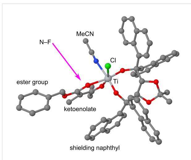
Figure 7: Steric model explaining the face selectivity observed in the titanium–TADDOLate complex catalyzed fluorination. The structural model of this complex [TiCl(TADDOLate)(β-ketoenolate)(MeCN)] of the type B (Scheme 7) was obtained by combining X-ray data of K2 with a modeled structure of the enol of substrate 10 . The arrow symbolizes the external attack of the fluorinating reagent N–F.
