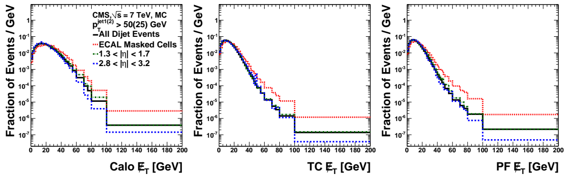
Figure 4. Distribution of (left) Calo \cancel{E}_T , (middle) TC \cancel{E}_T , and (right) PF \cancel{E}_T , normalized to unit area, for events containing at least 2 jets with p_T^{\text{jet1}(2)} > 50 (25) GeV (black solid), and for the subsets of these events with a jet aligned with \vec{\cancel{E}}_T within \Delta\phi(\vec{\cancel{E}}_T, \text{jet}) < 0.2 and pointing towards a masked ECAL cell (red dotted), the barrel-endcap boundary (green dot-dashed), and the endcap-forward boundary (blue dashed) in simulation.
