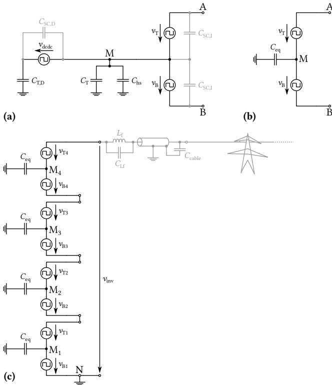
Fig. 4.13: (a) Common-mode equivalent circuit of a converter cell shown in Fig. 4.2a, including “local” common-mode effects and the DC-DC converter; (b) reduced version suitable for the analysis of “global” common-mode effects; and (c) corresponding common-mode equivalent circuit of a complete phase stack.
