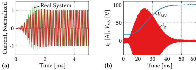
Fig. 4.12: (a) Comparison of the measured step responses of the real and the scaled system; (b) measurement of the scaled system’s startup with an initially empty MV-side DC link.
