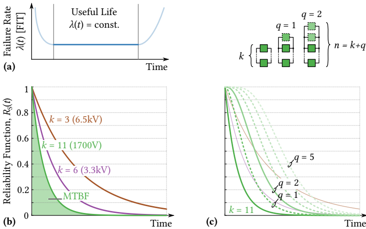
Fig. 2.16: (a) Typical evolution of a component’s failure rate over time (“bathtub curve”); (b) reliability function in dependence of the number of elements (cascaded cells with equal failure rate per cell), where the system-level MTBF_S is indicated as the area below the reliability function, and (c) improvement of the reliability by adding q redundant cells to the k cells strictly required for system operation.
