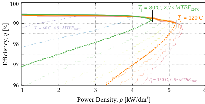
Fig. 2.20: Reliability versus power density trade-off for a design based on 1700 V/150 A IGBTs; no redundancy is considered.
