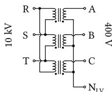
Fig. 4.28: Circuit schematic of a delta-wye connected LFT.
