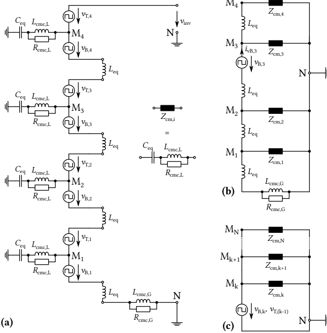
Fig. 4.19: (a) Common-mode equivalent circuit including parasitic inductances as well as local, i. e., per cell, common-mode chokes (CMCs), L_{cmc,L} , and a global, i. e., per phase, CMC, L_{cmc,G} . (b) Corresponding equivalent circuit for the case of a switching transition of the equivalent voltage source v_{B,3} . (c) Simplified and generalized equivalent circuit suitable for designing the local CMCs.
