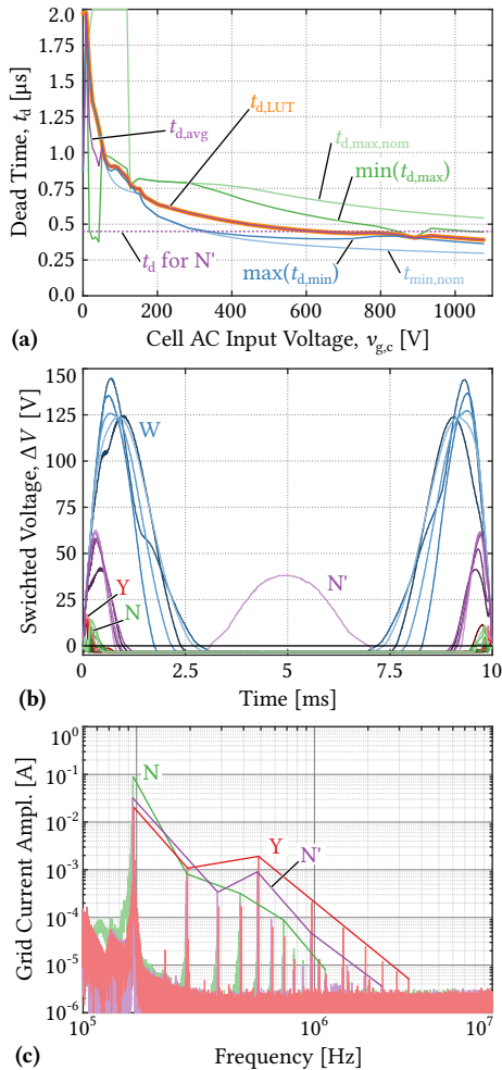
Fig. 5.23: (a) Valid t_d range for design N and chosen t_{d,LUT} for the look-up table used in the full-system simulation; (b) simulated \Delta V of the five converter cells for different designs (cf. Fig. 5.21), and (c) corresponding grid current spectra.
