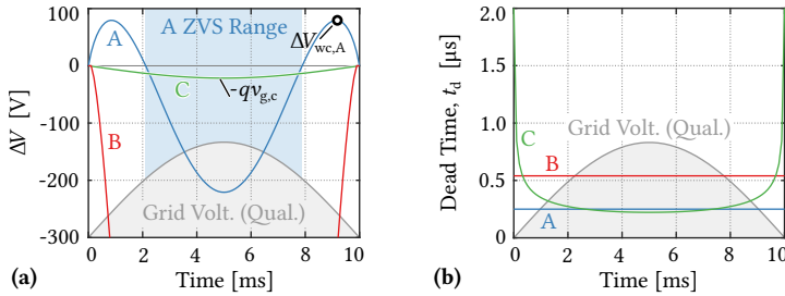
Fig. 5.17: (a) Switched voltage, \Delta V , over half a grid period for the three example designs from Fig. 5.16c and Tbl. 5.5. For design A, also the worst-case switched voltage, \Delta V_{wc} is indicated. (b) shows the corresponding dead times, t_d , over half a grid period.
