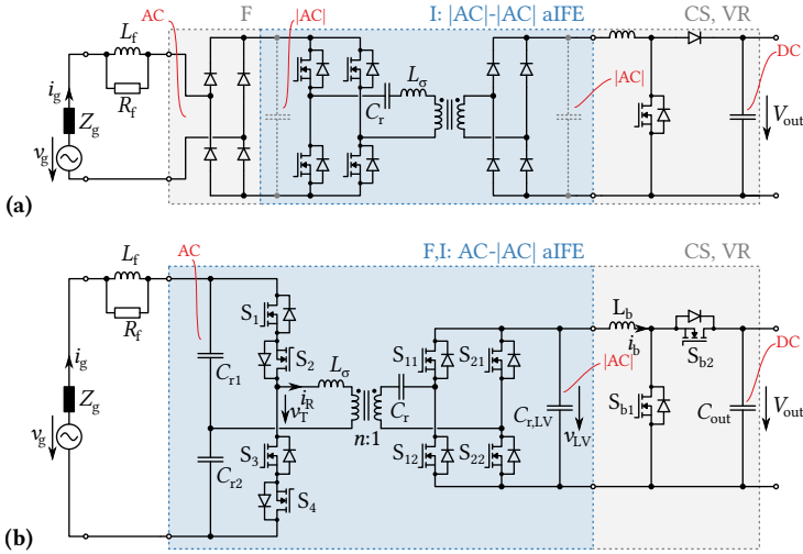
Fig. 5.3: (a) Unidirectional and (b) bidirectional single-cell IFE power circuit topologies. Note that C_{r1} , C_{r2} , C_r , and C_{r,LV} are resonant capacitors, not (large capacitance) DC link capacitors.
