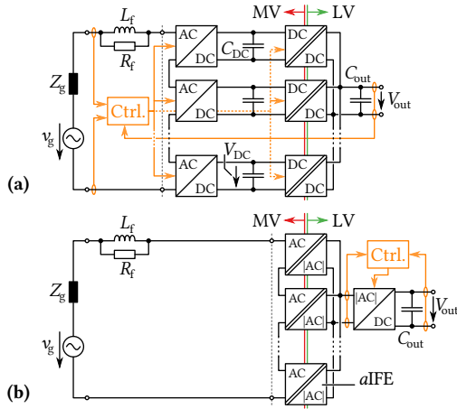
Fig. 5.2: (a) IBE and (b) IFE systems in ISOP configuration.
