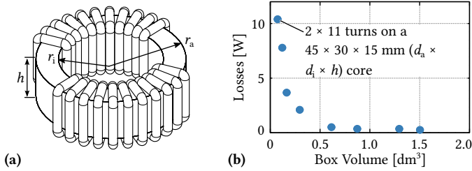
Fig. 4.27: (a) Geometric dimensions of the considered CMC and (b) thermally feasible CMC designs based on standard Vitroperm cores.
