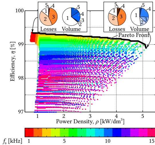
Fig. 3.23: Resulting designs in the \eta\rho -plane with C_p = 0.7 ; the Pareto front is highlighted and relative loss and volume distribution for the two extreme points of the Pareto front are shown: 1) transformer, 2) LV semiconductors, 3) MV semiconductors, 4) DC links, 5) resonant capacitors.
