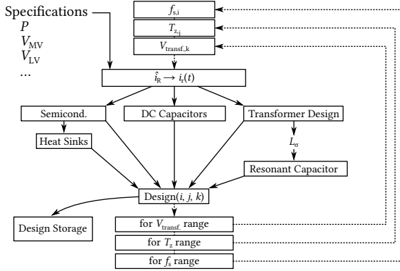
Fig. 3.22: Visualization of the procedure that calculates the design points used to find the Pareto front shown in Fig. 3.23 .
