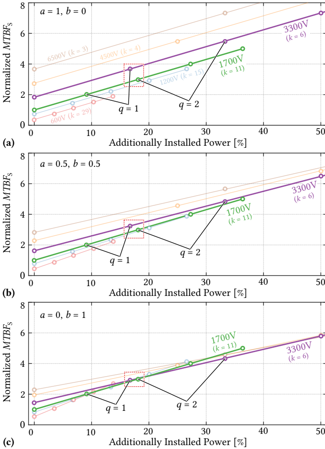
Fig. 2.17: Standby redundancy: MTBF_s (normalized to the 1700 V design without redundancy) versus additionally installed power capability for different blocking voltages (and therefore different numbers of required cells, k ). (a) considers a constant failure rate per cell ( a = 1, b = 0 ), (b) a 1:1 distribution between a constant and a blocking-voltage dependent part of the cells' failure rates ( a = 0.5, b = 0.5 ), and (c) only a blocking-voltage dependent part ( a = 0, b = 1 ).
