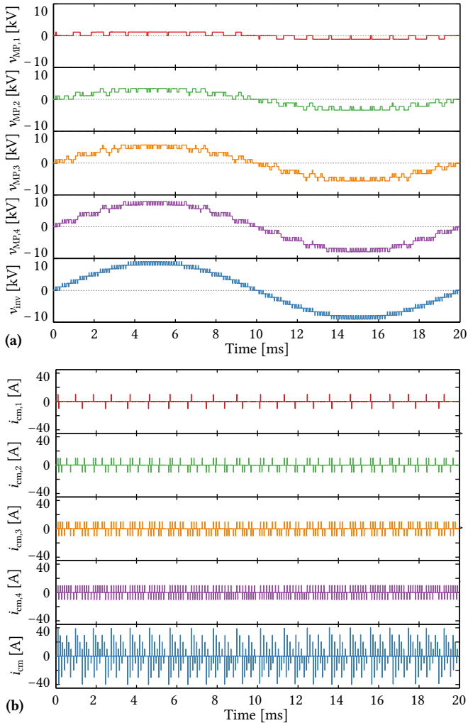
Fig. 4.15: Full-system simulation results for one SST phase considering C_{eq} = 650 pF and a dv/dt of 15 kV/ \mu s. (a) shows the voltages between the cell midpoints and ground as well as the total phase stack output voltage, v_{inv} , and (b) shows the corresponding common-mode currents flowing through the cell's parasitic capacitances to ground, and also the total common-mode current, i_{cm} , flowing back through the node N.
