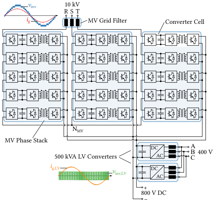
Fig. 4.1: Topology overview of the MEGALink SST, including key voltage and current waveforms on the MV and LV grid sides, respectively.
