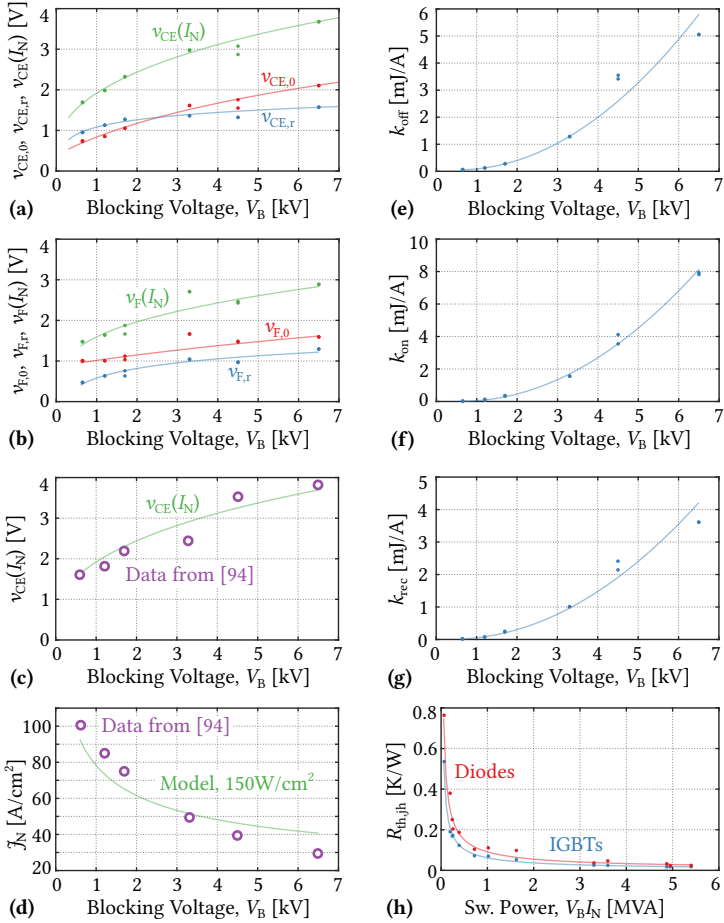
Fig. 2.4: Datasheet values for the loss-relevant IGBT and diode parameters and fitted analytical approximations for (a) IGBT conduction losses, (b) diode conduction losses, (e) normalized turn-off losses, (f) normalized turn-on losses, (g) normalized diode recovery losses, and (h) thermal resistances from junction to heat sink; (c) compares the conduction loss model with typical data for the forward voltage at rated current from [94], and (d) does the same for the corresponding nominal current densities.
