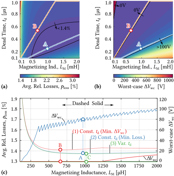
Fig. 5.16: Results for the analytic ZVS considerations using the model from Fig. 5.13 and the routine shown in Fig. 5.15. (a) averaged relative losses, p_{\text{loss}} , and (b) worst-case switched voltage, \Delta V_{\text{wc}} , in dependence of \{L_M, t_d\} . Following the highlighted trajectories in (a) and (b), (c) shows the corresponding dependencies of p_{\text{loss}} (dashed lines) and \Delta V_{\text{wc}} (solid lines) on the magnetizing inductance (note that the respective values of t_d are according to the trajectories given in (a) and (b)). The blue trajectory (trace 1) corresponds to minimum p_{\text{loss}} , the red trajectory (trace 2) corresponds to minimum \Delta V_{\text{wc}} , and trace 3 is for a variable dead time, the minimum possible losses (design B) are higher than the minimum possible losses without full-range ZVS (design A). If the dead time is variable, low losses and full-range ZVS can be obtained (design C). Note that the ragged appearance of the \Delta V_{\text{wc}} trace is due to the limited resolution of the L_M and t_d search ranges.
