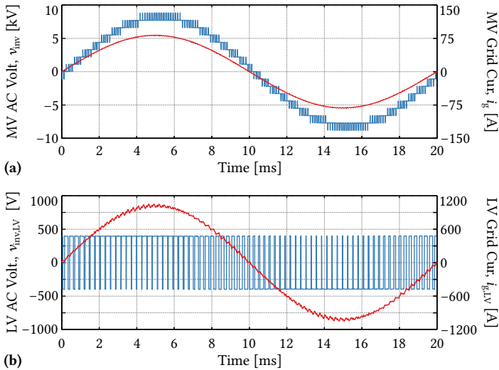
Fig. 4.30: (a) MV-side inverter voltage and resulting line current for (a) the cascaded 1000 kVA MV converter, and (b) corresponding LV-side waveforms for one of the 500 kVA LV converter units (cf. Fig. 4.1) for full-load active power operation.
