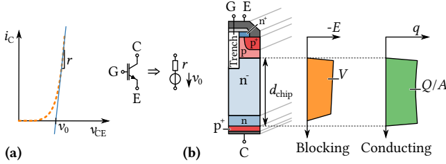
Fig. 2.3: (a) Approximation of an IGBT (or diode) forward characteristic by v_0 and r , and (b) schematic cross section (not to scale) of a trench/field-stop IGBT with qualitative drift region field distribution in the blocking state and qualitative charge carrier concentration in the conducting state [92]. The integral of the electric field corresponds to the applied reverse voltage, and the integral of the charge carrier density along d_{chip} gives the stored charge per chip area.
