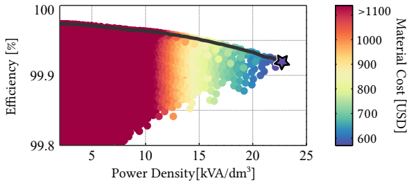
Fig. 4.31: Pareto optimization of the MV filter inductors with the chosen design highlighted.
