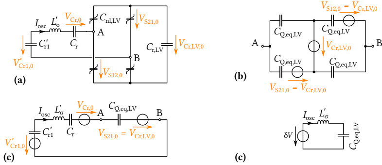
Fig. 5.20: Derivation of the equivalent circuit for the simplified calculation of HF oscillations during the zero-current interval (cf. Fig. 5.19). All quantities are referred to the LV side of the transformer. (a) Relevant part of the full circuit shown in Fig. 5.18; (b) simplification of the LV-side bridge, where C_{nl,LV} is replaced by the charge equivalent capacitance, C_{Q,eq,LV} , and where C_{r,LV} is neglected because C_{r,LV} \gg C_{Q,eq,LV} ; (c) intermediate simplification step where the circuit part from (b) has been replaced by its Thévenin equivalent; and (d) final equivalent circuit where all initial conditions are summarized as a voltage source, \delta V , and where C'_{r1} \gg C_{Q,eq,LV} and C_r \gg C_{Q,eq,LV} are neglected.
