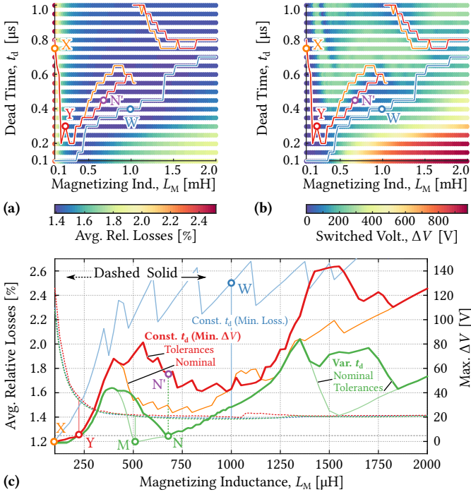
Fig. 5.21: Results of the advanced ZVS considerations. (a) averaged relative losses, p_{\text{loss}} , and (b) worst-case switched voltage, \Delta V_{\text{wc}} , in dependence of \{L_M, t_d\} . Following the highlighted trajectories in (a) and (b), (c) shows the corresponding dependencies of p_{\text{loss}} (dashed lines) and \Delta V_{\text{wc}} (solid lines) on the magnetizing inductance (note that the respective values of t_d are according to the trajectories given in (a) and (b)). The blue trajectory corresponds to minimum p_{\text{loss}} , the orange trajectory is for minimum \Delta V_{\text{wc}} assuming switching at t_{\text{off},1} , and the red trajectory is for minimum \Delta V_{\text{wc}} considering all four switching conditions, i. e., switching at t_{\text{off},1\dots 4} . The green curves in (c) are for cases where t_d is varied during the grid period such as to achieve minimum \Delta V_{\text{wc}} for a given L_M ; the bold curve considers component tolerances among the converter cells by taking into account the four different sets of initial conditions (cf. Fig. 5.19). Please refer to the text for a detailed explanation of the different highlighted designs. Note that the ragged appearance of the \Delta V_{\text{wc}} traces is due to the limited resolution of the L_M and t_d search ranges.
