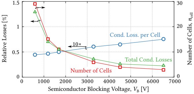
Fig. 2.12: Conduction losses per cell and total conduction losses, and number of cells used in the Pareto optimization as a function the blocking voltage. Note that the conduction losses per cell (blue curve) are multiplied by a factor of 10 for better visibility. Even though the losses per cell are increasing with the blocking voltage, the total conduction losses decrease because n_{\text{cell}} \propto 1/V_B .
