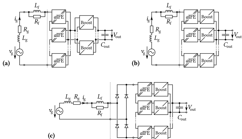
Fig. 5.6: Three ISOP configuration variants of the IFE topology; (a) common |AC| LV-side bus and single boost stage employing interleaved sub-units, (b) one boost stage per aIFE cell, and (c) common input rectifier using HV semiconductors (possibly realized as a synchronous rectifier by adding anti-parallel switches to the diodes).
