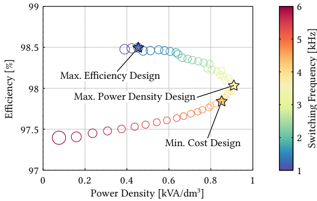
Fig. 4.35: Different design variants of a 500 kVA LV converter for 10 % peak-to-peak current ripple and different switching frequencies. The size of the circles indicates the designs' material costs.
