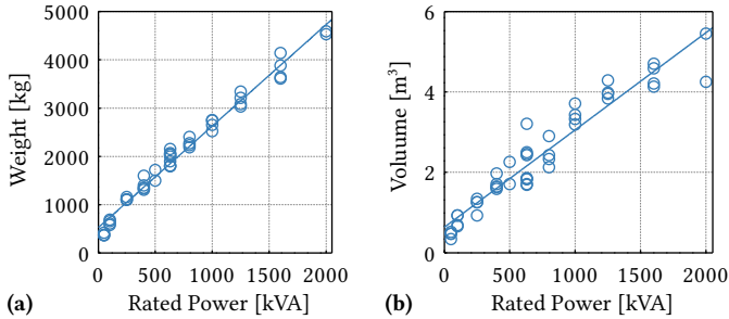
Fig. 4.29: Dependence of LFT weight (a) and volume (b) on the rated power; based on datasheet information from [166].
