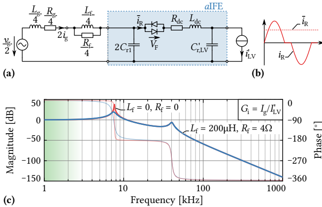
Fig. 5.5: (a, b) Dynamic equivalent circuit (referred to the MV side of the MFT) of the aIFE converter including input filter and grid impedances, and (c) corresponding transfer function from the boost stage inductor current to the grid current, G_i(s) , using the specifications from Tbl. 5.1 scaled to one instead of five cells. The resulting model parameters are L_{dc} = 26.7\ \mu\text{H} and R_{dc} = 510\ \text{m}\Omega ; furthermore, C_{r1} = 0.68\ \mu\text{F} , C_{r,LV} = 3.5\ \mu\text{F} , L_g = 690\ \mu\text{H} and R_g = 22\ \text{m}\Omega have been used for the calculation of the exemplary transfer function.
