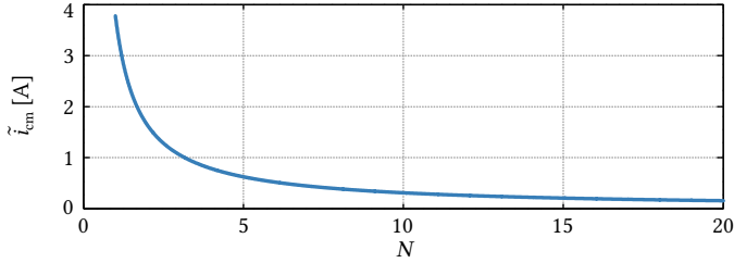
Fig. 4.18: Total RMS common-mode current, \tilde{i}_{cm} , as a function of the number of cascaded converter cells, N .
