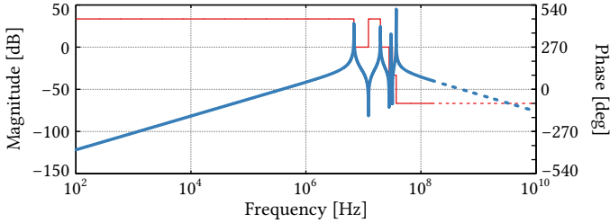
Fig. 4.20: Bode plot of the transfer function G_3(s) (cf. Fig. 4.19b ) for C_{eq} = 650 \mu\text{F} and L_{eq} = 100 \text{ nH} and without any CMCs, i. e., L_{cmc,G} = L_{cmc,L} = 0 \text{ H} .
