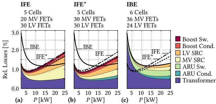
Fig. 6.4: Relative semiconductor and transformer losses for the three systems considered in the case study.
