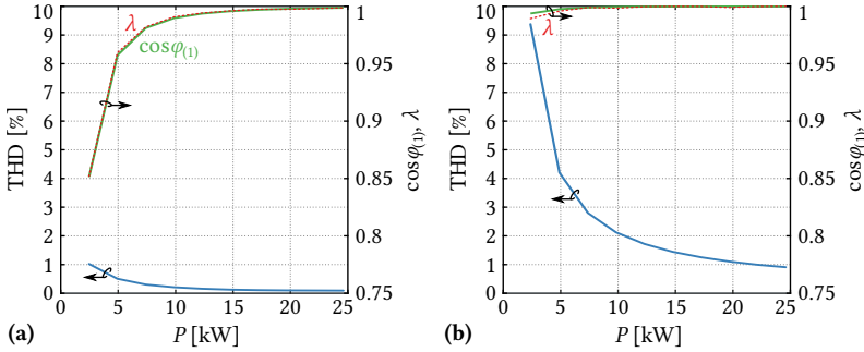
Fig. 5.26: Fundamental-frequency power factor, \cos \varphi_{(1)} , power factor, \lambda , and THD in dependence of the output power (a) without and (b) with compensation of the capacitive reactive power of the MV-side resonant capacitors.
