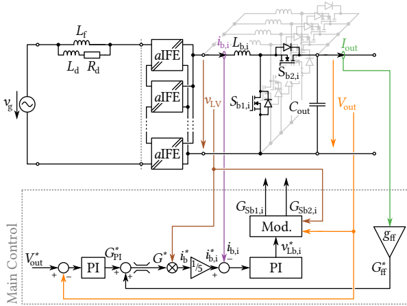
Fig. 5.24: Overview of the S 3 T’s control structure that utilizes only LV-side measurements (input polarity estimation not shown).
