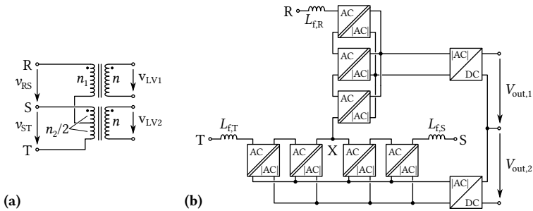
Fig. 5.11: (a) Magnetic Scott transformer, (b) IFE-based Scott transformer configuration.
