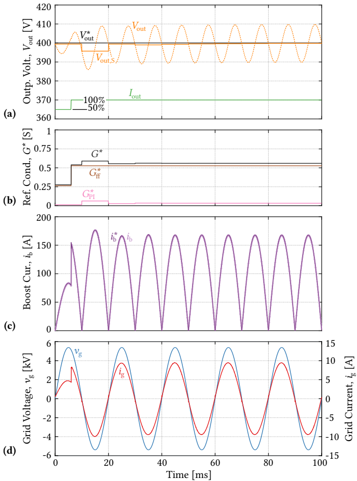
Fig. 5.25: Simulated controller behavior for a step from 50 % to 100 % (rated) load current. (a) Output voltage, (b) reference conductances, (c) boost inductor current reference and real value (note: superposition of the individual stages' boost currents that is seen by the a IFE stage), and (d) MV-side grid voltage and current.
