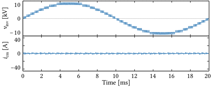
Fig. 4.26: Simulated phase stack output voltage, v_{inv} , and total common-mode current, i_{cm} , for the case of optimally damped local CMCs.
