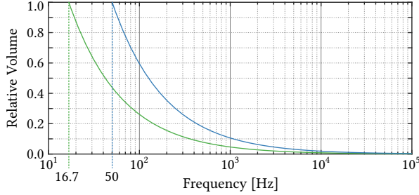
Fig. 1.4: Scaling of transformer volume with frequency (for constant power and given k_W, J_{\text{rms}} and \hat{B}_{\text{max}} ) according to (1.1); for two initial operating frequencies (related to 100 % volume) of 16.7 Hz and 50 Hz, respectively.
