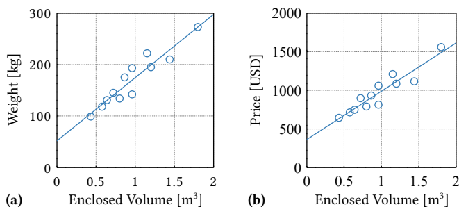
Fig. 4.32: Dependence of (a) cabinet weight and (b) price on the enclosed volume.
