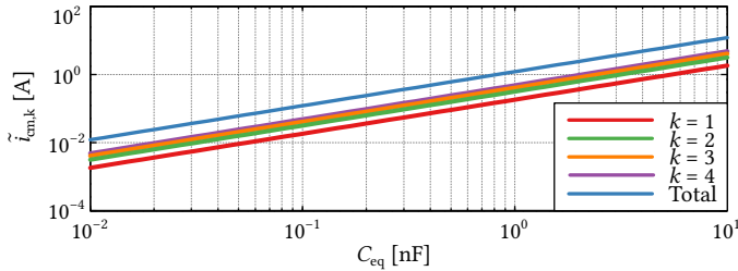
Fig. 4.17: Dependence of the individual cells' RMS common-mode currents, \tilde{i}_{\text{cm},k} , and of the total RMS common-mode current, \tilde{i}_{\text{cm}} , on C_{\text{eq}} .
