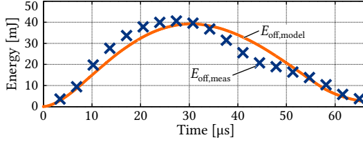
Fig. 3.21: Measurement and estimate of the turn-off losses in S_1 at T_j = 125^\circ\text{C} . The \Delta t values used for the measurements are the same as in Fig. 3.16 .
