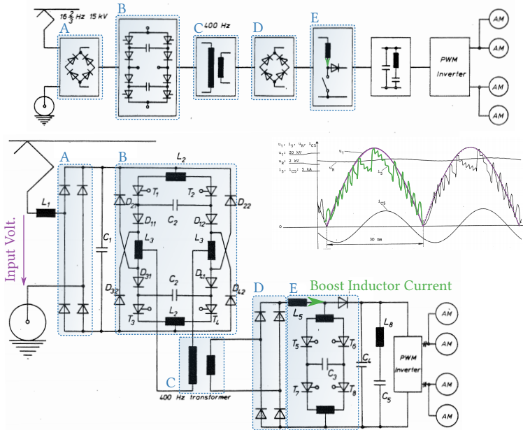
Fig. 1.11: Topology to “eliminate the 16\frac{2}{3} Hz main transformer on electrical traction vehicles” as proposed by Weiss in 1985 [55], where the control stage (boost converter, E) is placed on the secondary side of the MF isolation stage (B-C-D), resulting in an isolated front end (IFE) approach. The figure is from [55], and colors have been added by the author.
