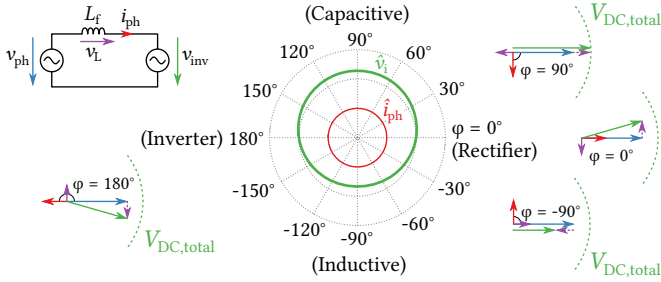
Fig. 2.9: Dependence of the required inverter output voltage amplitude, \hat{v}_i = M \cdot V_{DC,total} , on the phase angle between voltage and current, \varphi . The capacitive operating point ( \varphi = 90^\circ ) limits the maximum feasible filter inductance, L_f , for a given total DC voltage.
