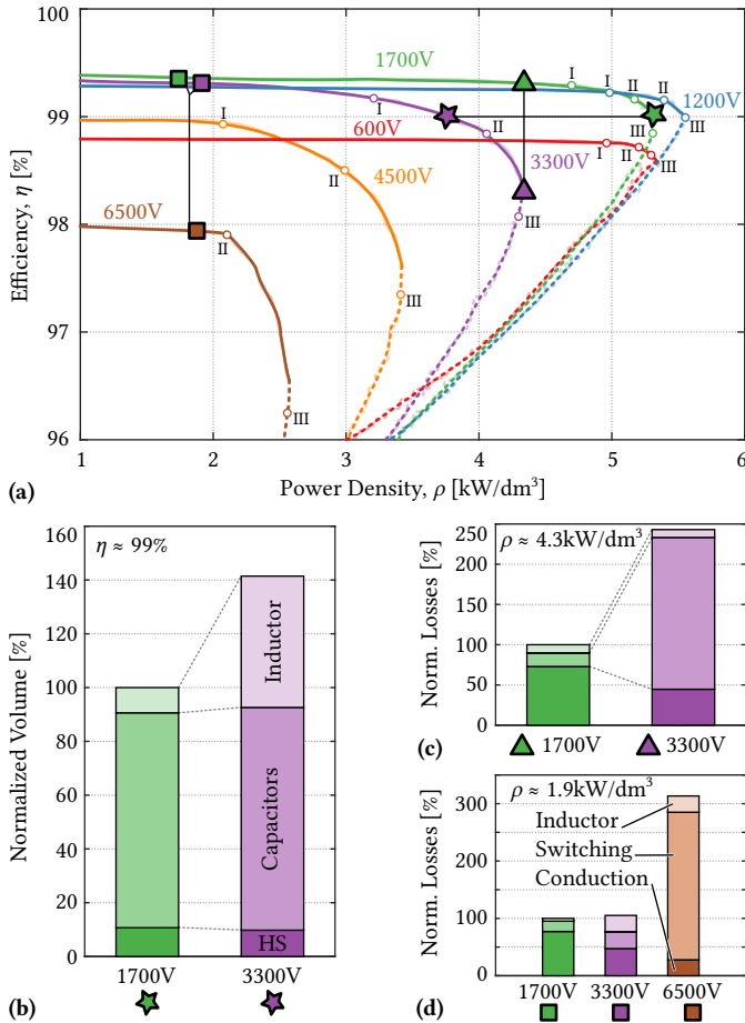
Fig. 2.11: (a) Results of the \eta\rho -Pareto optimization of a 1MVA system (operating in AC-DC rectifier mode with unity power factor) connected to a 10 kV grid, based on virtual IGBT modules with current ratings, I_N , according to Tbl. 2.3 , i. e., with equal total silicon areas for all designs. Approximate device switching frequencies are indicated by I \rightarrow 500 Hz, II \rightarrow 1 kHz, and III \rightarrow 2 kHz; Tbl. 2.4 shows the resulting effective switching frequencies of the multilevel output voltages. In addition, (b) shows the component volume distribution of two designs based on 1700 V and 3300 V IGBTs, respectively, which both feature the same efficiency of \eta = 99\% . Similarly, (c) shows the loss distribution of a 1700 V and a 3300 V design featuring the same power density (the maximum power density achievable with 3.3 kV IGBTs). Finally, (d) shows the loss distribution at a much lower power density, also including a 6.5 kV design.
