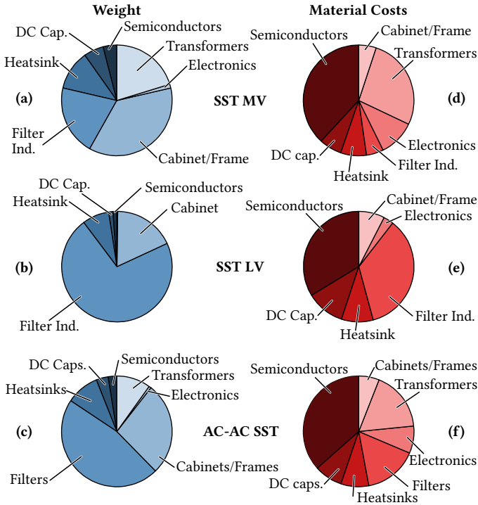
Fig. 4.36: Weight breakdowns of (a) the MV-side converter stage, (b) the LV-side converter stage, and (c) the complete AC-AC SST; material cost breakdowns of (d) the MV-side converter stage, (e) the LV-side converter stage, and (f) the complete AC-AC SST.
