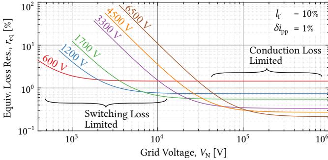
Fig. 2.8: Semiconductor losses expressed as an equivalent loss resistance, r_{eq} , for l_f = 10\% and \delta i_{pp} = 1\% , showing the silicon multilevel limits, i. e., the switching loss limited region and the conduction loss limited region.
