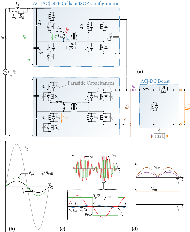
Fig. 5.12: Topology and key waveforms of the Swiss SST (S 3 T), an all-SiC IFE-based SST capable of providing bidirectional power flow with unity power factor at reduced system complexity. Note that no measurements are required on the MV side, and that C_{r1} and C_{r2} , i. e., the capacitors on floating potential, are only small resonant capacitors. Only two cascaded cells of the full system comprising five cells in an ISOP arrangement are shown. Tbl. 5.3 gives the S 3 T’s main specifications.
