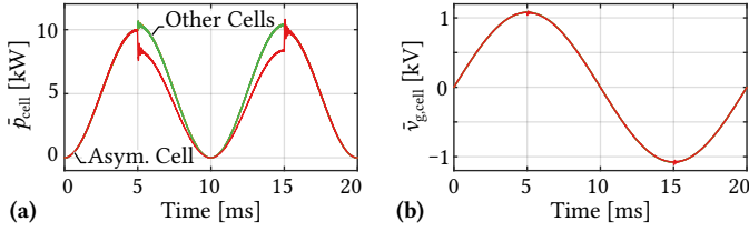
Fig. 5.8: Simulated self-balancing of the cells in ISOP configuration according to Fig. 5.6a and with specifications from Tbl. 5.1 , where the boost converter is modeled as a current source. At t = 5 ms, a disturbance is introduced by connecting a load resistor (10 % nominal cell power) at the MV terminals of one cell. At t = 15 ms, the disturbance is removed again. (a) Power distribution between the cells, and (b) sharing of the input voltage. Note that the waveforms show local average values.
