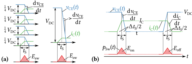
Fig. 2.14: (a) Increase of required dv/dt to obtain equal switching energies in a single-cell system as in a corresponding multi-cell system; (b) simplified modeling of turn-on and turn-off losses for the HV SiC devices.
