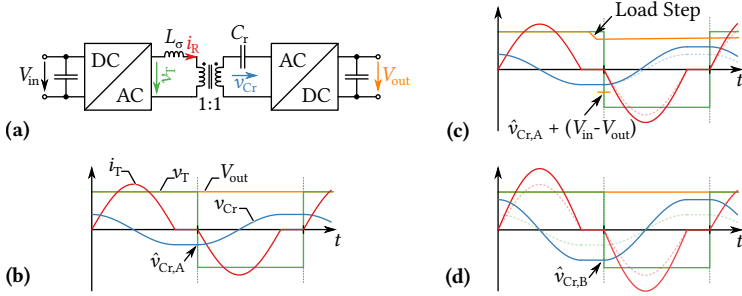
Fig. 3.3: (a) Basic topology of the HC-DCM SRC, (b) idealized waveforms for a steady state A, (c) disturbance of this steady state by a load step that causes a step in the output voltage, and (d) new steady state B corresponding to the increased power flow.
