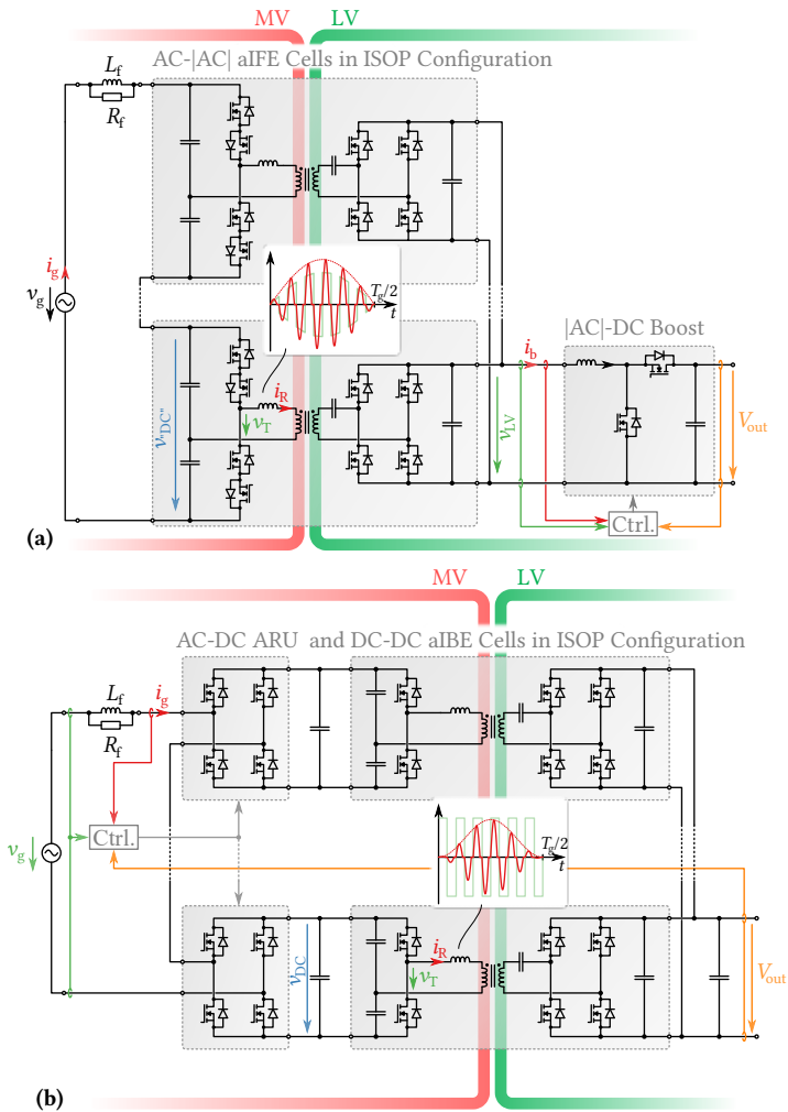
Fig. 6.1: Power circuits of the IFE (a) and the IBE (b) MVAC-LVDC SSTs considered in the comparative evaluation. Note that the number of cascaded cells is different for the two systems (cf. (6.1)), and that the boost stage of the IFE system would be realized in practice from several smaller boost stages using parallel interleaving.
