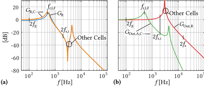
Fig. 4.7: Key transfer functions of the equivalent circuits shown in Fig. 4.6 : G_R = \bar{i}_R/i_{in} , G_{R,C \rightarrow \infty} = G_R but considering C_{inv} \rightarrow \infty , and G_{Out,A,C \rightarrow \infty} = i'_{out}/i_{in} using the same approximation. G_{Out,R} = i'_{out}/i_R , where i_R is the actual, i. e., switched, resonant current. The specifications used to generate the plots are given in Tbl. 3.1 , from which R_{dc} = 59.6 \text{ m}\Omega and L_{dc} = 35 \text{ }\mu\text{H} follow. Furthermore, L'_d = 20 \text{ }\mu\text{H} and R'_d = 1 \text{ m}\Omega are considered. Note that the R'_{dp} = 5 \text{ }\Omega damping is chosen very low in order to highlight the resonances caused by the other cells' DC link assemblies.
