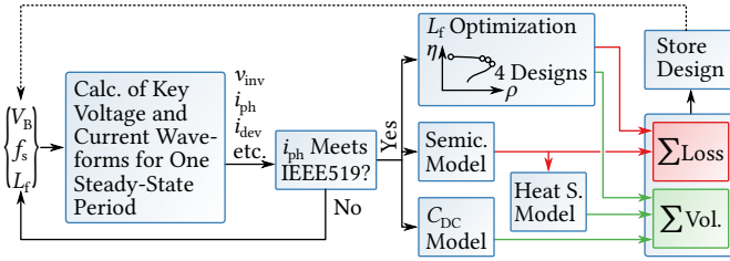
Fig. 2.10: Flowchart illustrating the optimization procedure used to calculate many design points allowing for the \eta\rho -Pareto fronts in Fig. 2.11a to be extracted. The component models and the overall optimization procedure are described in Section 2.3.1.
