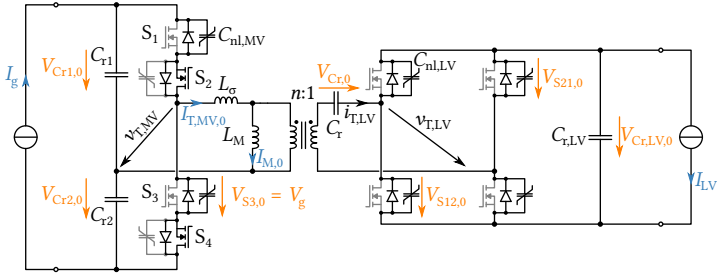
Fig. 5.18: Full aIFE circuit, including non-linear MOSFET capacitances, which is used to simulate the ZVS transitions for given initial conditions. These initial conditions are also highlighted in the figure.
