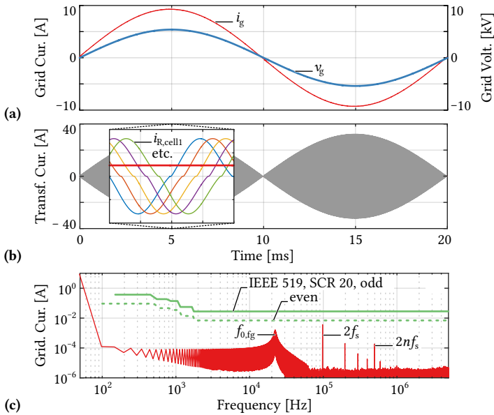
Fig. 5.7: Simulation results of a single-phase ISOP system according to Fig. 5.6a (the boost converter is modeled as a current source) and with specifications given in Tbl. 5.1 . Furthermore, L_g = 690 \mu\text{H} , R_g = 22 \text{ m}\Omega , L_f = 200 \mu\text{H} , and R_f = 10 \Omega are used.
