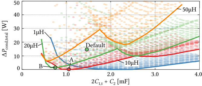
Fig. 4.10: Loss increase vs. capacitance Pareto fronts for four different L_d values with the two designs A and B from Fig. 4.9 indicated.
