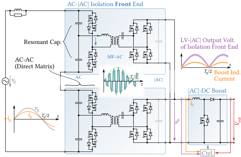
Fig. 1.12: Typical modern IFE topology (cf. Fig. 1.11 ), using also cascaded converter cells and a resonant AC-|AC| isolation stage (cf. also Fig. 1.6b ).
