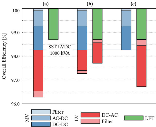
Fig. 4.38: Loss distribution of the three considered application cases, where (a) is for full AC-AC operation, (b) is for 50 % AC-DC and 50 % AC-AC operation, and (c) is for full AC-DC operation. Note that overall system losses at full-load operation, i. e., where AC and DC outputs are loaded with their respective rated power, are considered.
