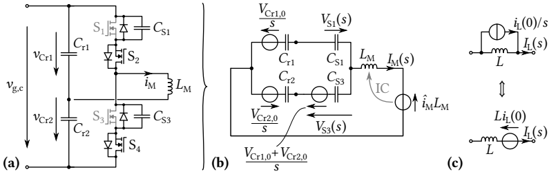
Fig. 5.13: (a) MV-side bridge leg during commutation from S_1 to S_3 and (b) corresponding Laplace equivalent circuit, where the voltage source \hat{i}_M L_M represents the initial condition of the magnetizing inductor current. Note that this circuit is valid for a simplified analysis only, because the parasitic capacitances of the LV-side switches are not yet considered. (c) Two equivalent variants for representing the initial condition of an inductor in the Laplace domain.
