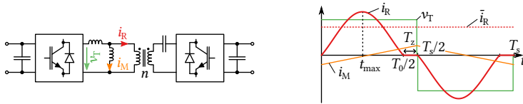
Fig. 3.8: Key waveforms of the HC-DCM SRC, where the local average value, \bar{i}_R , of the resonant current, i_R , is highlighted.
