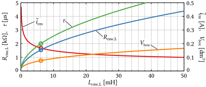
Fig. 4.23: Required damping resistor, R_{\text{cm},L} , resulting time constant, \tau , and RMS common-mode current, i_{\text{cm}} , as functions of L_{\text{cm},L} . The estimated boxed volume of the CMC, V_{\text{box}} , is also shown. The circles indicate the design selected for further evaluation (cf. text).
