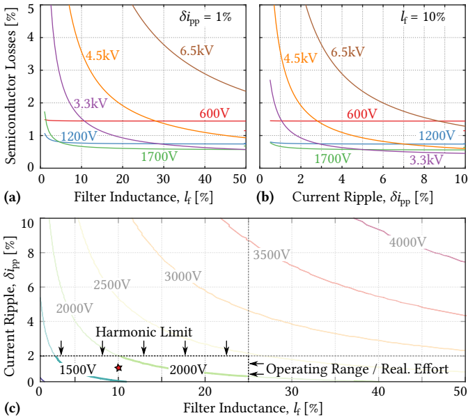
Fig. 2.6: Sensitivity of the semiconductor losses to variations of (a) the filter inductance, l_f , and (b) the allowable grid current ripple, \delta_{i_{pp}} ; (c) corresponding dependence of the optimum blocking voltage on these parameters, where the basic limitations of feasible values are indicated.
