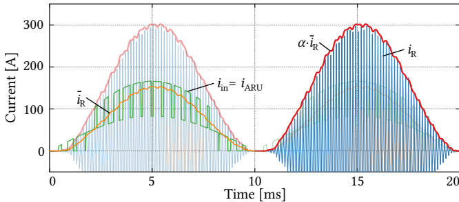
Fig. 4.3: Simulated waveforms of the circuits shown in Fig. 3.9a and c for pure active power transfer from the grid. i_{\text{ARU}} denotes the output current of the cell's ARU stage (cf. Fig. 4.2a), and \alpha = \hat{i}_{\text{R}}/\bar{i}_{\text{R}} as derived in Section 3.2.
