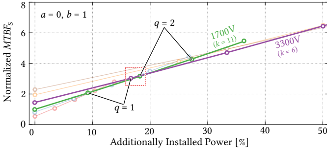
Fig. 2.18: Active redundancy: MTBF_S (normalized to the 1700 V design without redundancy) versus additionally installed power capability, considering only a blocking-voltage dependent failure rate ( a = 0 , b = 1 ).
