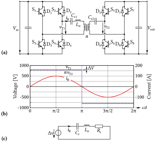
Fig. 3.4: (a) HC-DCM SRC topology; (b) simulated current and voltage waveforms for L_\sigma = 16 \mu\text{H} , C_r = 25 \mu\text{F} , R_r = 130 \text{ m}\Omega , V_{in} = 800 \text{ V} and P_{out} = 50 \text{ kW} ; (c) simplified and primary side referred converter model [133].
