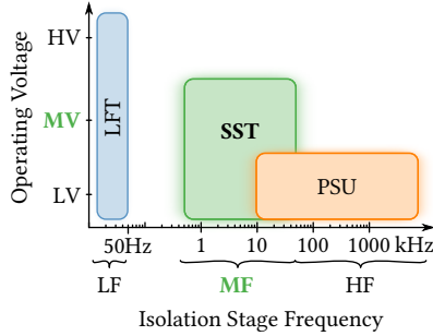
Fig. 1.3: Key characteristics that set an SST apart from a low-frequency transformer (LFT) and from a conventional power supply unit (PSU).
