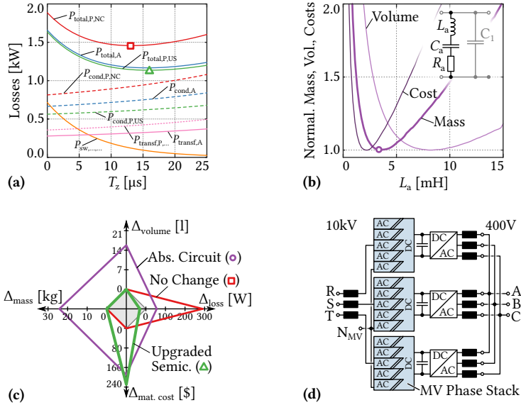
Fig. 4-5: (a) Converter losses for average and pulsating power transfer (cf. Tbl. 3.1 for specifications). Index \dots_A denotes averaged power transfer, index \dots_{P,NC} denotes pulsating power transfer without changed power semiconductors, and index \dots_{P,US} denotes pulsating power transfer with upgraded power semiconductors. (b) Optimization of the absorption circuit. (c) Comparison of the two approaches on the basis of one converter cell; the symbols in parentheses refer to the respective designs in (a) and (b). (d) Overview schematic of a fully phase-modular SST system.
