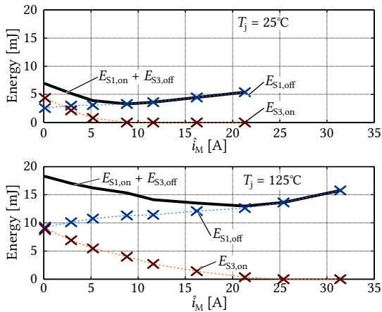
Fig. 3.19: Influence of the magnetizing current peak value, \hat{i}_M , on the turn-off losses in S_1 and the turn-on losses in the complementary switch S_3 .
