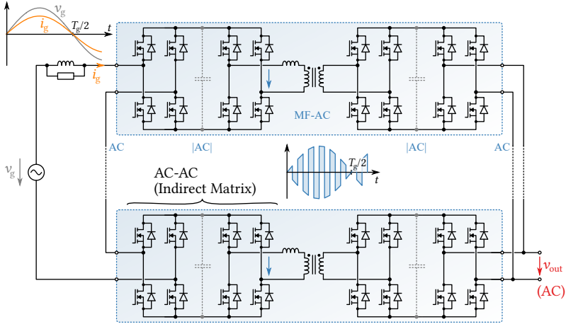
Fig. 1.8: Typical modern matrix-type AC-AC SST topology, which consists of an ISOP arrangement of AC-AC isolation stages as shown in Fig. 1.6 (resonant or non-resonant variants are possible); an industrial prototype employing this topology is shown in Fig. 1.10a .
