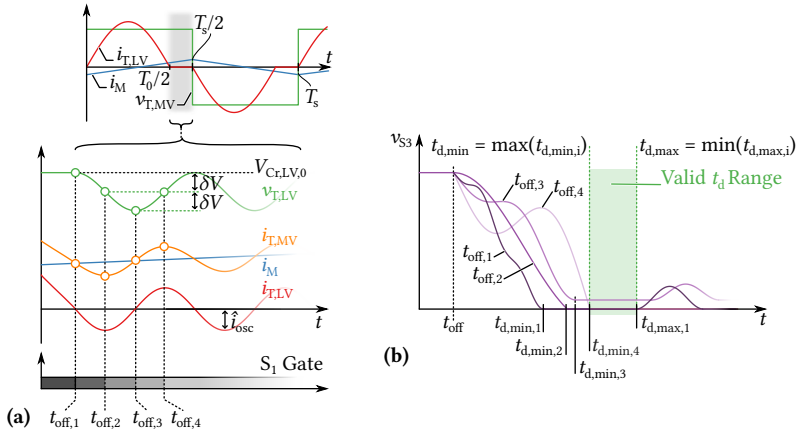
Fig. 5.19: (a) Parasitic HF oscillation during the current zero interval. The actual turn-off instant of S_1 may occur at any time relative to this HF oscillation; four representative cases are indicated as t_{\text{off},\{1,2,3,4\}} , whereby t_{\text{off},1} constitutes the nominal case (the switching occurs at the same instant as the resonant current, i_{T,LLV} becomes zero). (b) Exemplary switching transitions for different initial conditions (e. g., switching at t_{\text{off},1} , t_{\text{off},2} , t_{\text{off},3} or t_{\text{off},4} ). The shapes and durations of the transitions vary, some may not swing to zero completely, and some may start to swing back to positive voltage values at some point. Thus, a dead time t_{d,\min} \leq t_d \leq t_{d,\max} must be chosen if ZVS shall be obtained.
