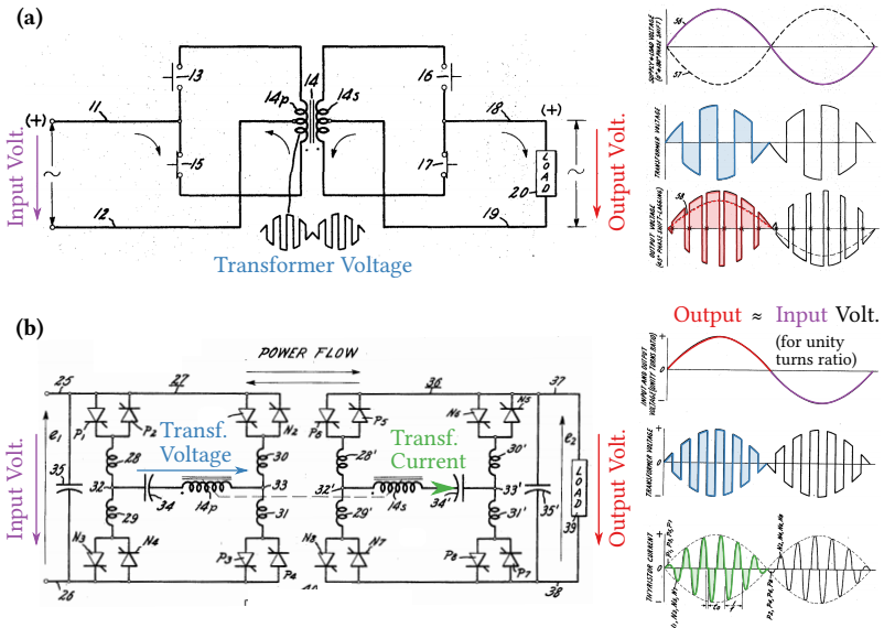
Fig. 1.6: (a) Non-resonant AC-AC power converter with a HF link as proposed in 1968 by McMurray [37], with key converter waveforms illustrating the output voltage regulation by delaying the firing of the secondary side bridge; and (b) resonant variant (also shown in an AC-AC configuration) employing the half-cycle discontinuous conduction mode (HC-DCM), also taken from a patent filed by McMurray in 1968 [38] (colors added by the author).
