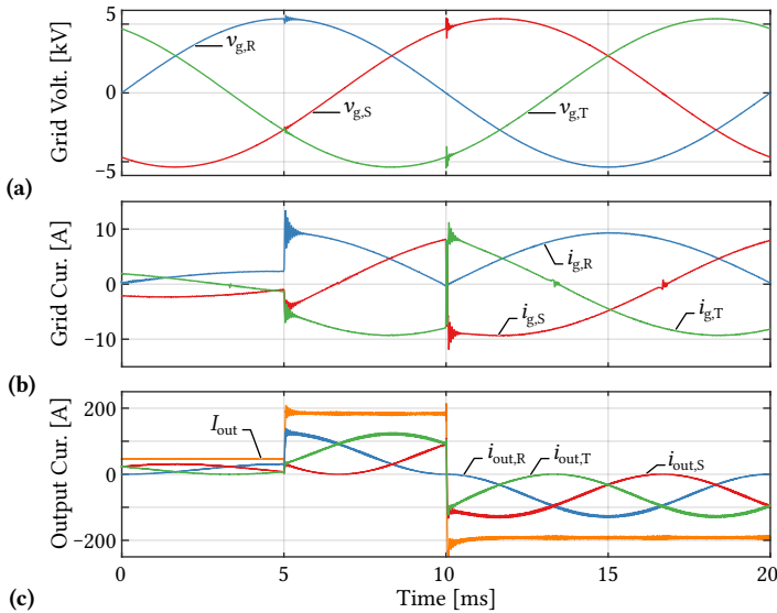
Fig. 5.9: Simulation of a three-phase IFE AC-DC SST system, where three phase stacks according to Fig. 5.6b are connected in star configuration. The currents i_{out,R} , i_{out,T} and i_{out,S} are the DC-side output currents of the three phase stacks; due to the three-phase configuration, the fluctuating power of the three phase stacks adds up to a constant DC-output power and hence constant overall output current, I_{out} . The specifications are given in Tbl. 5.1 , i. e., the three-phase power is 75 kW. Furthermore, L_g = 690 \mu\text{H} , R_g = 22 \text{ m}\Omega , L_f = 200 \mu\text{H} , and R_f = 4 \Omega are used. At t = 5 \text{ ms} , the load current reference changes from 25 % to 100 %, and at t = 10 \text{ ms} , the power flow direction is fully reversed at rated load.
