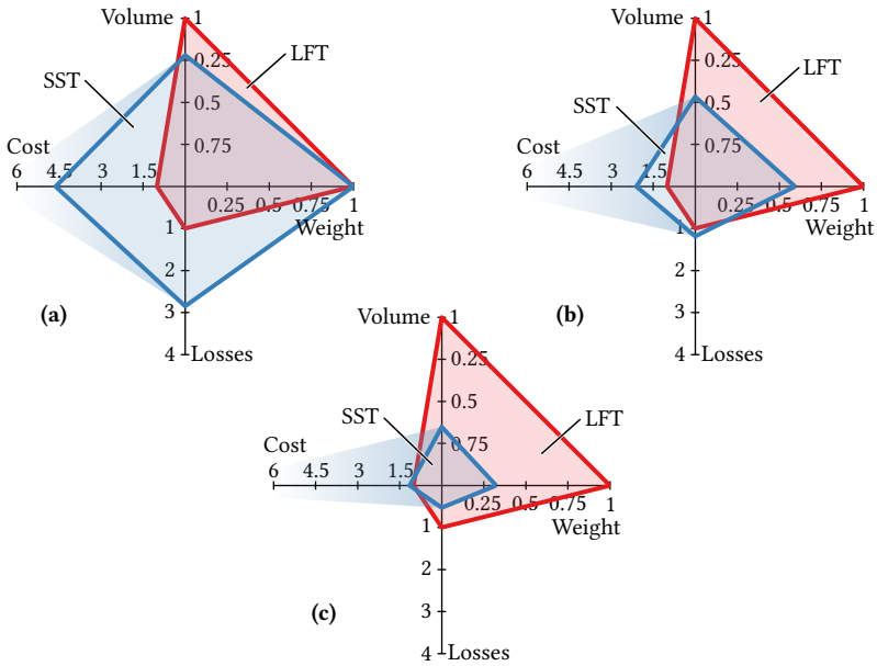
Fig. 4.37: Comparison of LFT and SST performance characteristics, normalized to the LFT-based solutions. (a) for AC-AC operation, (b) for 50 % AC-AC and 50 % AC-DC operation, and (c) for AC-DC operation. Note that the material cost estimates for the SST-based solutions constitute lower bounds only.
