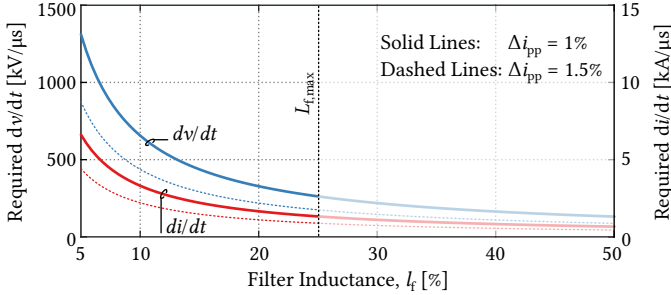
Fig. 2.15: Required dv/dt and di/dt (cf. Fig. 2.14b ) to obtain relative switching losses of 0.5% with a single-cell HV SiC solution as a function of the filter inductance and for two different current ripple limits. L_{f,max} is the maximum allowable inductance value if the pure capacitive operating point must be achievable with rated current and V_{DC,total} = 10.3 kV.
