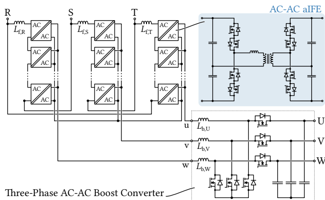
Fig. 5.10: Three-phase IFE SST for AC-AC applications.
