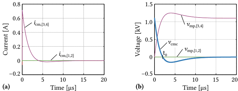
Fig. 4.25: Considering a step transition of v_{B,3} , (a) shows the response of the common-mode currents and (b) shows the corresponding midpoint voltages, where also the voltage across a local CMC, v_{cmc} , is shown. Note that L_{eq} = 100 nH is considered in addition to the designed local CMCs.
