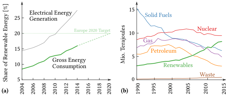
Fig. 1.1: (a) Share of renewables in total energy consumption and electrical energy generation in the EU28 countries (data from [3]). (b) Primary energy production in the EU28 countries (data from [4]).
