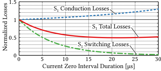
Fig. 3.17: Calculated influence of the zero current interval duration on the semiconductor losses for f_s = 7.5 kHz and T_j = 125 °C. Note that the optimum is shifted to the left and upwards if other losses related to RMS current are included.
