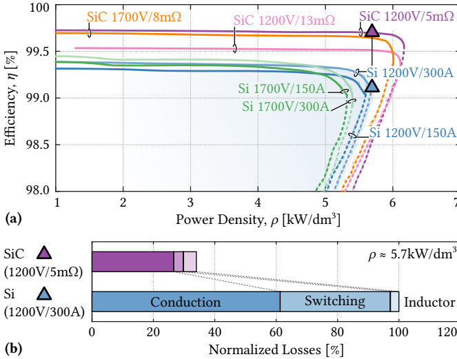
Fig. 2.13: (a) Comparison of Pareto fronts of designs based on Si IGBTs (cf. also Fig. 2.11) and SiC power MOSFET modules; (b) shows the the loss distribution of a SiC and a Si design featuring the same power density (the maximum power density achievable with Si designs).
