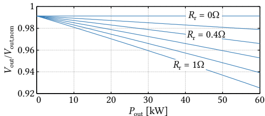
Fig. 3.7: Dependence of the LV-side output voltage on the transferred power and the resistor R_r .
