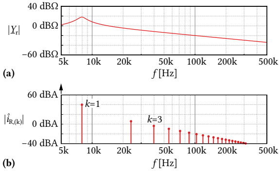
Fig. 3.5: (a) Admittance of the resonant tank ( L_\sigma = 16 \mu\text{H} , C_r = 25 \mu\text{F} , R_r = 130 \text{ m}\Omega ); (b) calculated spectrum of i_R : \hat{i}_{R,(1)} is 34 dB higher than \hat{i}_{R,(3)} . The spectrum shown in (b) corresponds to the current depicted in Fig. 3.4b, which is almost sinusoidal.
