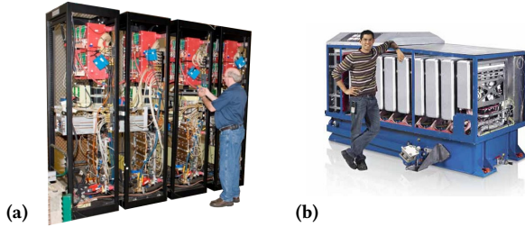
Fig. 1.10: Examples of industrial realizations of SST systems: (a) GE’s all-SiC 1 MVA single-phase “solid-state power substation” (SPSS) prototype featuring a matrix-type AC-AC topology as shown in Fig. 1.8 (photo from [51]), and (b) ABB’s single-phase 1.2 MVA AC-DC “power electronic traction transformer” (PETT) employing an IBE topology as shown in Fig. 1.9 (photo from [53]).
