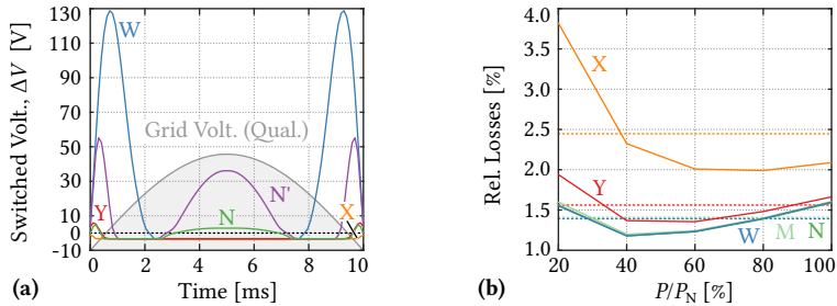
Fig. 5.22: (a) Switched voltage over half a grid period for different designs (W and X are for switching under nominal conditions, i. e., at t_{\text{off},1} ; Y, N and N' consider all four switching conditions, i. e., switching at t_{\text{off},1\dots4} , and thus show the worst-case \Delta V curve that is to be expected in a multi-cell system). (b) Calculated efficiency curves for specific designs. In addition, also the averaged relative losses (as, e. g., shown in Fig. 5.21) are indicated.
