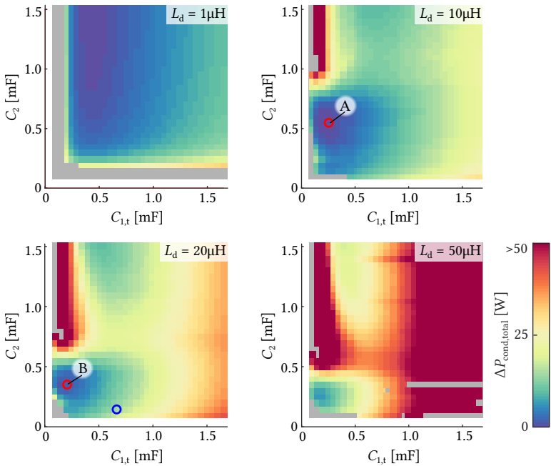
Fig. 4.9: Grid search result overview where the color encodes the overall conduction loss increase, \Delta P_{\text{cond, total}} , with respect to the design with lowest losses.
