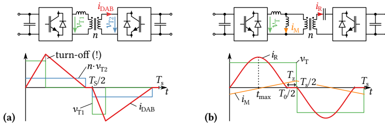
Fig. 3.1: (a) Basic operating principle of a DAB converter with triangular current mode [119, 123]; and (b) as HC-DCM SRC. Note that typically series capacitors need to be placed on both sides of the transformer in order to prevent saturation of the transformer core in case of a (small) DC bias of the bridge output voltage.
