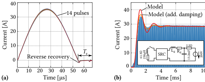
Fig. 3.12: (a) Measured resonant pulses used to determine \alpha and \beta ; (b) measured step response compared with results from the dynamic model.
