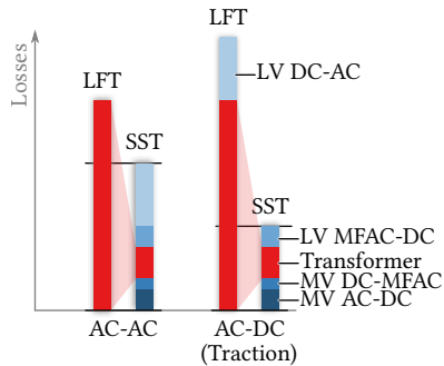
Fig. 7.5: “Efficiency challenge” in a weight/volume restricted environment: The achievable efficiency gain in the transformer itself justifies the additional conversion stages for both, AC-AC and AC-DC (e. g., traction) applications.
