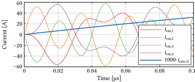
Fig. 4.22: Step responses of the common-mode currents, i_{cm,k} , and the current in the global CMC, i_{cm,G} , for L_{eq} = 100 nH, L_{cm,G} = 10 mH and R_{cm,G} = 10 k \Omega .
