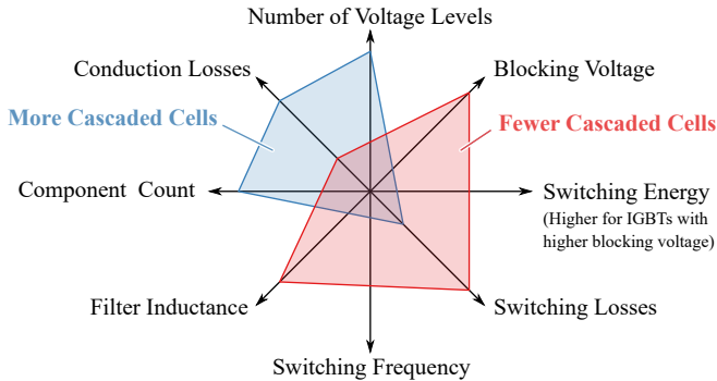
Fig. 2.2: Overview of the trade-offs that are affected by the number of cascaded converter cells.
