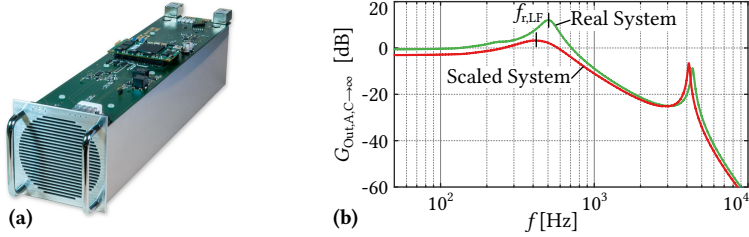
Fig. 4.11: (a) Scaled demonstrator SST cell providing a 100 V “MV” AC input (note that four cells will be cascaded to interface the 400 V grid) and an isolated 800 V LV DC output; (b) comparison of the main transfer function, G_{\text{Out,A,C} \rightarrow \infty} , of the full-scale and the built scaled SST cell.
