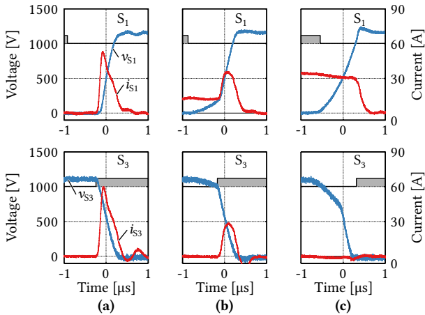
Fig. 3.18: The commutation process changes with increasing magnetizing current from (a) pure ZCS via (b) a mixed form to (c) soft-switching. The measurements were taken with a zero current interval of about 2 \mu\text{s} and an effective interlock time of about t_d = 0.8 \mu\text{s} ; the gate signals are indicated qualitatively.
