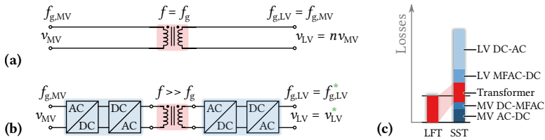
Fig. 7.1: “Efficiency challenge” faced when replacing an LFT (a) with an AC-AC SST (b): the additional conversion stages create losses, whereas the efficiency gain of the transformer itself is only minor (c). Note that for reasons of clarity only a single-phase system is shown; however, the considerations apply equally to a three-phase system.
