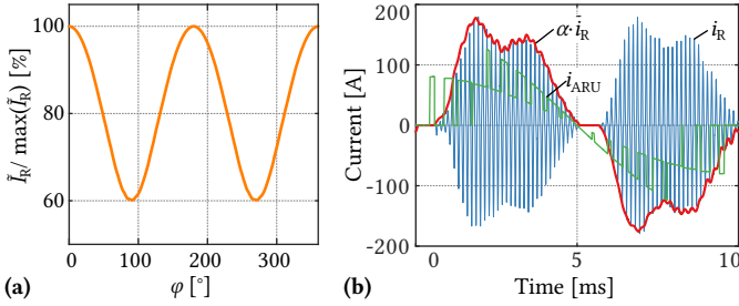
Fig. 4.4: (a) Relative \tilde{I}_R for various grid current phase angles; (b) simulated example for \varphi = 90^\circ (note that \alpha \tilde{I}_R < 0 corresponds to reversed power flow).
