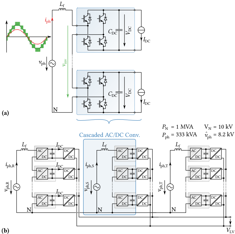
Fig. 2.1: (a) Single-phase CHB converter structure with the DC-side supply/loads modeled as DC current sources (as considered throughout the chapter), including key waveforms, and (b) exemplary application of this CHB structure in a three-phase AC-DC SST.
