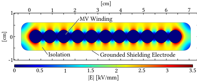
Fig. 4.14: Electrostatic FEM simulation of the transformer MV winding.
