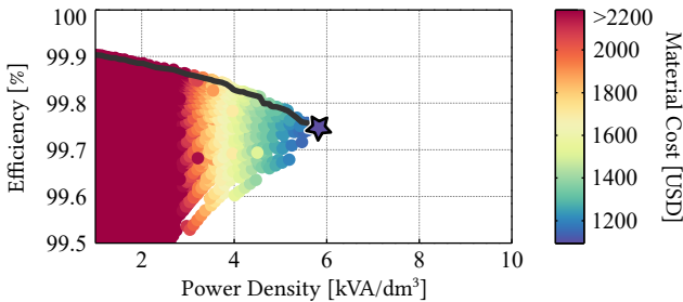
Fig. 4.34: Pareto optimization of the LV-side filter inductors with the chosen design highlighted. Due to the very high currents, the achievable power densities are significantly lower than in the MV case.
