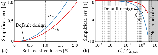
Fig. 3.11: Deviation of the simplified \alpha and \beta (cf. Fig. 3.10b ) from the correct calculation for (a) the influence of damping on the waveform (cf. Fig. 3.10c ), and (b) for the case of small DC capacitors with C_{dc,tot.} := C_1 C_2' / (C_1 + C_2') (cf. Fig. 3.10d ).
