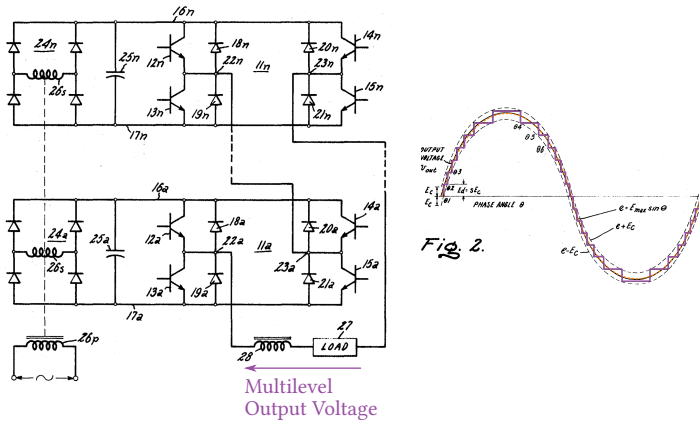
Fig. 1.7: “Fast response stepped-wave switching power converter circuit” patented in 1971 by McMurray [40] (colors added by the author).
