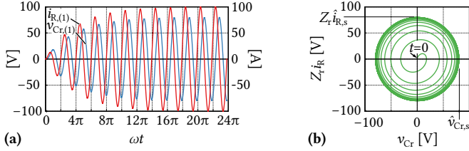
Fig. 3.6: (a) Response of the resonant tank of Fig. 3.4c to a sinusoidal excitation; (b) corresponding phase diagram.
