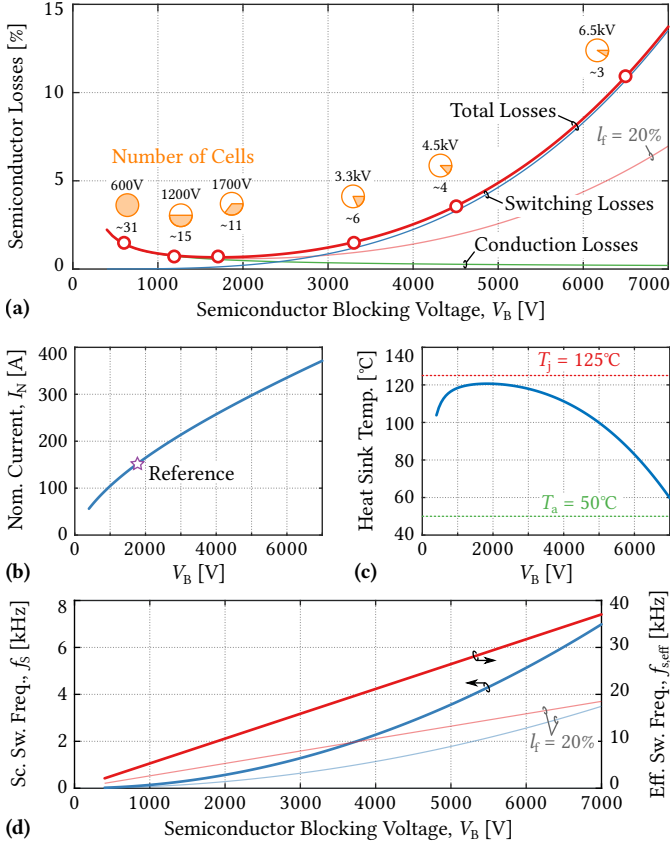
Fig. 2.5: (a) Normalized semiconductor losses as a function of the cells' blocking voltage in a 1 MVA CHB system interfacing a 10 kV grid. The total silicon area is kept constant for all designs, and the required number of cascaded cells is indicated for common IGBT blocking voltages. The main loss curves are for l_f = 10\% and \delta i_{\text{pp}} = 1\% , and additionally the total losses for the case of an increased l_f = 20\% is shown. (b) Nominal device currents for a constant total silicon area as a function of the blocking voltage. (c) Heat sink temperature that is required to dissipate the losses indicated in (a) with T_j = 125^\circ\text{C} . (d) Required switching frequencies per semiconductor and resulting effective switching frequencies of the output multilevel voltage waveforms, f_{s,\text{eff}} = 2 \cdot n_{\text{cell}} \cdot f_s . Note that f_{s,\text{eff}} \propto V_B because f_{s,\text{eff}} \propto n_{\text{cell}} f_s \propto n_{\text{cell}} \cdot 1/n_{\text{cell}}^2 \propto 1/n_{\text{cell}} \propto V_B , as described by (2.18) and (2.11).
