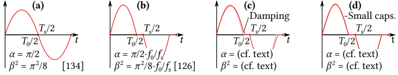
Fig. 3.10: SRC current shapes: (a) pure sinusoidal current; (b) piece-wise sinusoidal current; (c) effect of damping; (d) deviation caused by small DC capacitors.
