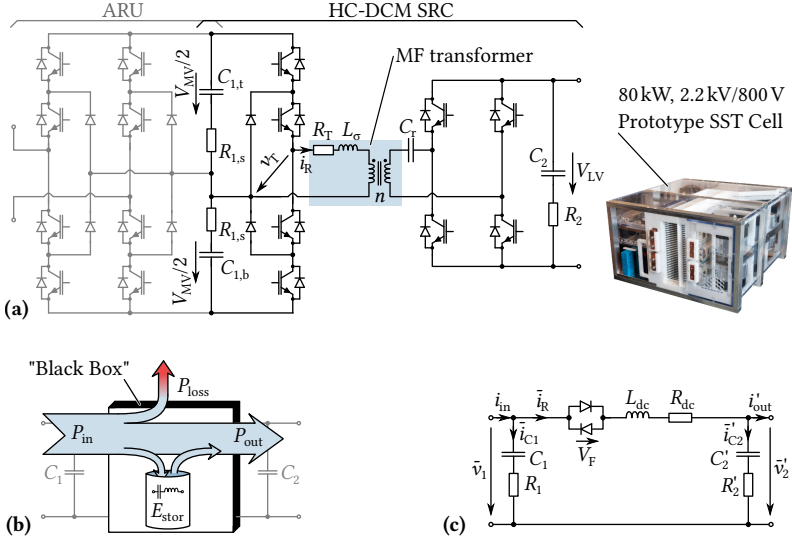
Fig. 3.9: (a) IBE SST cell power circuit consisting of an active rectification unit (ARU) and a HC-DCM SRC, and photo of realized prototype [136]; (b) energy- and loss-based modeling concept visualization; (c) resulting MV-referred dynamic equivalent circuit.
