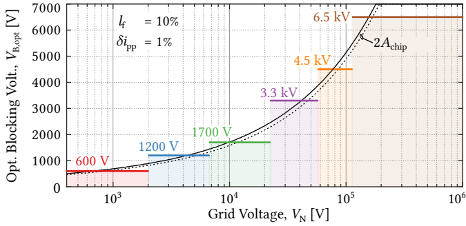
Fig. 2.7: Optimum blocking voltage as a function of the grid voltage (line-to-line); the theoretical curve is overlaid by bars indicating the most suitable IGBT voltage rating. The results consider l_f = 10\% and \delta i_{pp} = 1\% . The optimum blocking voltage is slightly lowered if the available silicon chip area is doubled.
