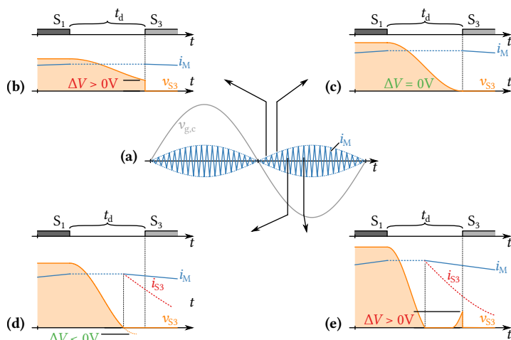
Fig. 5.14: (a) Available magnetizing current over a grid period, and (b-e) exemplary switching transitions with ZVS ( \Delta V \leq 0 V) or partial ZVS ( \Delta V > 0 V).
