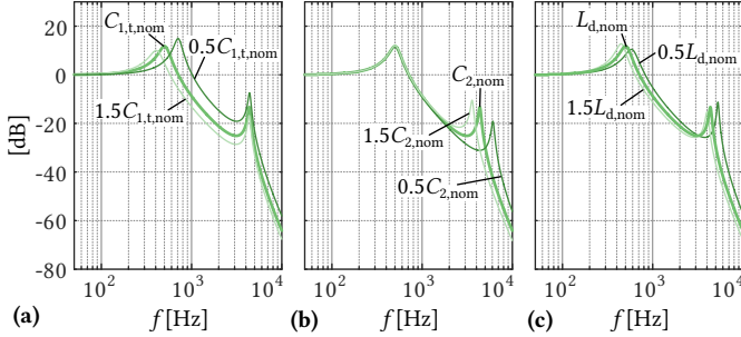
Fig. 4.8: Influence of the main parameters on the transfer function G_{\text{Out,A,C} \rightarrow \infty} : (a) MV capacitor, C_{1,t} ; (b) LV capacitor, C_2 ; and (c) decoupling inductor, L_d .
