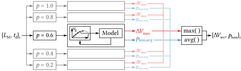
Fig. 5.15: Schematic representation of the ZVS optimization procedure with constant dead time. The optimization routine assigns to each tuple \{L_M, t_d\}_i a tuple \{\Delta V_{wc}, p_{loss}\}_i , i. e., a worst-case \Delta V_{wc} and averaged relative losses, p_{loss} . Please refer to the text for a more detailed description.
