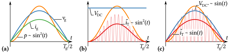
Fig. 6.2: Power transfer in (a) a single-phase grid, (b) in an IBE, and (c) in an IFE system.
