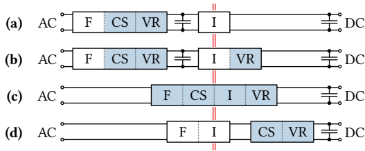
Fig. 5.1: Partitioning and sequencing of the tasks required to perform isolated AC-DC conversion and PFC: Folding (F), current shaping (CS), isolation (I), and output voltage regulation (VR). A shaded background indicates a controllable stage.
