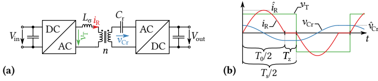
Fig. 3.2: Basic topology (a) and key waveforms (b) of the HC-DCM SRC.
