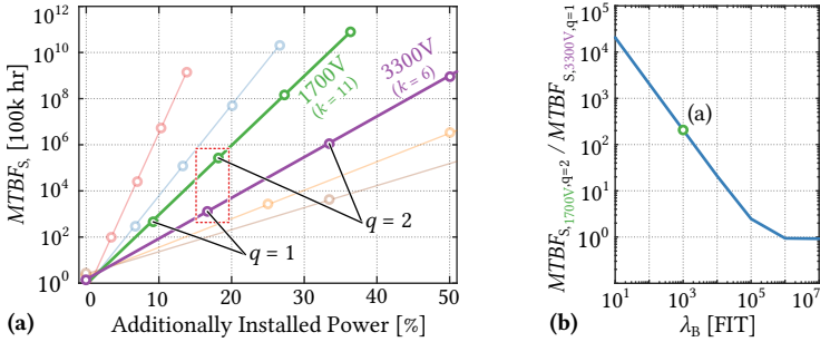
Fig. 2.19: (a) System-level (one phase stack) MTBF_S versus additionally installed power capability considering a repairable system with standby redundancy ( \lambda_B = 1000 FIT, \mu = 1/(7 \cdot 24 h), a = 0.5 , b = 0.5 ) and (b) impact of the base failure rate, \lambda_B , on the ratio between the MTBF_S values of a 1700 V design with q = 2 and a 3300 V design with q = 1 .
