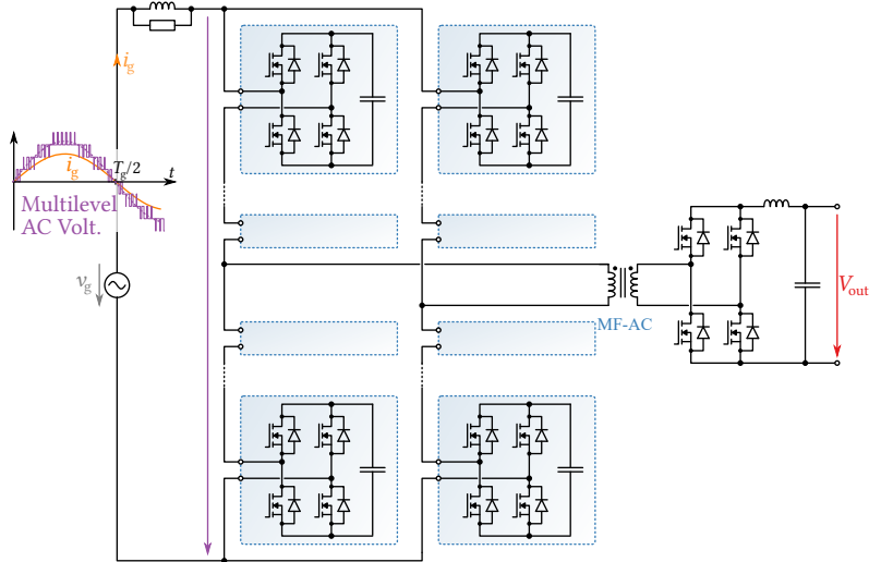
Fig. 1.13: Modular multilevel converter (M2LC) based SST topology [61]. There is only a single transformer, i. e., the modularity is limited to the power electronics.
