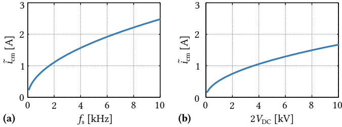
Fig. 4.16: (a) Dependence of the total RMS common-mode current, \tilde{i}_{\text{cm}} , on the cells' switching frequency, f_s , at V_{\text{DC}} = 1.1 \text{ kV} , and (b) on the cells' DC link voltage, V_{\text{DC}} , at f_s = 1 \text{ kHz} .
