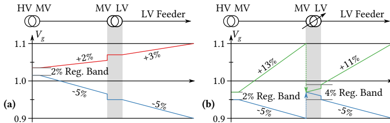
Fig. 7.3: (a) Voltage band usage in a conventional distribution grid and (b) improvement if a voltage regulation transformer is employed at the MV-LV interface. The example data is taken from [217].
