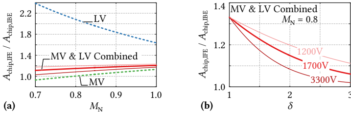
Fig. 6.3: Ratio of the chip area requirements of IFE and IBE systems as a function of the nominal modulation index, M_N , in (a), and in (b) as a function of \delta in r_{\text{on}} \propto V_B^\delta for M_N = 0.8 . For the combined metric, u = 0.66 , f_s = f_0 , V_{\text{out}} = 400 \text{ V} is assumed, and three different MV semiconductor blocking voltages are considered. Note that the three curves in (b) intersect for \delta = 1 , i. e., for r_{\text{on}} \propto V_B , where hence the MV-side conduction losses do not depend on the chosen blocking voltage for a given total chip area.
