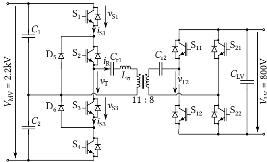
Fig. 3.13: HC-DCM SRC topology considered for the \eta\rho -Pareto analysis.
