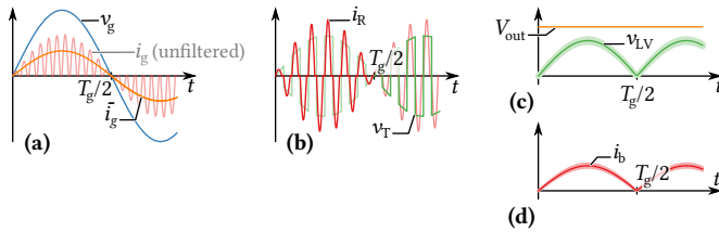
Fig. 5.4: Key waveforms (simplified) of the IFE topology shown in Fig. 5.3b , where a very low switching frequency is assumed for illustration purposes.
