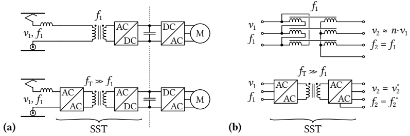
Fig. 1.5: Replacement of an LFT by an SST in (a) a traction application in order to comply with weight and space constraints, and (b) in a distribution grid application, which is motivated by increased functionality such as, e. g., output voltage control or reactive power compensation. Note that v_1 is in the MV range, f_T is in the MF range, and f_2^* includes also the possibility of a DC output ( f_2^* = 0 Hz).
