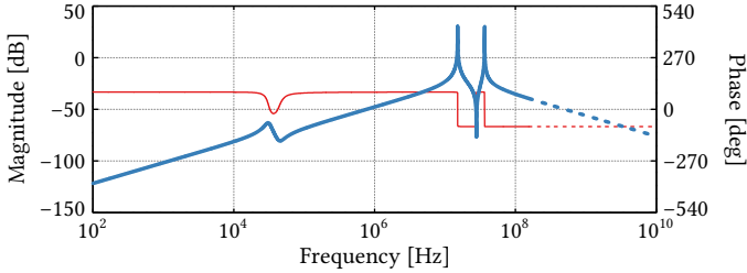
Fig. 4.21: Bode plot of the transfer function G_3(s) for L_{eq} = 100 nH, a global common-mode inductance of L_{cm,G} = 10 mH and a parallel damping resistor of R_{cm,G} = 10 k \Omega .
