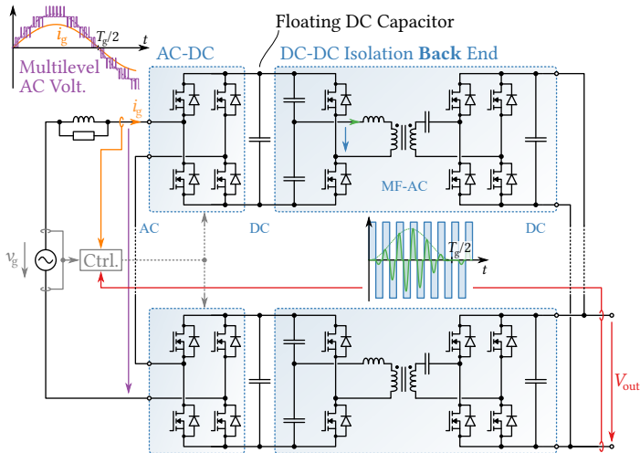
Fig. 1.9: Typical modern Isolated Back End (IBE) topology, realizing a multilevel AC input voltage by means of cascaded H-bridges (cf. Fig. 1.7) and employing a resonant DC-DC isolation stage (cf. Fig. 1.6b); an industrial prototype is shown in Fig. 1.10b.
