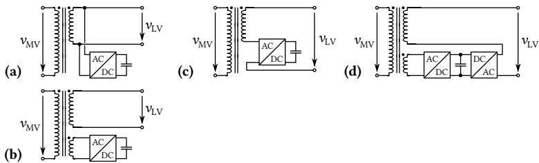
Fig. 7.4: Different realization options of hybrid SSTs as described in [221]. In all cases, the power electronic converters are only rated at a fraction of the total power.
