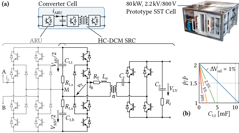
Fig. 4.2: (a) Topology of the converter cell of the considered IBE SST shown in Fig. 4.1 and photo of realized prototype [136]; (b) trade-off between MV-side capacitance and ripple of the power processed by the DC-DC converter; \Delta V_{rel} denotes the relative peak-to-peak MV DC voltage ripple ( C_{1,t} = C_{1,b} ).
