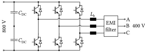
Fig. 4.33: Power circuit of the LV inverter stage.
