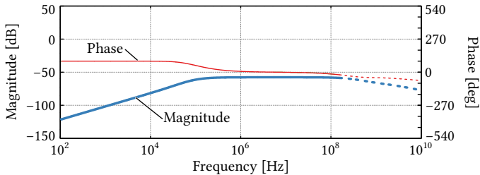
Fig. 4.24: Bode diagram of G_3(s) considering the designed local CMCs (cf. Fig. 4.23) and L_{eq} = 100 nH.
