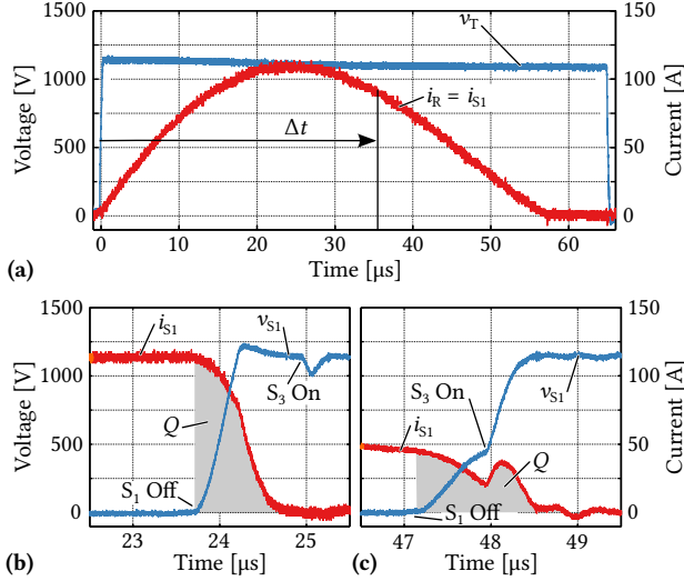
Fig. 3.15: (a) Positive current pulse where the current through S_1 equals the current i_R for L_\sigma = 7.6 \mu\text{H} and C_r = 43 \mu\text{F} , resulting in f_0 \approx 8.8 \text{ kHz} . The turn-off time is defined by \Delta t and varied to measure the extracted charge at different points of the current waveform. Definition of the charge extracted from S_1 for (b) \Delta t = 24 \mu\text{s} and (c) \Delta t = 48 \mu\text{s} .
