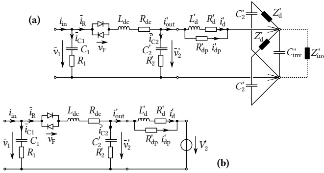
Fig. 4.6: Equivalent circuits of an SST cell, with (a) including a model of the LV-side DC bus assembly including the other converter cells, and (b) with simplification C_{inv} \rightarrow \infty . Z'_{inv} in (a) represents the input impedance of the LV-side DC-AC inverter, which is, however, not considered here.
