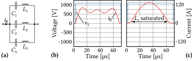
Fig. 3.20: (a) Extended resonant tank where branch 1 is tuned to f_0 = 7.5 kHz, branch 2 to 3f_0 and branch 3 to 5f_0 and (b) resulting current waveform. (c) shows the current shape when a saturable inductor is connected in series to the normal LC resonant tank instead.
