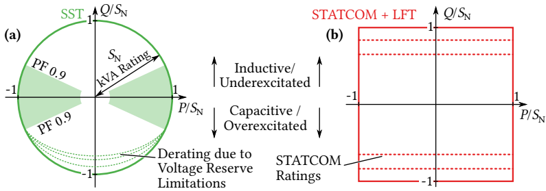
Fig. 7.2: Operating range in the PQ -plane for (a) an SST and (b) for a combination of an LFT and a dedicated STATCOM (the small voltage drop caused by the LFT's inner impedance is neglected).
