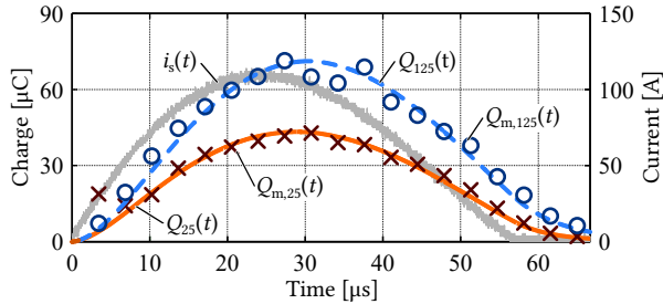
Fig. 3.16: Behavior of the stored charge for the IGBT Infineon FF150R17KE4 at T_j = 25^\circ\text{C} and T_j = 125^\circ\text{C} . Q_{m,25}(t) , Q_{m,125}(t) are measurements and Q_{25}(t) , Q_{125}(t) are obtained with (3.30) and k_s , \tau as given in Tbl. 3.4 .
