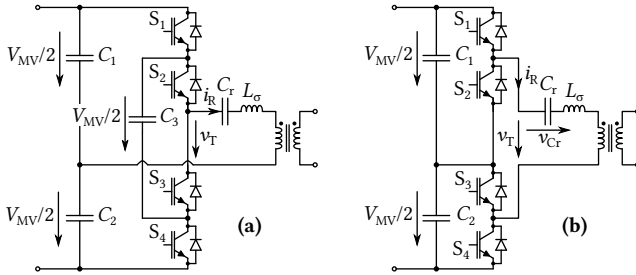
Fig. 3.14: Other realization options for the MV-side bridge that allow for using 1.7 kV IGBTs for V_{MV} = 2.2 kV; (a) adds a flying capacitor while (b) uses a DC offset of V_{MV}/2 on the resonant capacitor [140].
