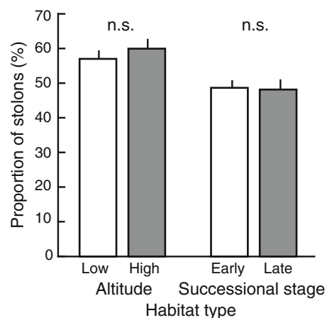
Fig. 2 Frequency (mean \pm SE) of clonal reproduction in plants of Geum reptans from five populations, each from low and high altitude, and from early and late successional habitats (in total 900 plants). The difference between populations of low + high altitude versus early + late succession is significant (a priori contrast, P < 0.05 , from Weppeler and Stöcklin 2005)
