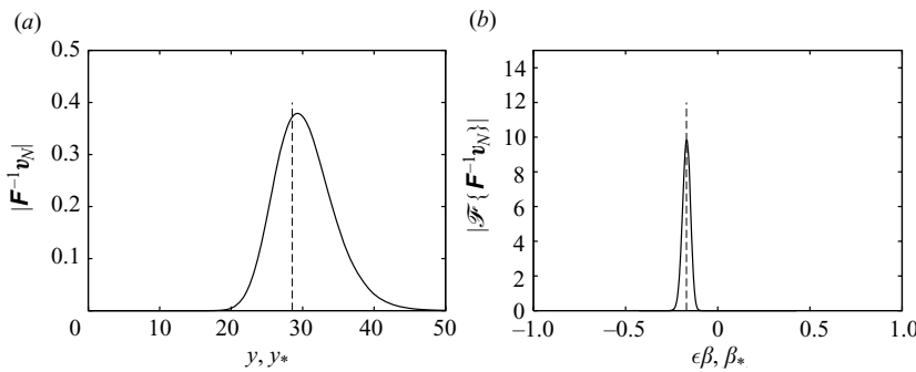
FIGURE 10. (a) Absolute value and (b) Fourier spectrum of the algebraically decaying mode for \lambda = (1.5 - 0.1i)\gamma together with the values y_* and \beta_* from the - branch (broken lines) for which \lambda = f(y_*, \beta_*) .
