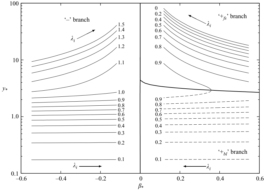
FIGURE 9. Ranges of \{y_*, \beta_*\} for which the twist condition is satisfied ( +_{fs} and - branches) or is not satisfied ( +_{bl} branch). The thin lines are curves for \lambda_r = \text{const.} and \lambda_i/\gamma ranging from -1 to -0.05 (the value of \lambda_r/\gamma is indicated next to the curves; \gamma = 0.3, R = 1000 ).
