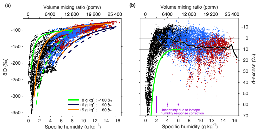
Figure 6. Scatter diagrams of (a) \delta D (‰) and (b) d-excess (‰) versus specific humidity q ( \text{g kg}^{-1} ). Shown are 30 s averaged data from all valid flights. Data points acquired below 500 (1700) m a.s.l. are marked in red (blue). Coloured curves in (a) represent idealized mixing (solid lines) and Rayleigh fractionation processes (dashed lines) as described in the main text. Upper x axis gives water concentration in units of parts per million by volume for easier comparison with other published studies. Green line in (b) represents d-excess from a Rayleigh fractionation process. Black line in (b) is a bin average. Purple points with error bars show the uncertainty resulting from the isotope–humidity response correction at different humidity levels. Note that the d-excess axis in (b) is inverted for display purposes.
