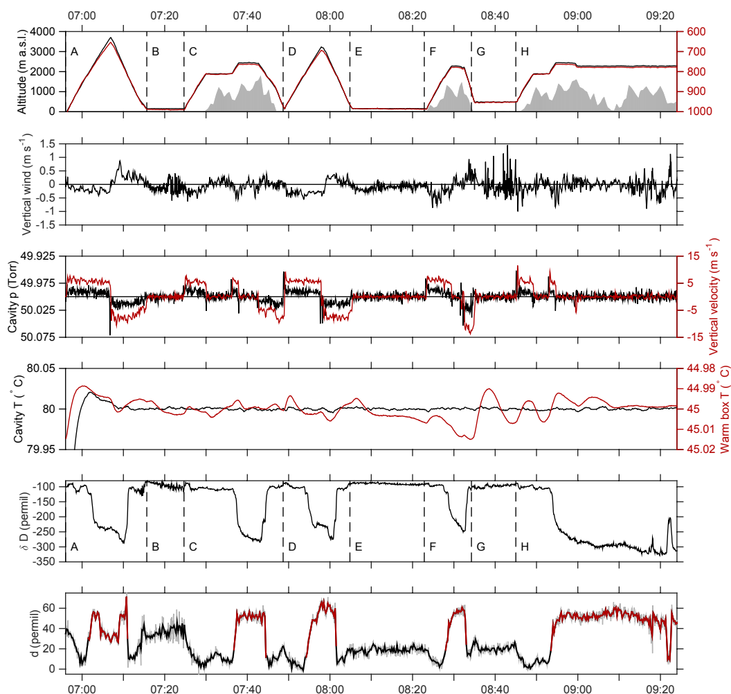
Figure A6. Instrument control parameters during segments A–H of flight 10 on 21 September 2012, 07:00–09:25 UTC. (a) Flight altitude (m a.s.l.; black), cabin pressure (hPa; red) and topography (m; grey shading); (b) vertical wind ( \text{m s}^{-1} ); (c) CRDS cavity pressure (Torr; black) and vertical aircraft velocity ( \text{m s}^{-1} ; red); (d) CRDS cavity temperature ( ^{\circ}\text{C} ; black) and CRDS warm-box temperature ( ^{\circ}\text{C} ; red); (e) \delta\text{D} (black line; ‰) at 15 s averaging time; (f) d-excess (‰) at 15 s averaging time (grey line) and 30 s averaging time (black line). Sections highlighted in red are for specific humidity below 2 \text{ g kg}^{-1} .
