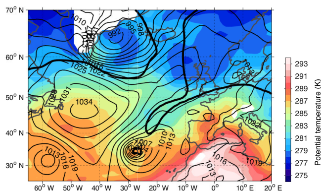
Figure 7. Weather situation at 12:00 UTC, 21 September 2012 (flights 09–11). Shown are sea level pressure (black lines, 3 hPa contour interval), equivalent potential temperature at 850 hPa (colour shading, 1 K interval), and the tropopause structure depicted by a contour of two potential vorticity units on the 315 K isentrope (thick black line) from ECMWF analysis data.
