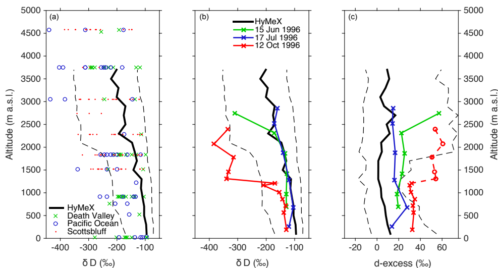
Figure 5. (a) Comparison of HyMeX measurements of \delta D (mean and range, black lines) to airborne \delta D data by Ehhalt (1974) and Ehhalt et al. (2005) from repeated flights over Death Valley, California (green crosses), the Pacific Ocean off the coast of California (blue circles), and Scottsbluff, Nebraska (red dots). (b) Comparison of HyMeX measurements of \delta D and (c) d-excess (mean and range, black lines) to flight measurements by He and Smith (1999) over New England forests on 15 June 1996 (green), 17 July 1996 (blue), and 12 October 1996 (red). Red circles and dashed lines denote data points for which He and Smith (1999) estimated the d-excess from all other measurements due to low-humidity conditions.
