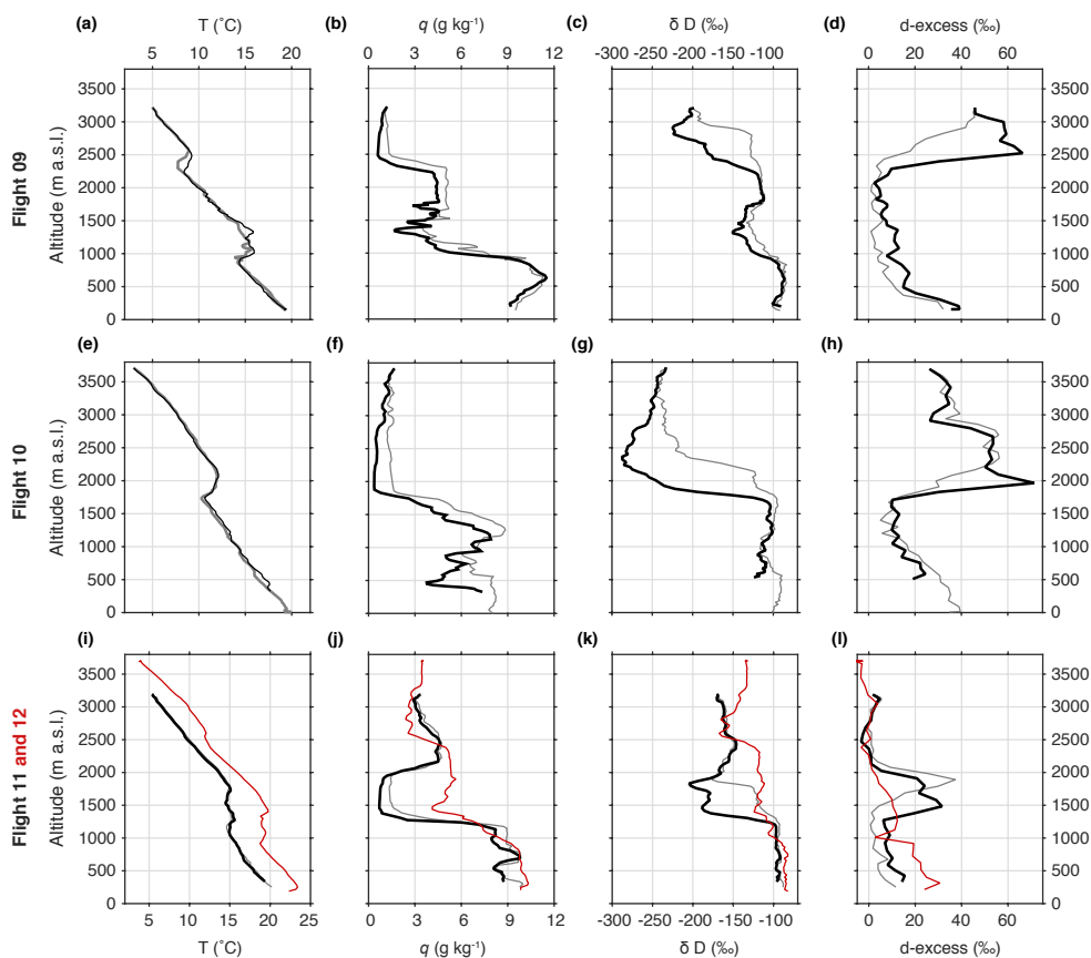
Figure 9. Vertical profiles of air temperature ( T , °C; first column), specific humidity ( q , \text{g kg}^{-1} ; second column), \delta D (‰; third column), and the d -excess (‰; fourth column) for flights 09–12 conducted during 21–23 September 2012. Only downward profiles are shown as they are less affected by memory than upward profiles. Red lines in panels (i) to (l) show the downward profile acquired during flight 12.
