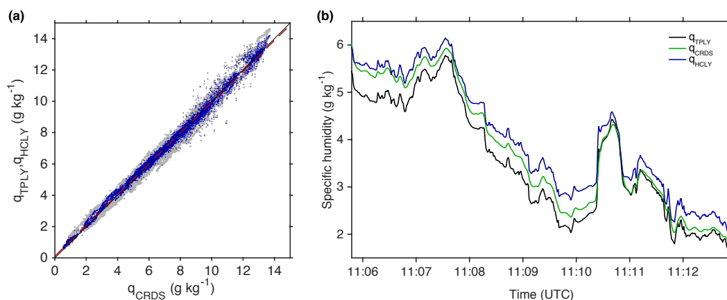
Figure 2. (a) Correlation between calibrated specific humidity from the CRDS ( q_{\text{CRDS}} ), the Humicap–Lyman- \alpha ( q_{\text{HCLY}} , blue dots, \rho = 0.994 ), and the dew point hygrometer–Lyman- \alpha product ( q_{\text{TPLY}} ; grey dots; \rho = 0.989 ) at 1 s time interval for flight 01 on 11 September 2012. Red dashed line shows a linear least-squares fit to the q_{\text{HCLY}} and q_{\text{CRDS}} data; black line is a 1 : 1 relation. (b) Comparison of calibrated humidity measurements from the three products for a representative vertical profile during flight 01 ascending from 1500 m to 3700 m a.s.l.
