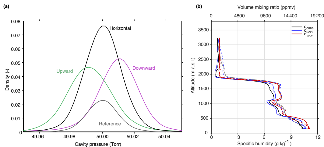
Figure A5. (a) Distributions of cavity pressure for flights 01–14 and 28–32 in purple for vertical velocities < 2 \text{ m s}^{-1} (downward), in green for vertical velocities > 2 \text{ m s}^{-1} (upward), and in black for horizontal legs with vertical velocities 2 \leq v \leq 2 \text{ m s}^{-1} . The distribution of the cavity pressure during a stability experiment (Allan test) in the hangar during the campaign (6 Oct 2012, 10:00–14:00 UTC) is shown in grey as a reference for stable measurement conditions. (b) Vertical profile of specific humidity during flight 10. Upward (dashed lines) and downward (solid lines) from three humidity products CRDS (black), HCLY (blue), and TPLY (red) are shown.
