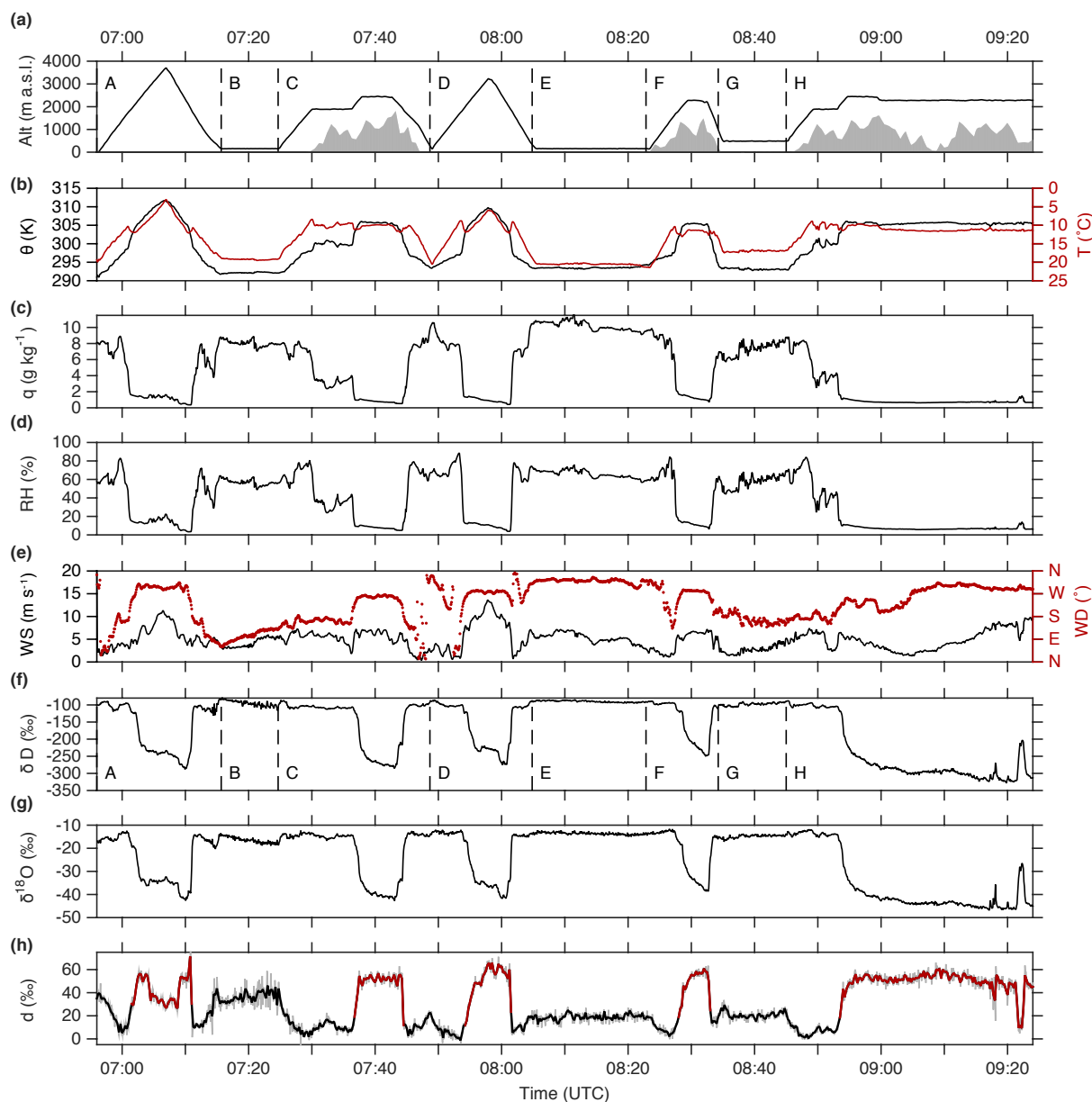
Figure 10. Segments A to H of flight 10 on 21 September 2012, 07:00–09:25 UTC. (a) Flight altitude (black line) and topography (grey shading), (b) potential temperature (K; black) and air temperature ( ^{\circ}\text{C} ; red), (c) specific humidity from CRDS ( \text{g kg}^{-1} ; black), (d) relative humidity from HCLY temperature and humidity (%; black), (e) wind speed ( \text{m s}^{-1} ; black) and wind direction ( ^{\circ} ; red), (f) \delta\text{D} (‰; black) at 15 s averaging time, (g) \delta^{18}\text{O} (‰; black) at 15 s averaging time, (h) d-excess (‰) at 15 s averaging time (grey) and 30 s averaging time (black). Sections highlighted in red are for specific humidity below 2 \text{ g kg}^{-1} . Labels A–H denote different sections of the flight pattern.
