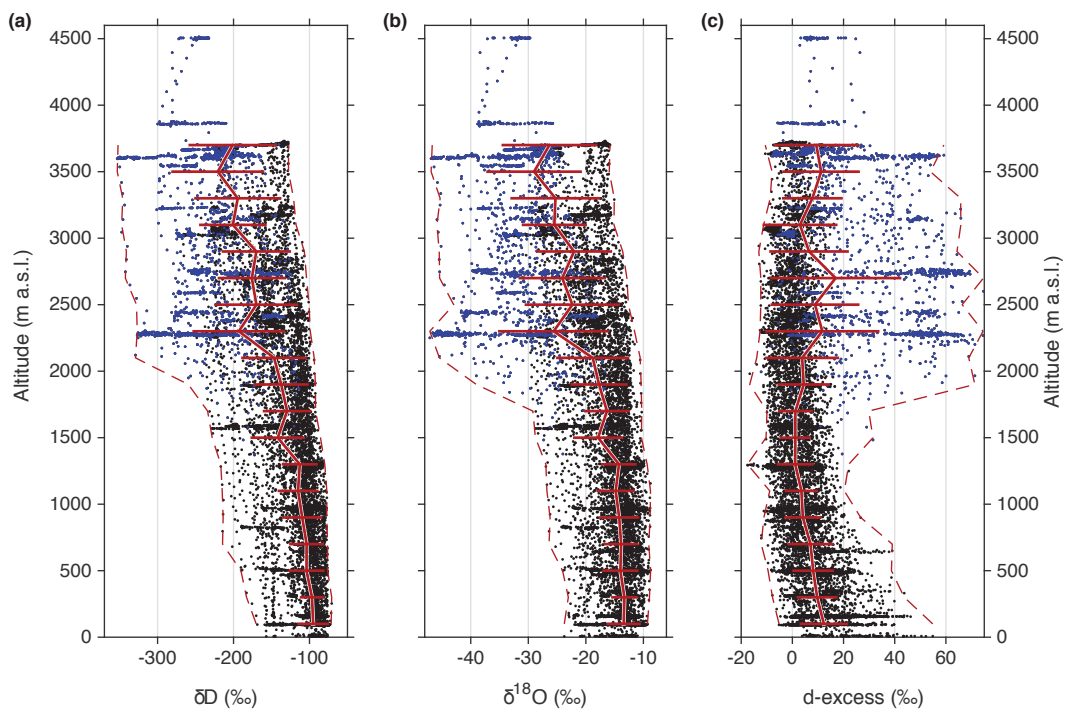
Figure 4. Vertical profiles of the isotopic composition of ambient water vapour for all valid flight data acquired during the campaign. Overlaid are 200 m binned mean (red solid line) and 200 m binned minimum and maximum values (dashed red lines) of (a) \delta D , (b) \delta^{18}O , and (c) d-excess. Data points with a specific humidity below 2 \text{ g kg}^{-1} are shown in blue. Bin averages do not extend above 3700 m because of low data coverage.
