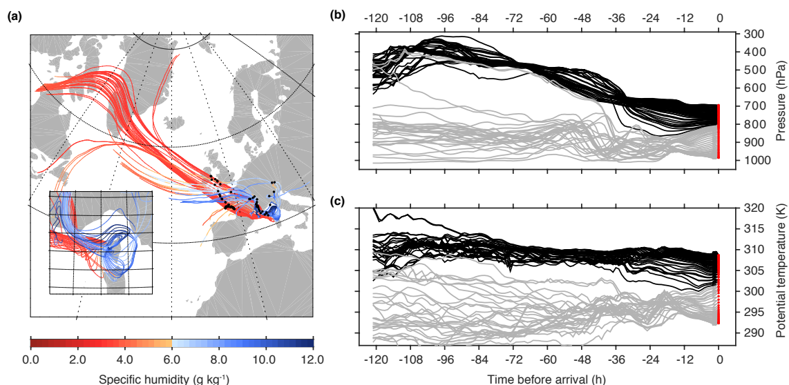
Figure 11. Backward trajectories for the downward leg of the second profile in segment D during flight 10 (21 September 2012, 07:54–08:06 UTC). (a) Five-day trajectories coloured with specific humidity ( \text{g kg}^{-1} ), with small inset showing a zoom around Corsica. Black dots indicate trajectory locations 48h before measurement time. (b) Pressure in hectopascal and (c) potential temperature in kelvin along 5-day trajectories vs. time before measurement. Trajectories arriving with a humidity of less than 2 \text{ g kg}^{-1} are shown in black, all others in grey. Time of aircraft encounter in panel (b) and (c) is marked by red dots.
