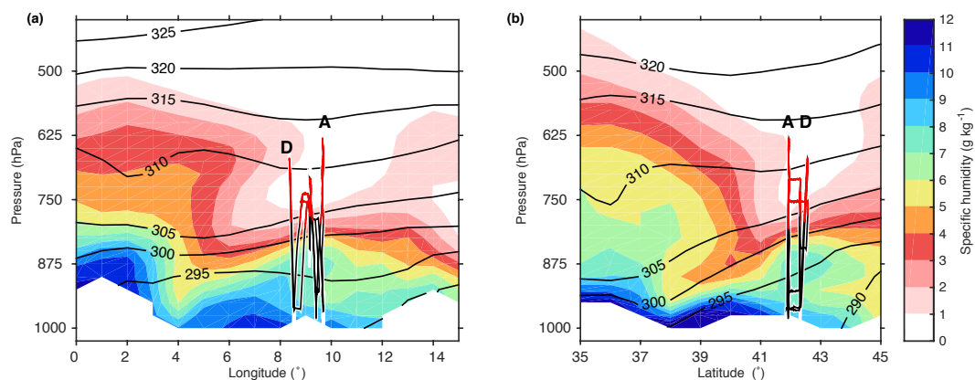
Figure 12. Vertical sections across Corsica during flight 10 (06:00 UTC, 21 September 2012): (a) from 0 to 15^\circ \text{ E} at 42^\circ \text{ N} and (b) from 35 to 45^\circ \text{ N} at 9^\circ \text{ E} . Panels show specific humidity ( \text{g kg}^{-1} , shading), and potential temperature (K, black contours) from ECMWF operational analyses. The flight track for flight 10 is overlaid as a black line, with segments of specific humidity below 2 \text{ g kg}^{-1} plotted in red. A and D correspond to the segments in Fig. 10.
