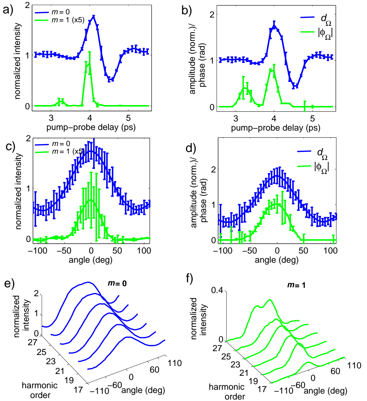
FIG. 2: a) Evolution of the normalized intensities of H19 in the zero order and the first-order diffraction side band with pump-probe delay, measured in N_2 . b) Reconstructed relative amplitude and phase of H19, referenced to an isotropically aligned sample. c) Undiffracted ( m = 0 ) and diffracted ( m = 1 ) intensities of the high-harmonic emission as a function of the alignment angle measured at a pump-probe delay of 4.1ps. d) Reconstructed relative high-harmonic amplitudes and phases as a function of the alignment angle. e,f) Evolution of the normalized intensities of harmonics 17 to 27 in the zero order (e) and the first-order (f) diffraction side band with alignment angle, measured at \Delta t = 4.1 ps.
