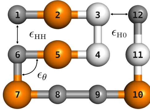
Figure 2. A schematic example of a semi-flexible HOP model. The interaction between monomers 1 and 6 is \epsilon_{\text{HH}} , and that between monomers 3 and 12 is \epsilon_{\text{HO}} . The angle constituted by monomers 5, 6 and 7 contributes \epsilon_{\theta} energy. In this particular 2-dimensional structure, n_{\text{HH}} = 1 , n_{\text{HO}} = 2 and n_{\theta} = 5 . Hydrophobic and “neutral” monomers are colored dark gray and white, respectively, while polar monomers are colored orange. An HP model results if no 0-mers are present and the angle energy is zero. Both models are actually simulated in three dimensions.
