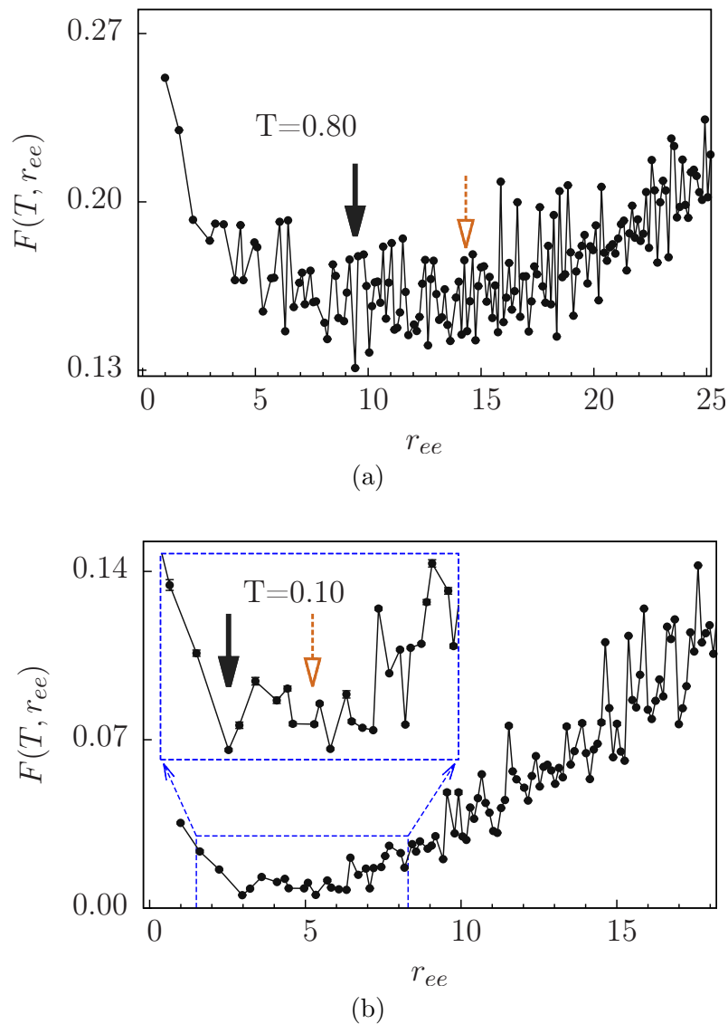
Figure 5. Normalized free energy vs end-to-end distance at (a) T = 0.8 and (b) T = 0.1 for the HOP124 lattice protein. Black arrows indicate the lowest free energy at each temperature ( T ), orange arrows point to the mean end-to-end distance at that temperature. Error bars are smaller than the data points.
