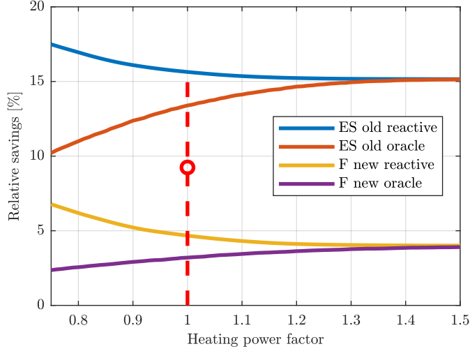
Figure 11: The relative savings for two types of artificial households (typical schedules for employed singles (ES) and family (F), either in a “new” or “old” dwelling) depending on the design heat load (scaled default value). The vertical dashed line corresponds to the default design heat load, at which we carried out the main evaluation. The red circle marks the average (9.24% according to Table 4) of all households in the CER dataset using the oracle strategy.
