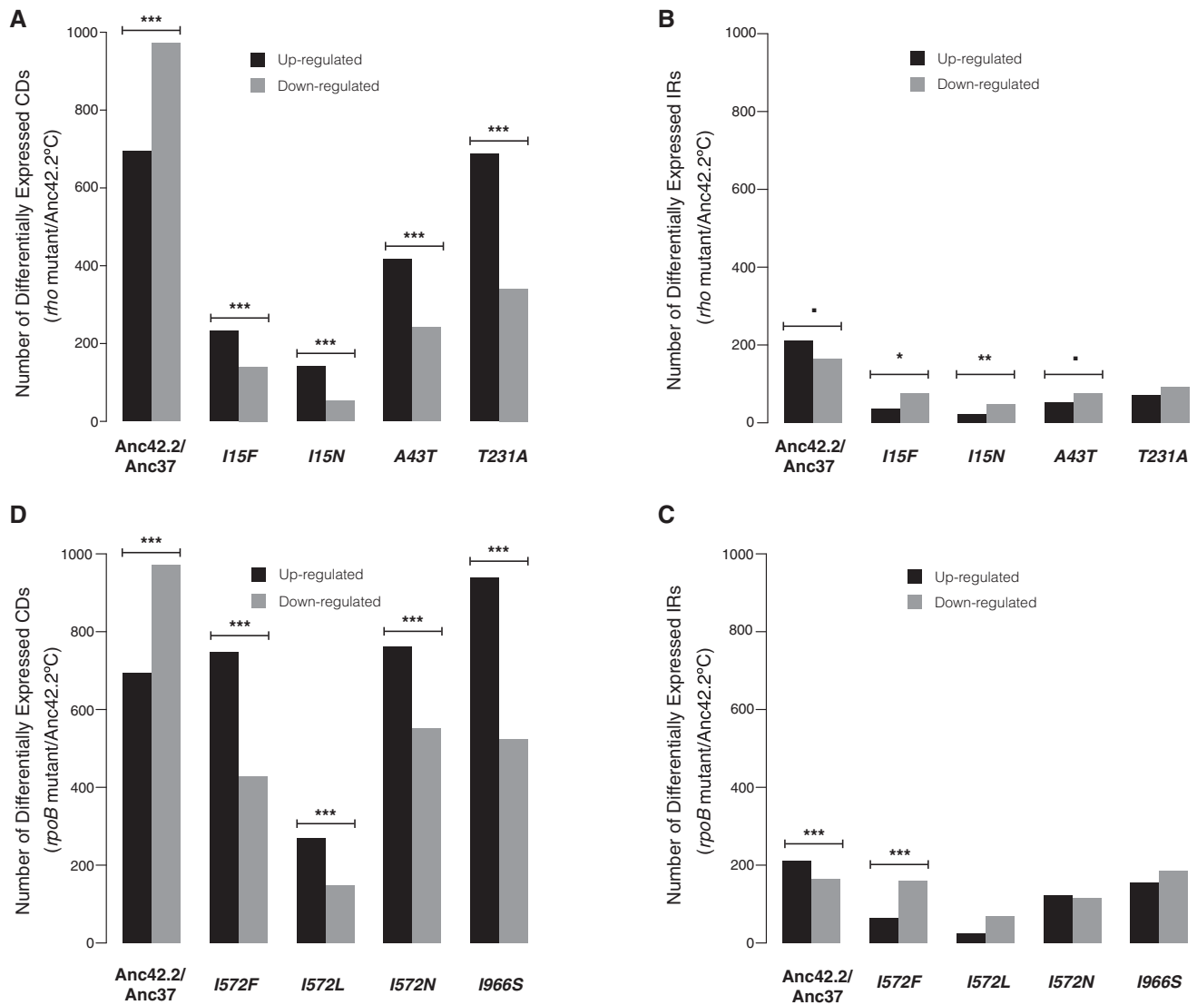
Fig. 5. Genome-wide expression patterns of genic and intergenic regions at 42.2 °C. Histograms showing the number of coding regions that are up or down regulated compared with REL1206. (A) The first pair of histograms shows REL1206 at 37.0 °C versus 42.2 °C. Up- or down-regulation is relative to the first of the listed pair. For example, the first pair of histograms show that REL1206 at 42.2 °C has ~700 and ~1,000 genes that are expressed at higher and lower levels, respectively, than REL1206 at 37.0 °C. The remaining histograms compare rho mutants at 42.2 °C to REL1206 at 42.2 °C. The bars with three, two and one asterisks indicate P < 0.0001 , P < 0.001 and P < 0.01 , respectively, a dot indicates P < 0.05 . (B) Similar histograms as in A, but based on intergenic regions (IRs). (C) and (D) are identical to (A) and (B) but based on the rpoB mutants.
