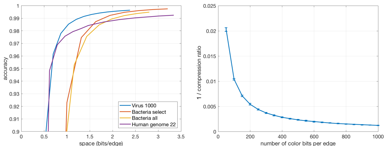
(a) Accuracy as a function of Bloom filter size in terms of bits per edge across all datasets. (b) Compression ratio at 99% accuracy as a function of color bits per edge in Virus1000 .
