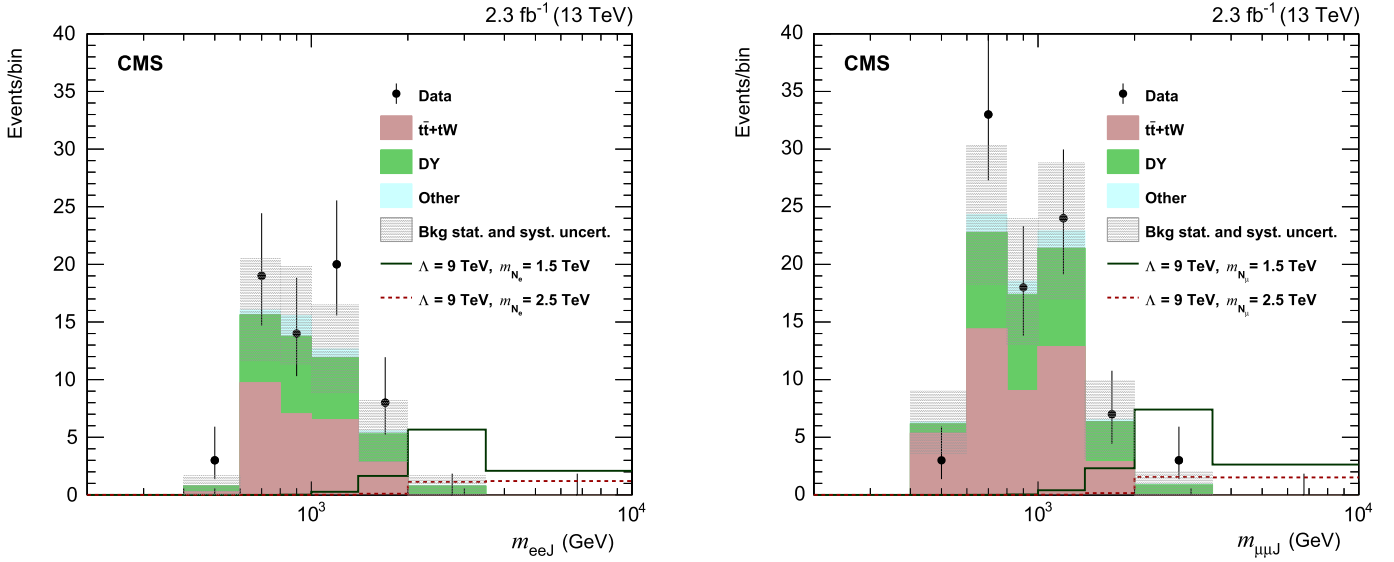
Fig. 4. Distribution of the variable m_{\ell\bar{\ell}q} for the data (black points), the estimated SM backgrounds (stacked filled histograms), and the signal (lines) with \Lambda = 9 TeV and masses of N_\ell equal to 1.5 and 2.5 TeV, for the ee\bar{q} (left) and the \mu\mu\bar{q} (right) channels. “Other” stands for the contribution from W+jets and diboson events. The background uncertainties are the combined statistical and systematic uncertainties. (For interpretation of the references to colour in this figure, the reader is referred to the web version of this article.)
