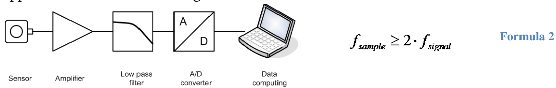
Fig. 1. Measuring chain setup
