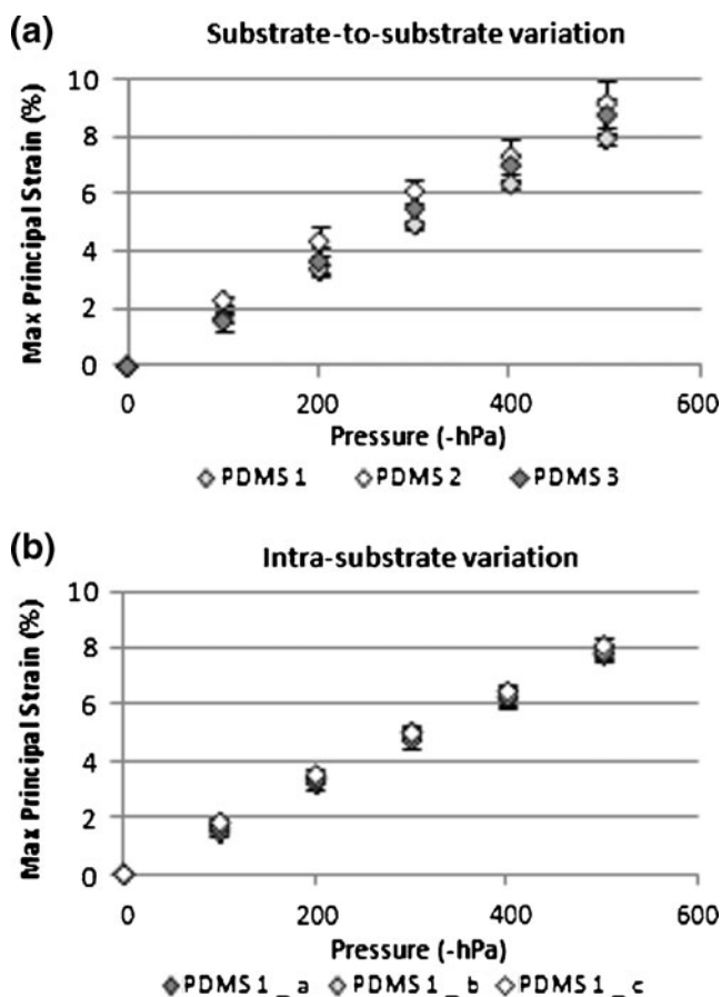
Fig. 6 PDMS surface strain calibration. (a) Substrate-to-substrate and (b) intra-substrate variations are shown
