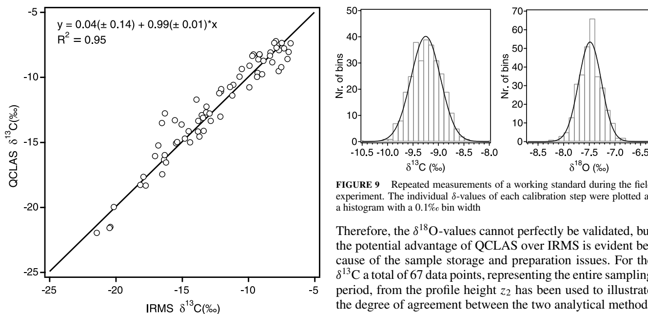
FIGURE 8 Comparison of ^{13}\text{C} -values measured with QCLAS and IRMS. Flask samples for the IRMS were collected every 2 h during the experimental period (August 15–23, 2007). The linear regression indicates an excellent agreement between the two techniques
