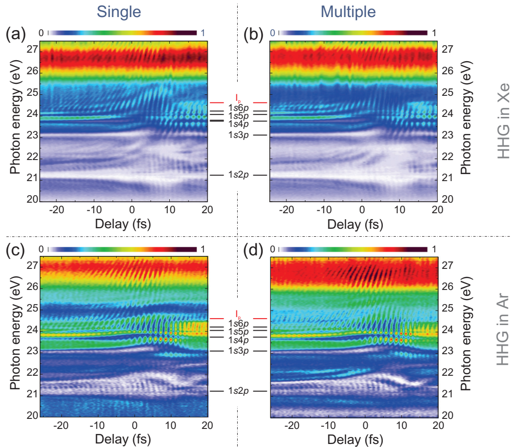
Figure 8. Delay-dependent transmitted XUV spectra for a CEP value \varphi_0 leading to the generation of a SAP (a, c) and for CEP = \varphi_0 + \pi/2 (b, d). Panels (a) and (b) are obtained with the XUV light generated in xenon while in (c, d) attosecond pulses generated in argon were employed. The lines mark the energy position of single-photon accessible atomic states of helium. Fast modulation of the transmitted signal is evident both for single and multiple attosecond pulse excitation independent of the generation medium.
