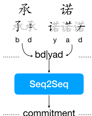
Figure 1: Overview of the wubi2en approach to Chinese-to-English translation. A raw Chinese word (‘承诺’) is encoded into ASCII characters (‘bd|yad’), using the Wubi encoding method, before passing it to a Seq2Seq network. The network generates the English translation ‘commitment’, processing one ASCII character at a time.
