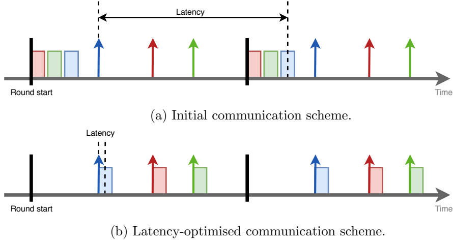
Figure 3.3: Illustration of the offset compensation. (a) shows the large latency for a possible initial situation. The black bars denote the start of a round. The arrows represent data generation and the blocks are used for the Baloo rounds. Blocks and arrows of the same colour are used for communication and data generation of the same source. (b) shows an optimal schedule with minimal latency.
