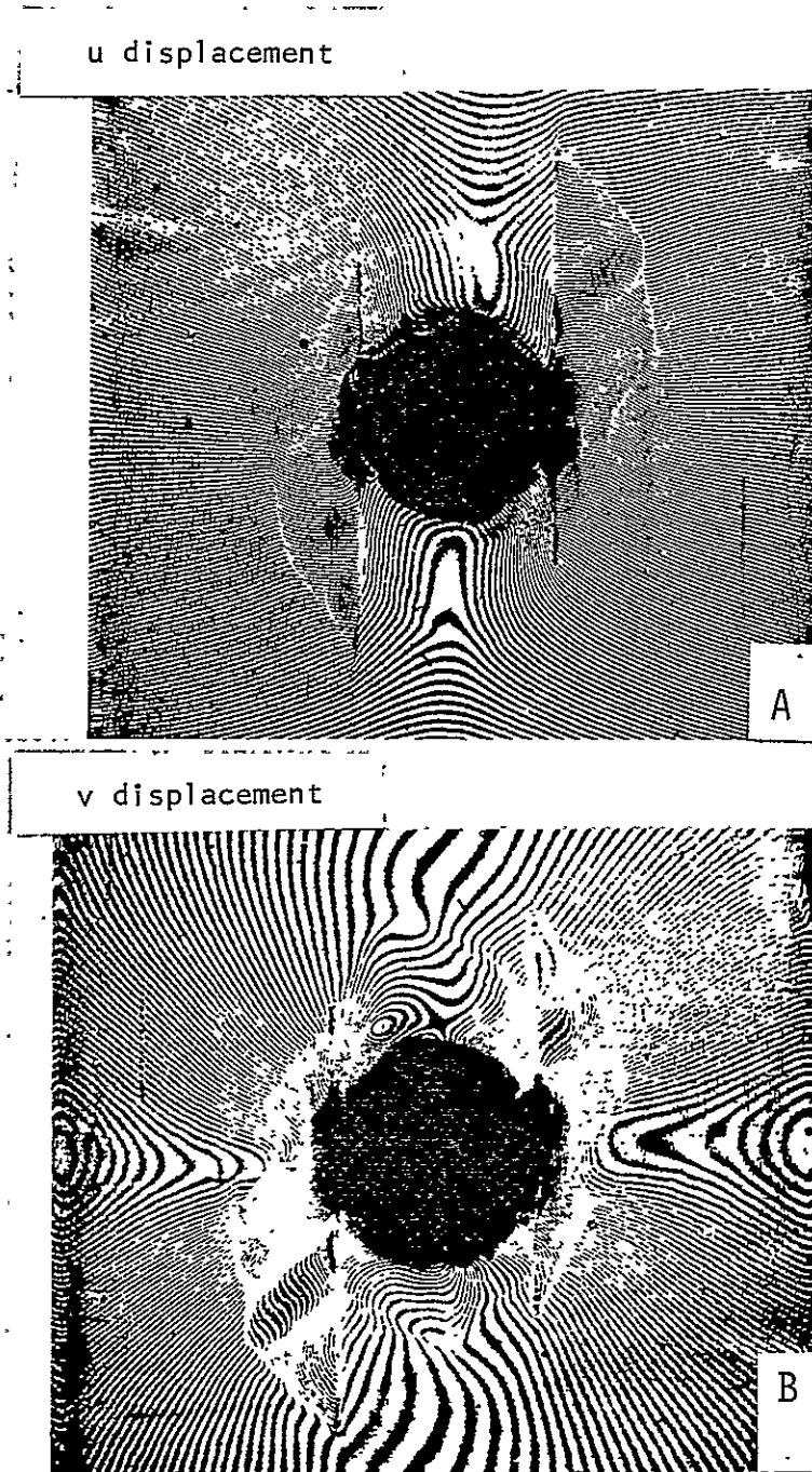
Figure 18: Fringe Pattern of the Highly Damaged A-Laminate
